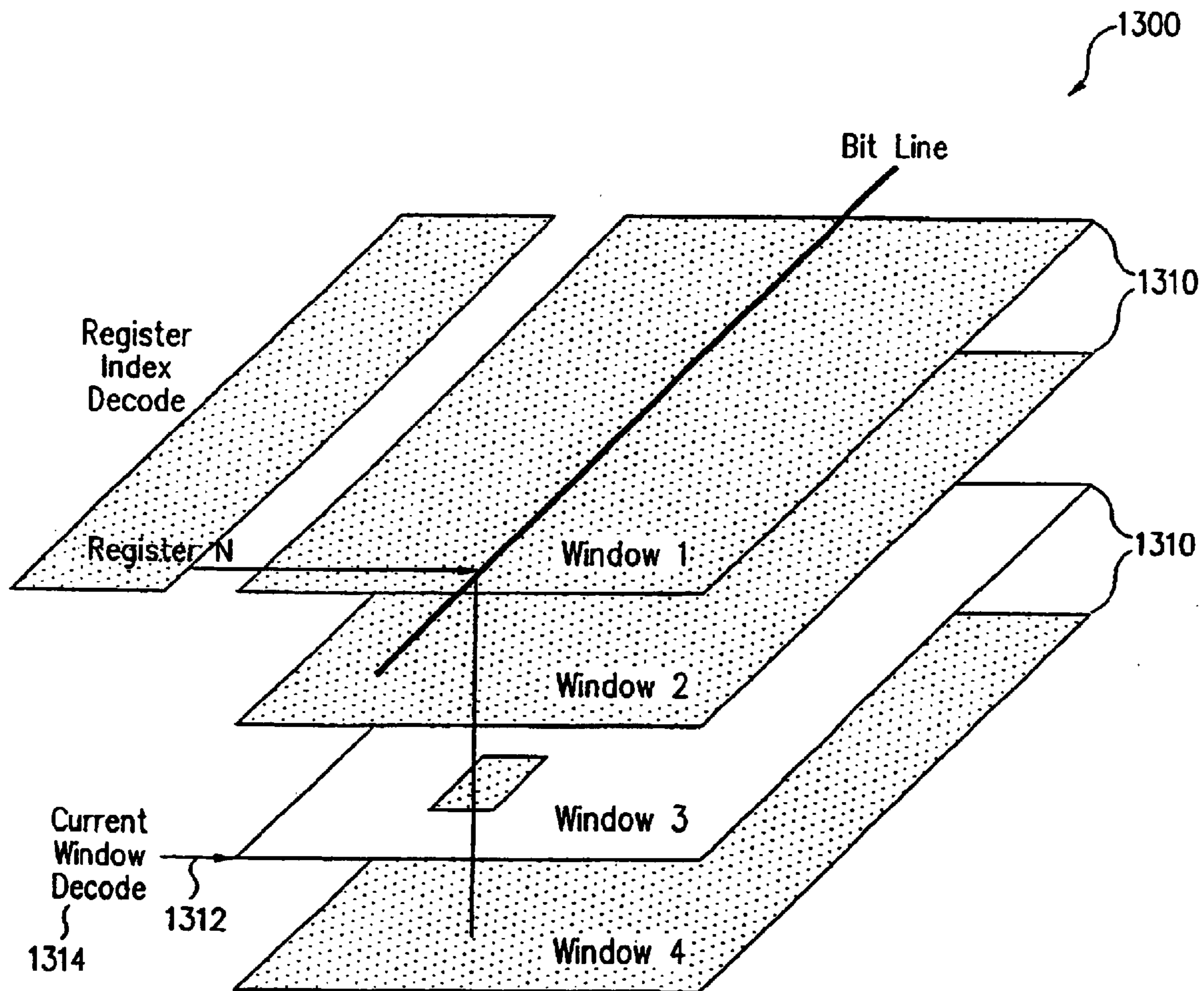
A Three Dimensional Register File
