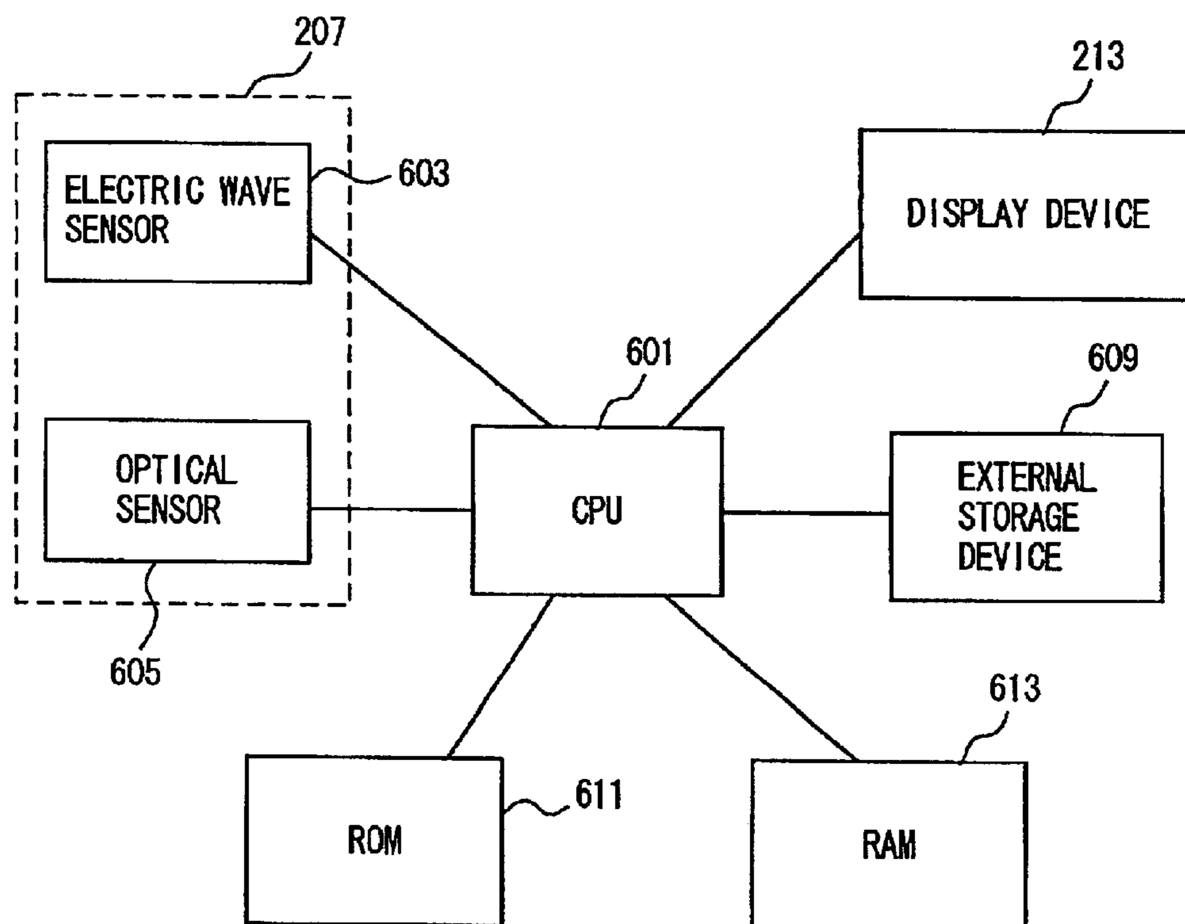
SYSTEM OUTLINE
