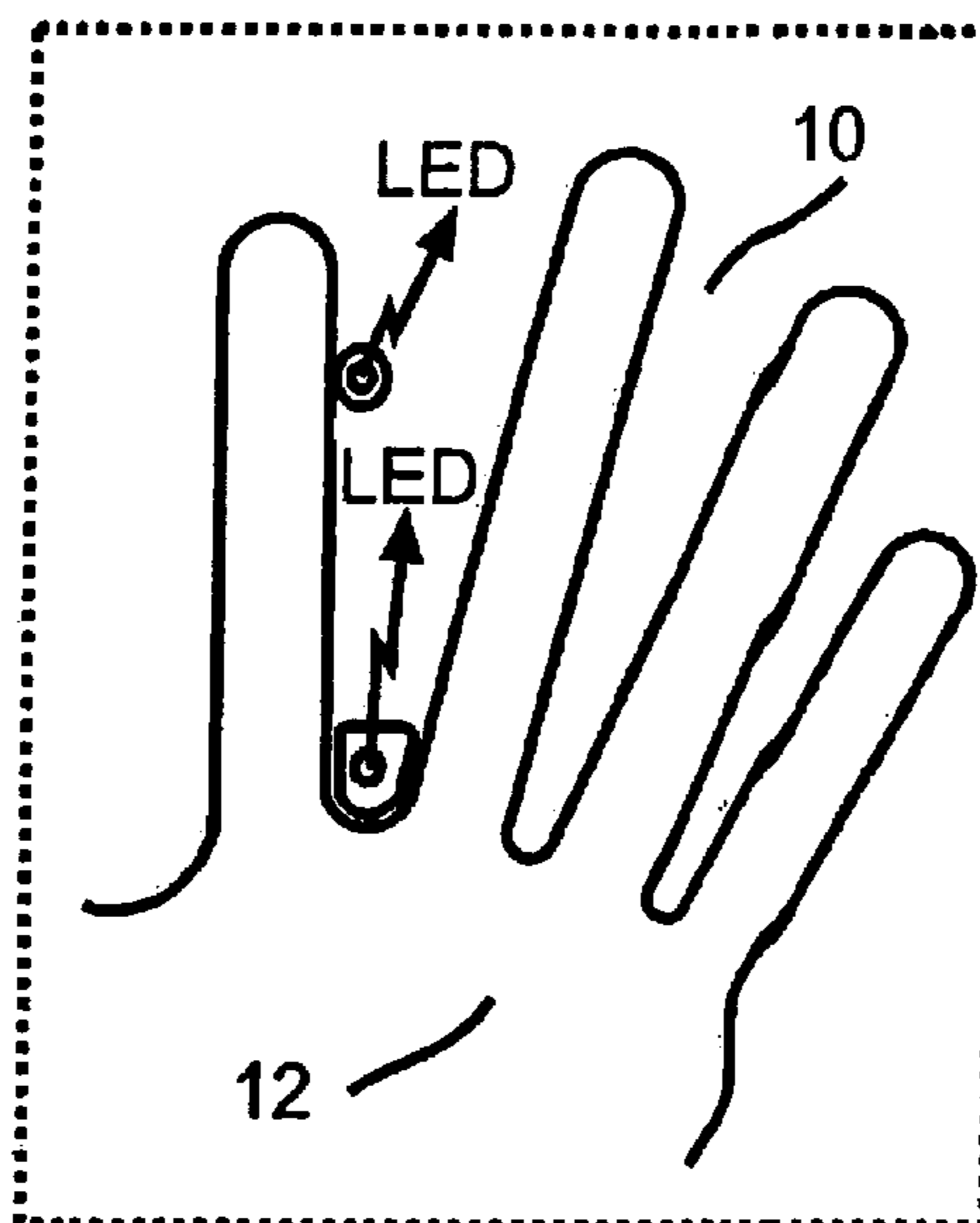
USER FINGER POSITION FEEDBACK DISPLAY
