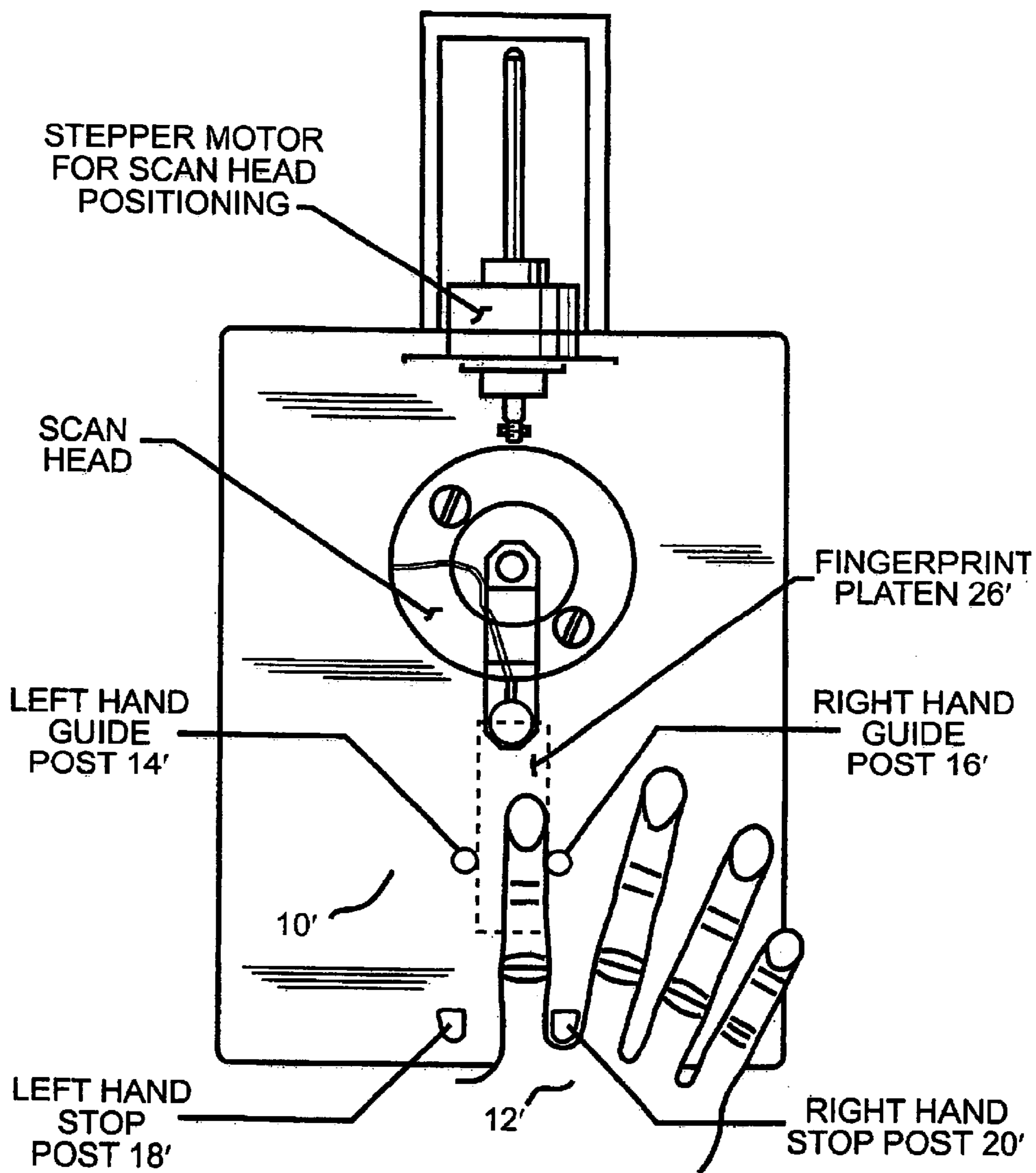
FINGER GUIDE FOR USE WITH MOVABLE SCAN HEAD SCANNER (TOP VIEW)
