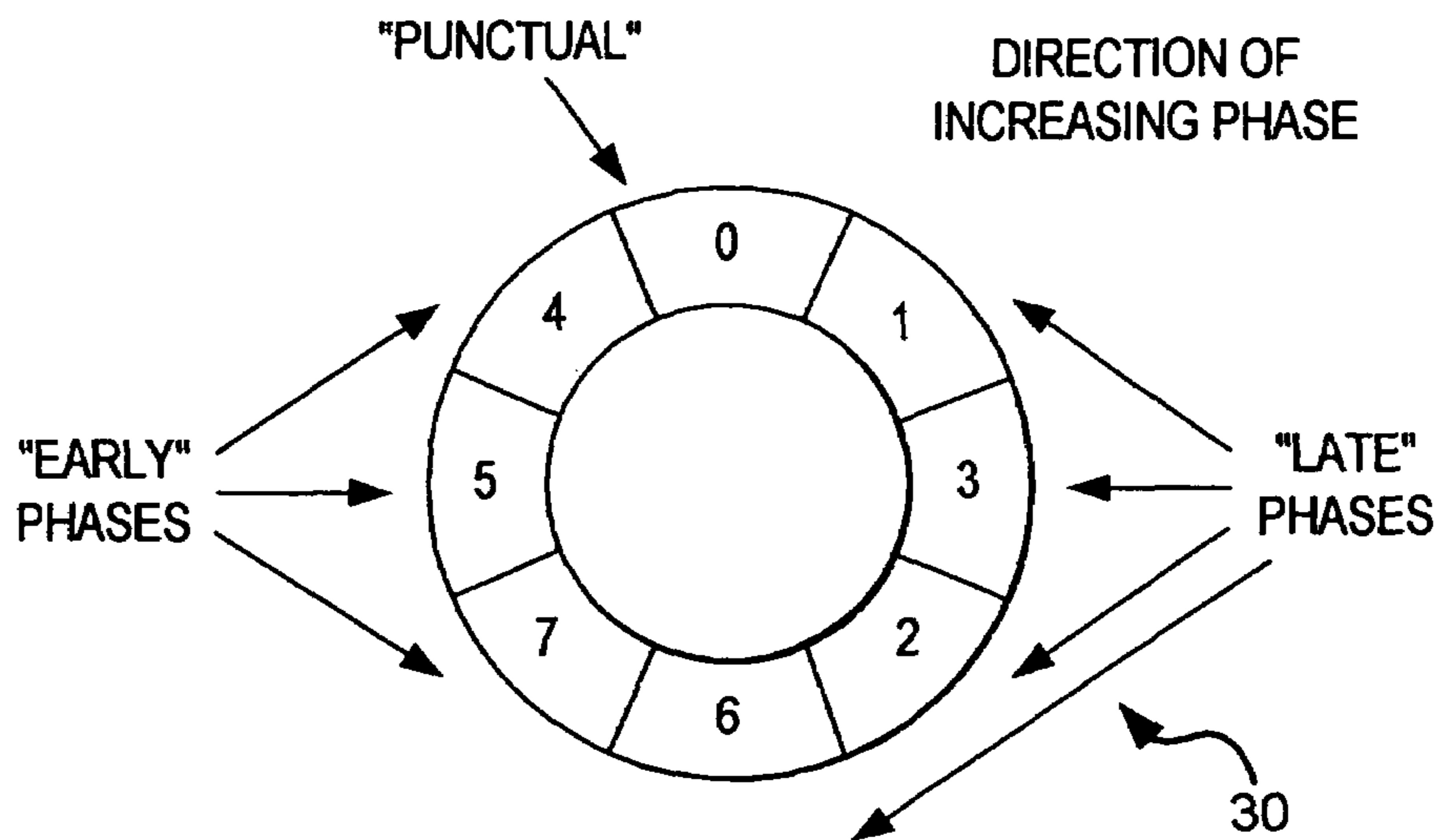
FIG. 4 NONLINEAR PHASE COUNTER.
