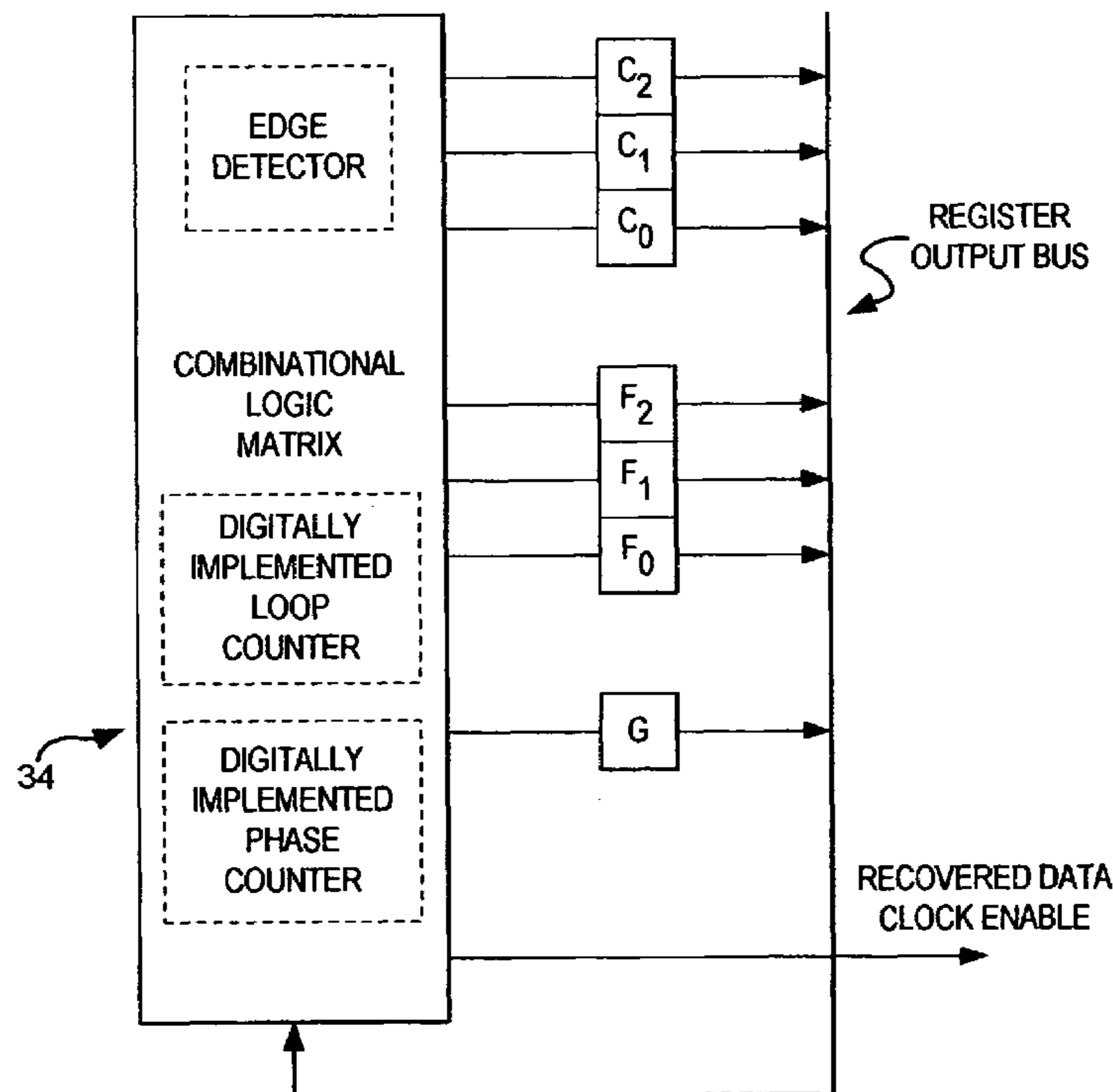
LOGIC CIRCUIT IMPLEMENTATION OF SIMPLIFIED TIMING RECOVERY CIRCUIT.
