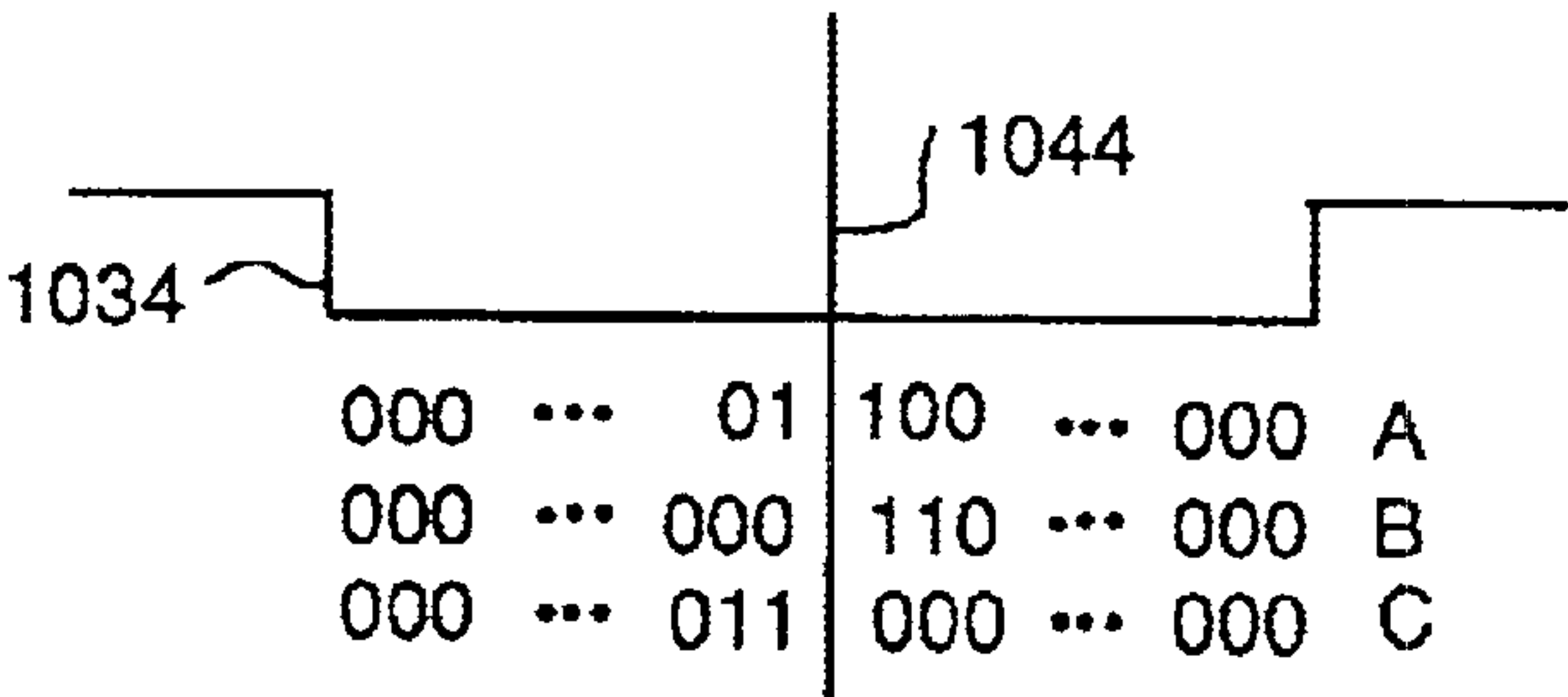
FIG. 37 FINE TUNING TO CENTER BARKER CODE
