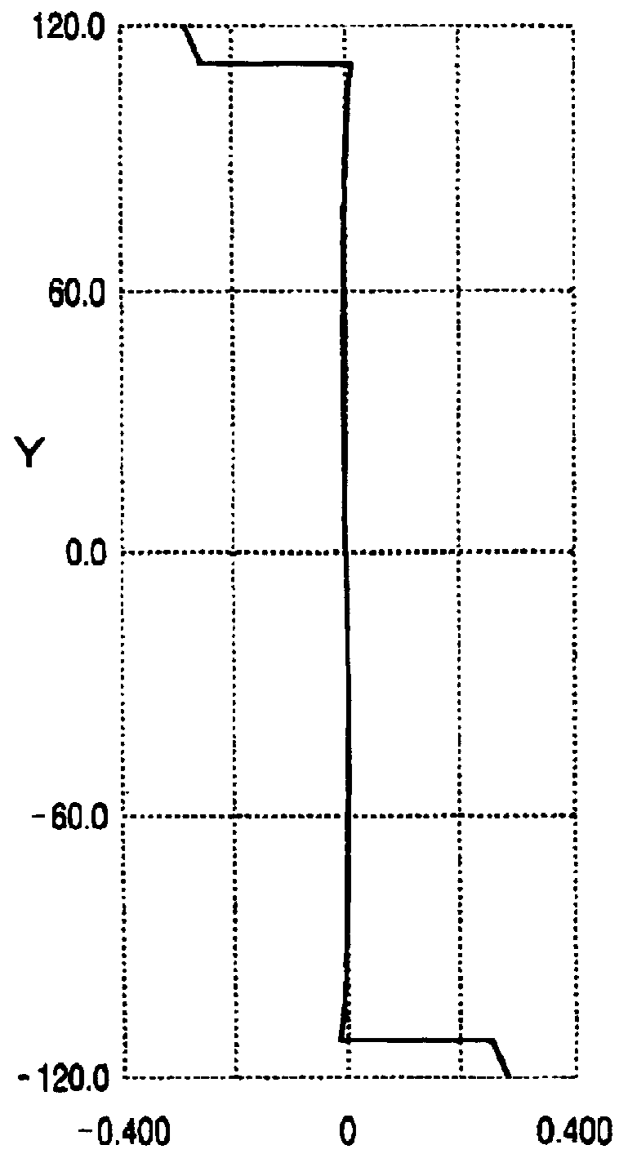
LATERAL CHROMATIC ABERRATION (WITH DIFFRACTIVE LENS)
