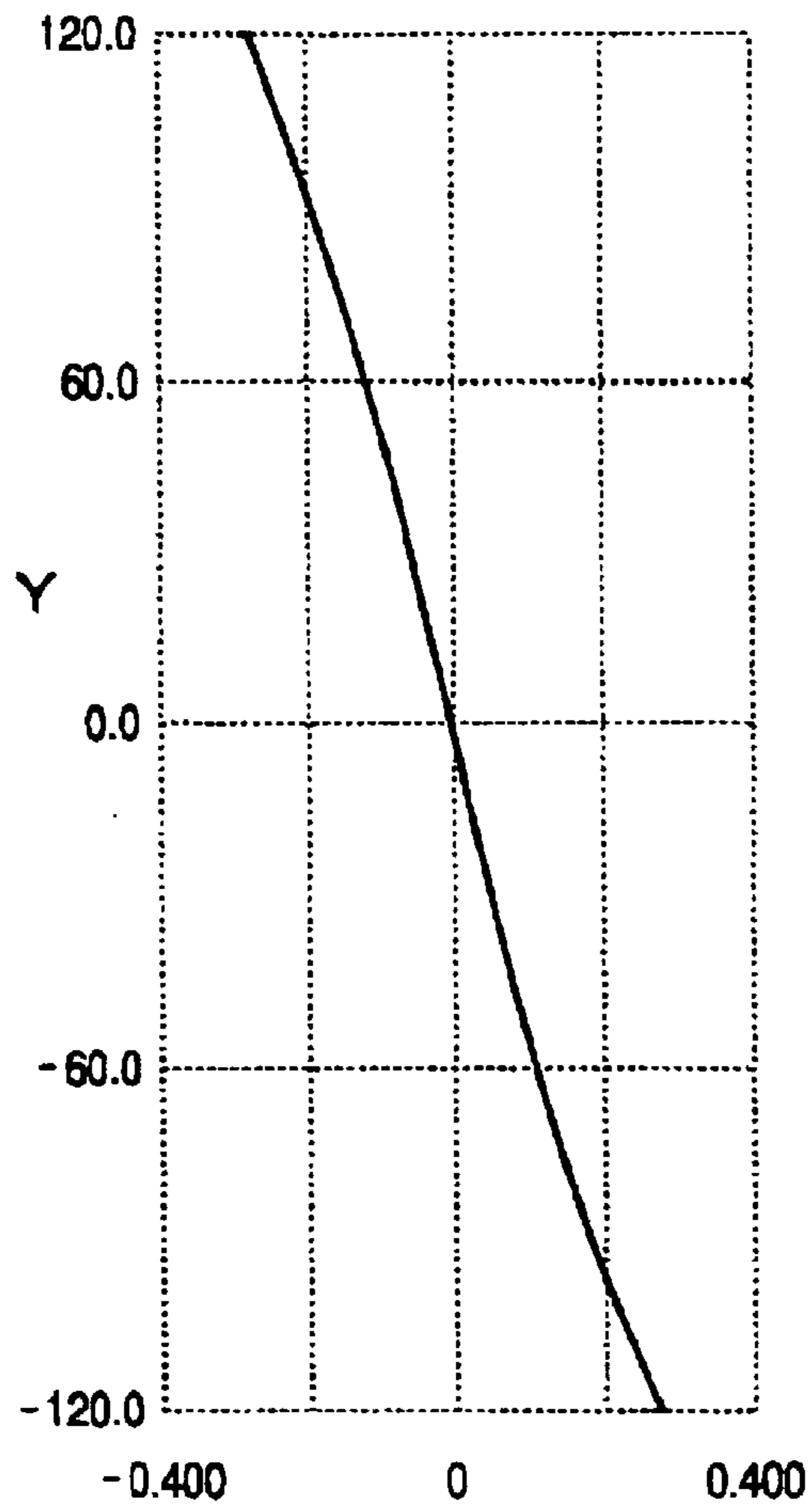
LATERAL CHROMATIC ABERRATION (WITHOUT DIFFRACTIVE LENS)
