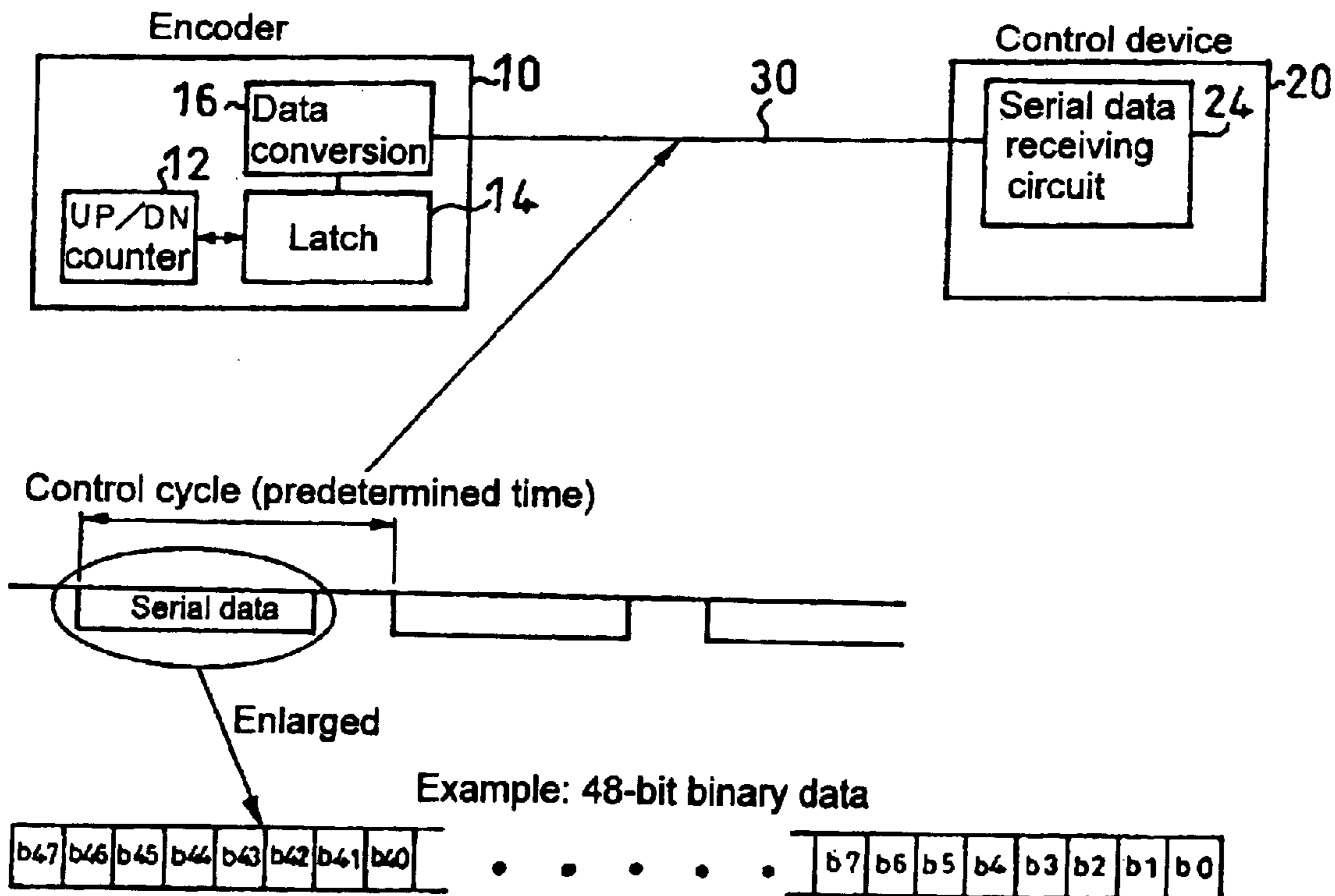
Fig. 2 PRIOR ART
