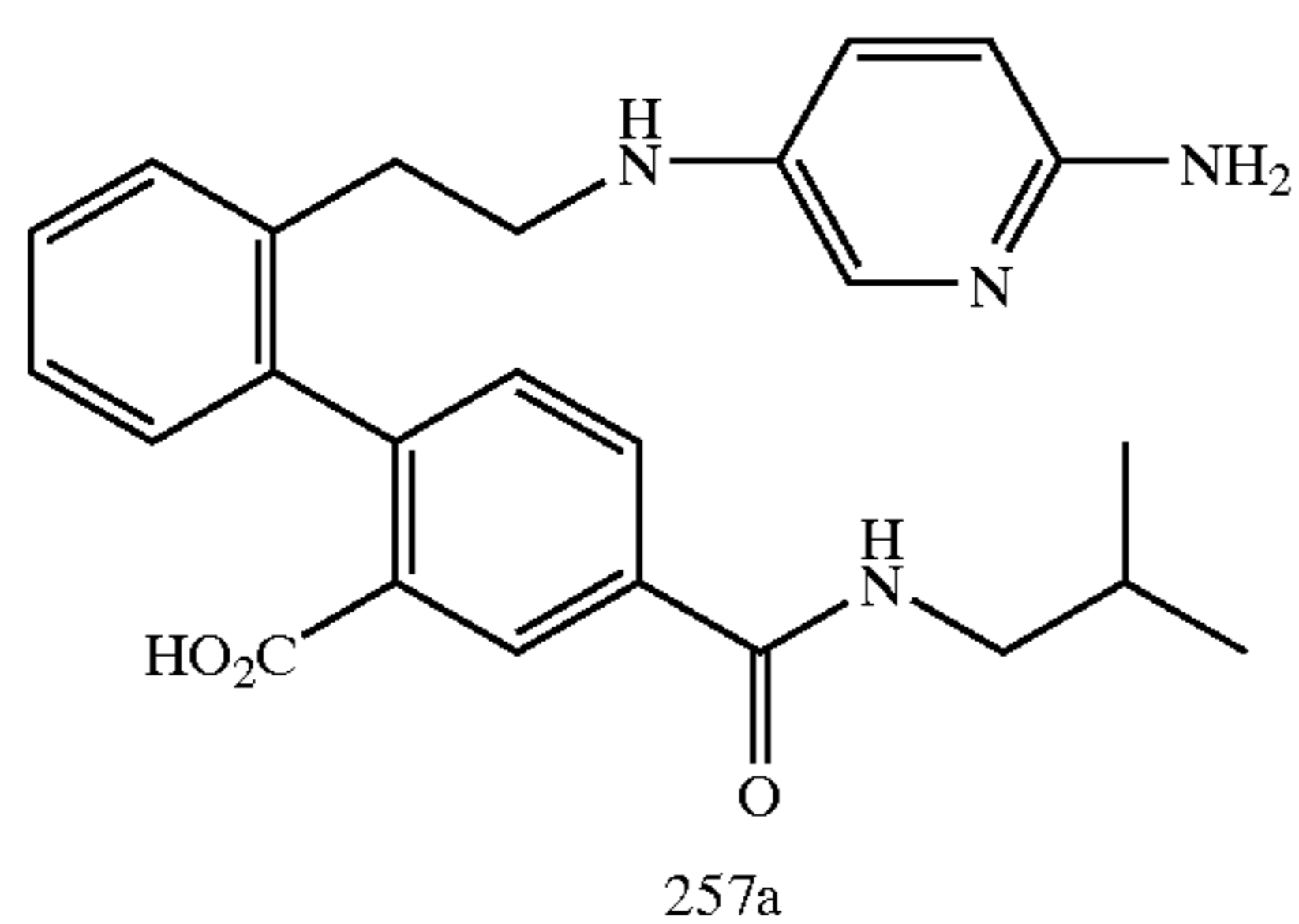
Scheme 36a
