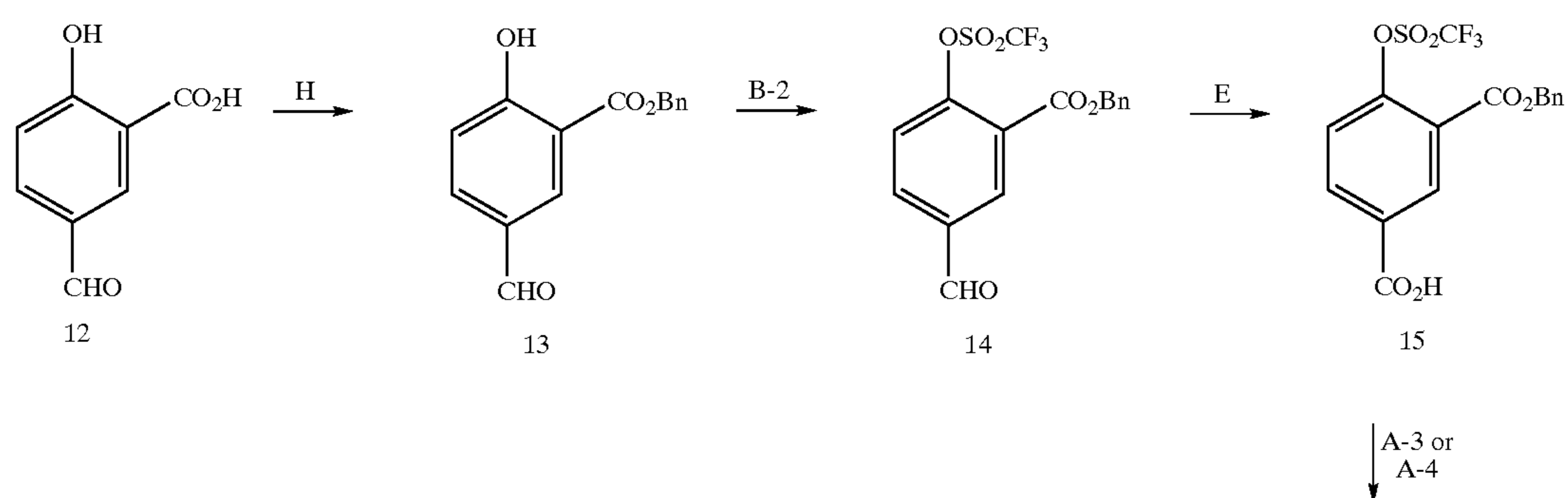
Scheme 3
