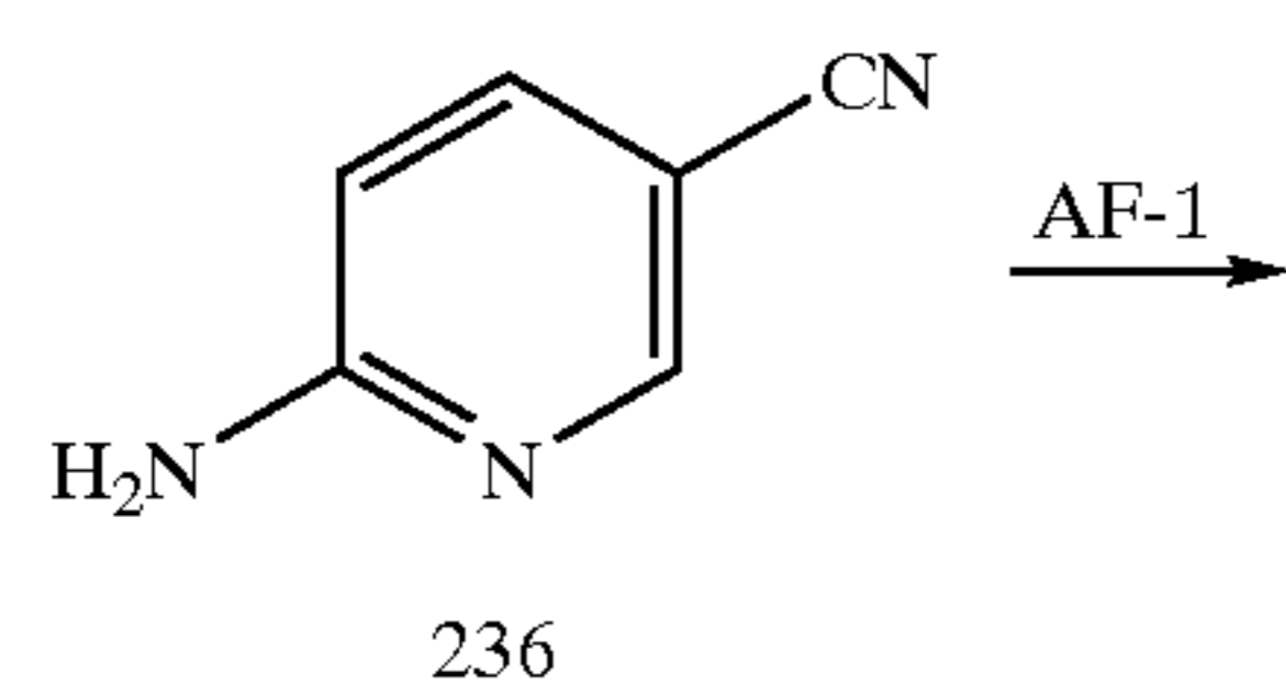
Scheme 33
