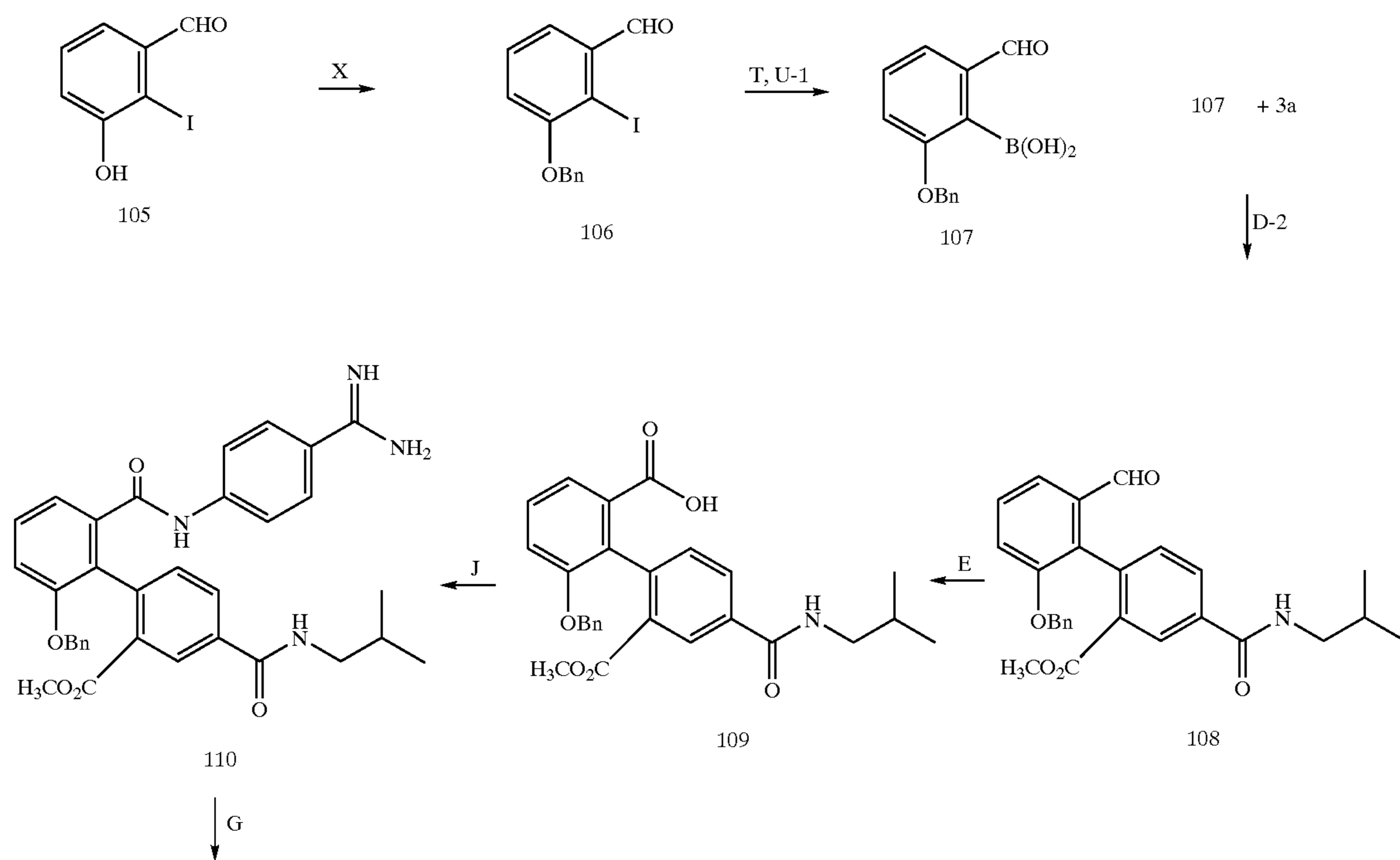
Scheme 15
