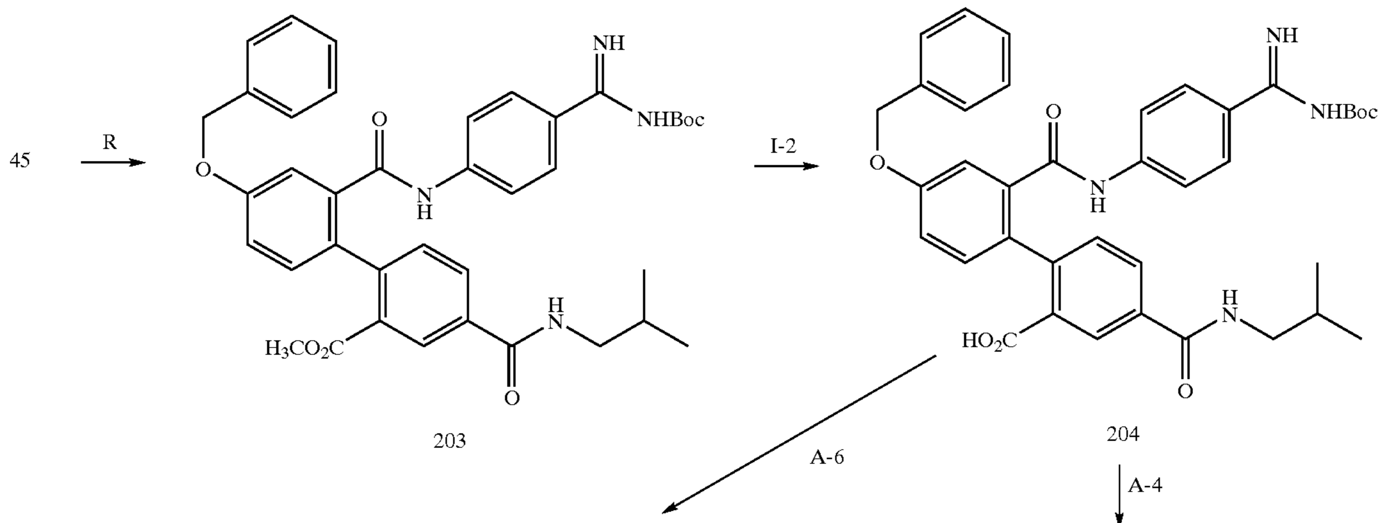
Scheme 28
