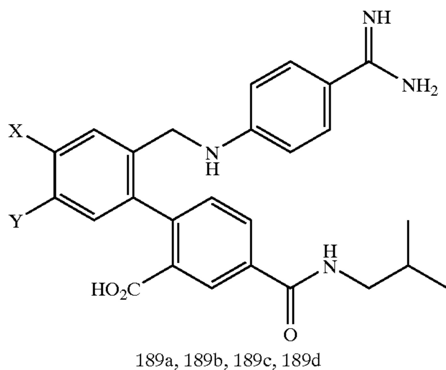
Scheme 25
