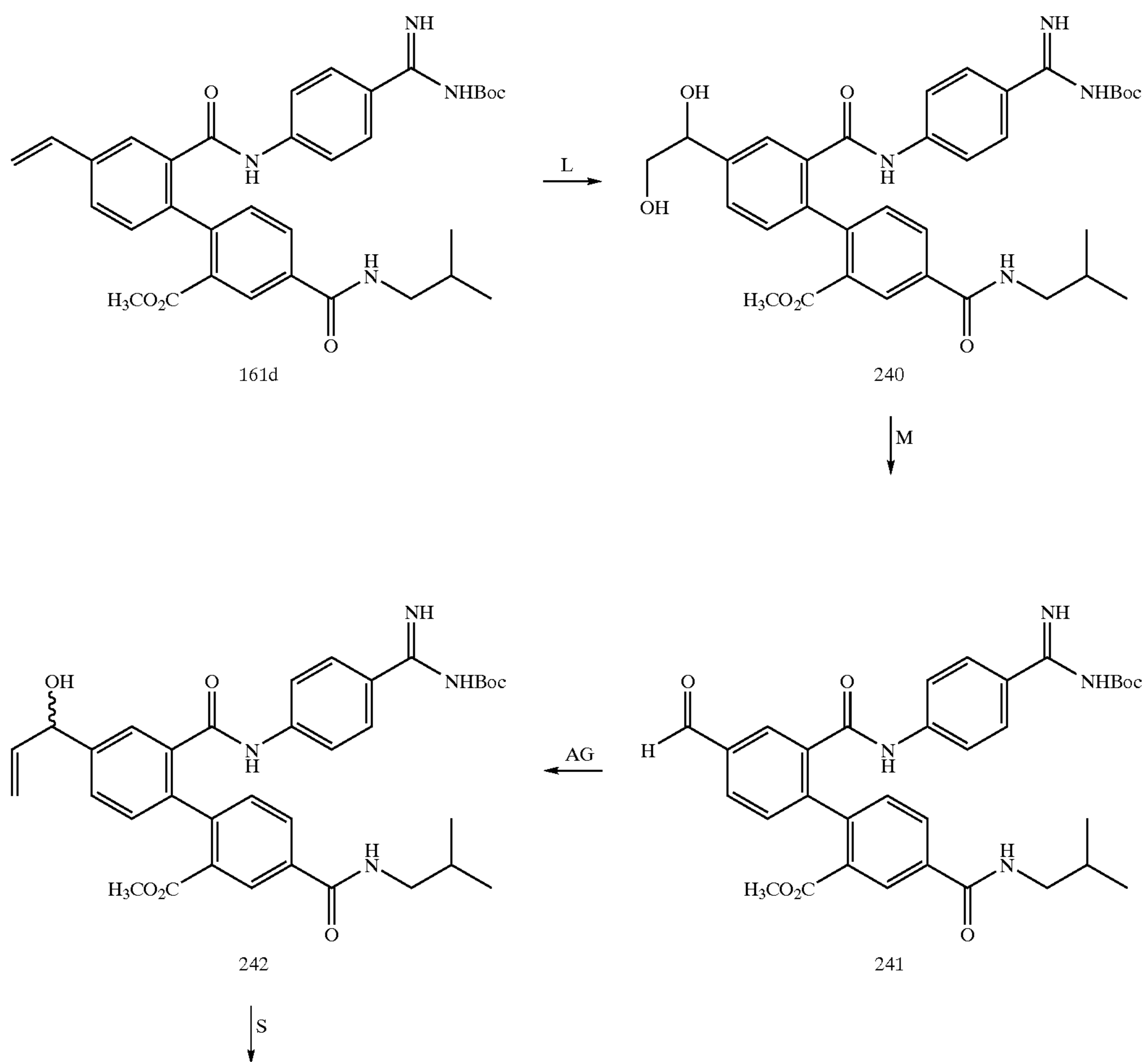
Scheme 34
