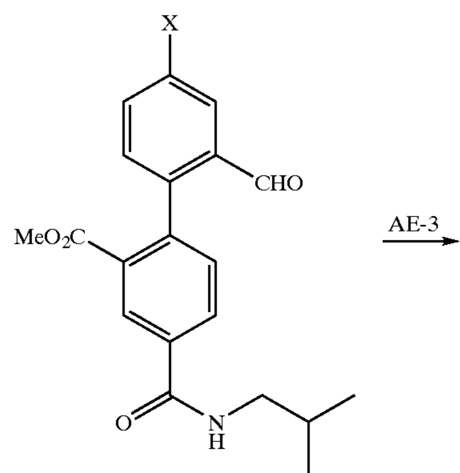
Scheme 37
