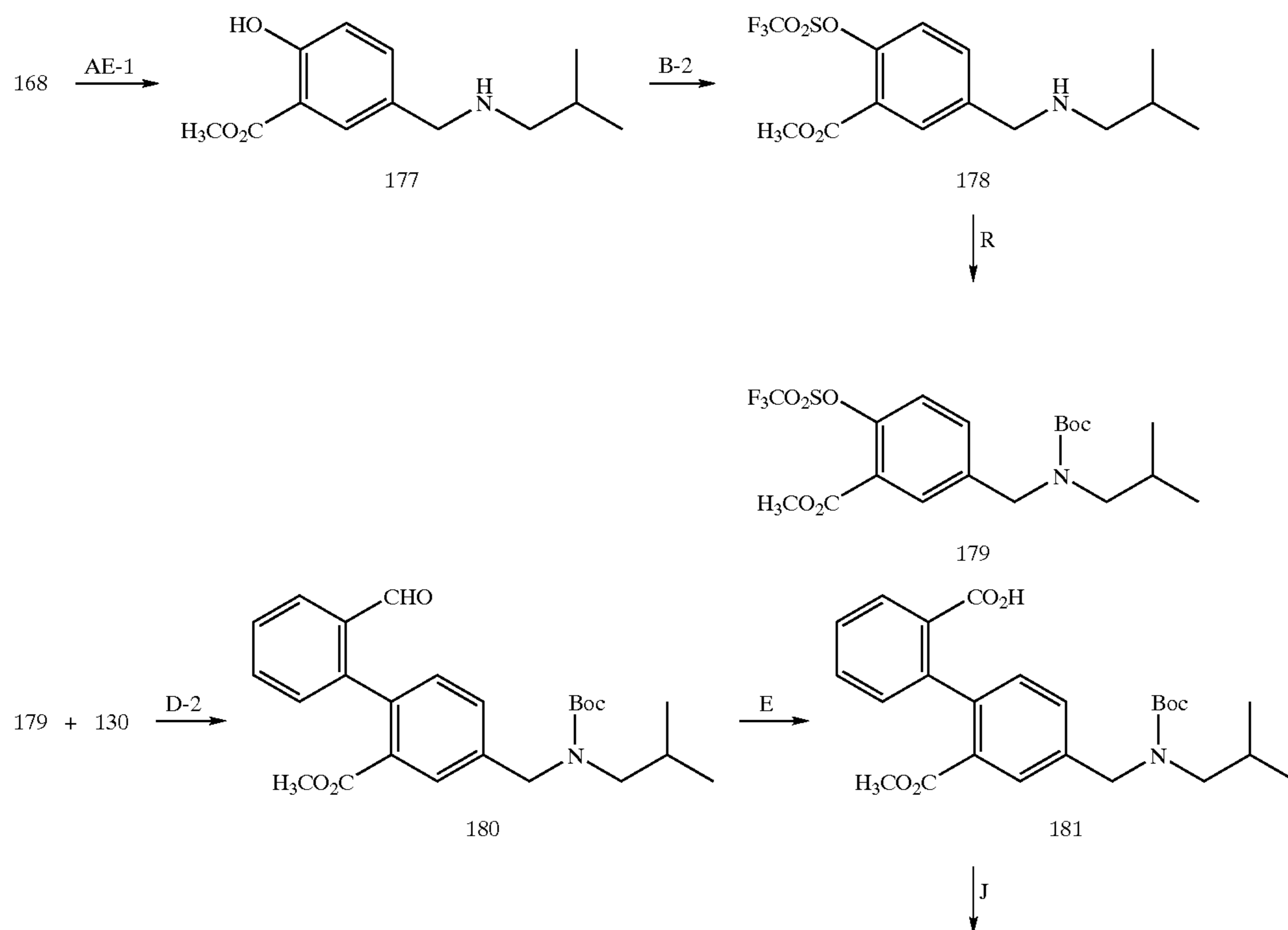
Scheme 23
