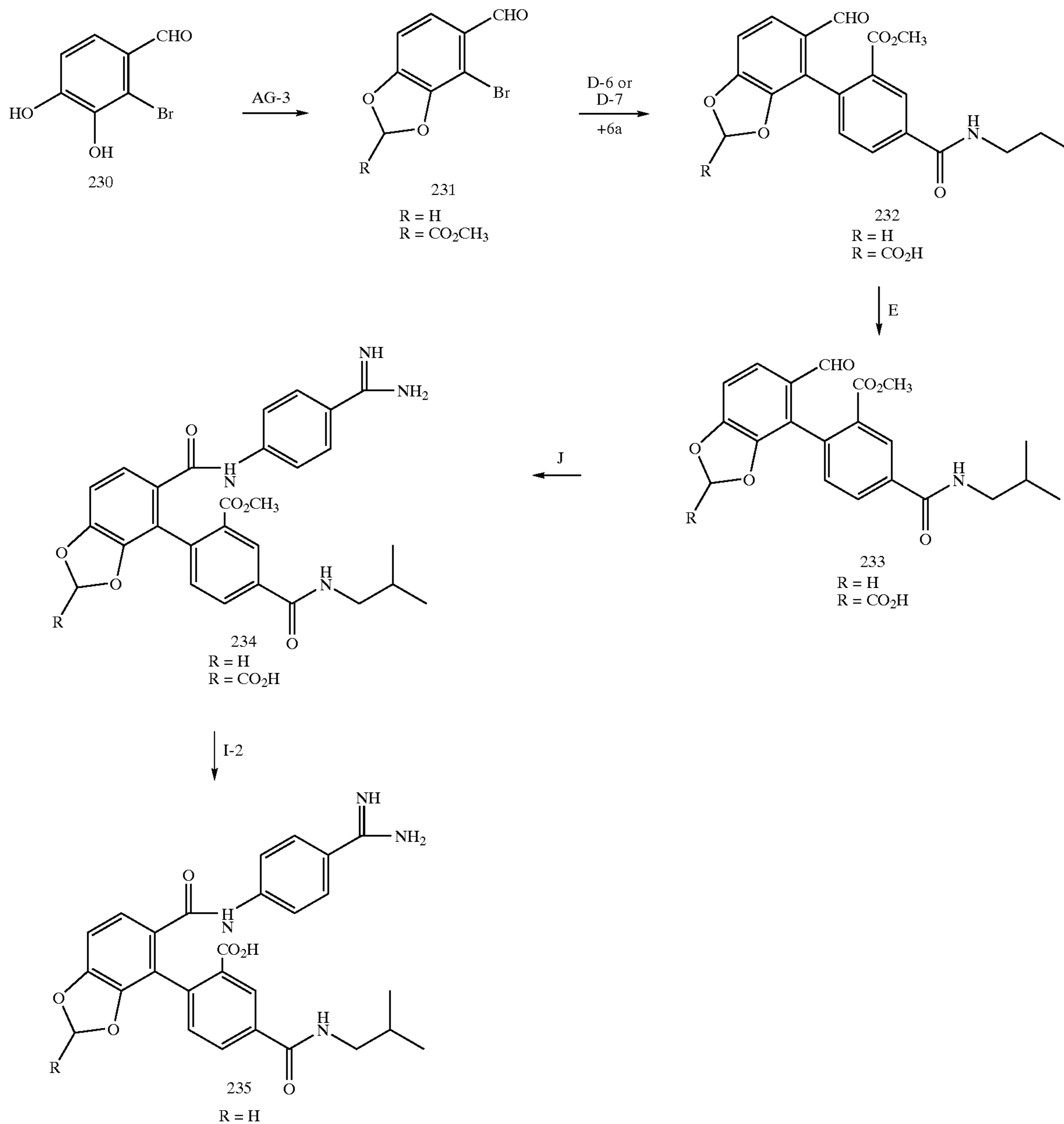
Scheme 32
