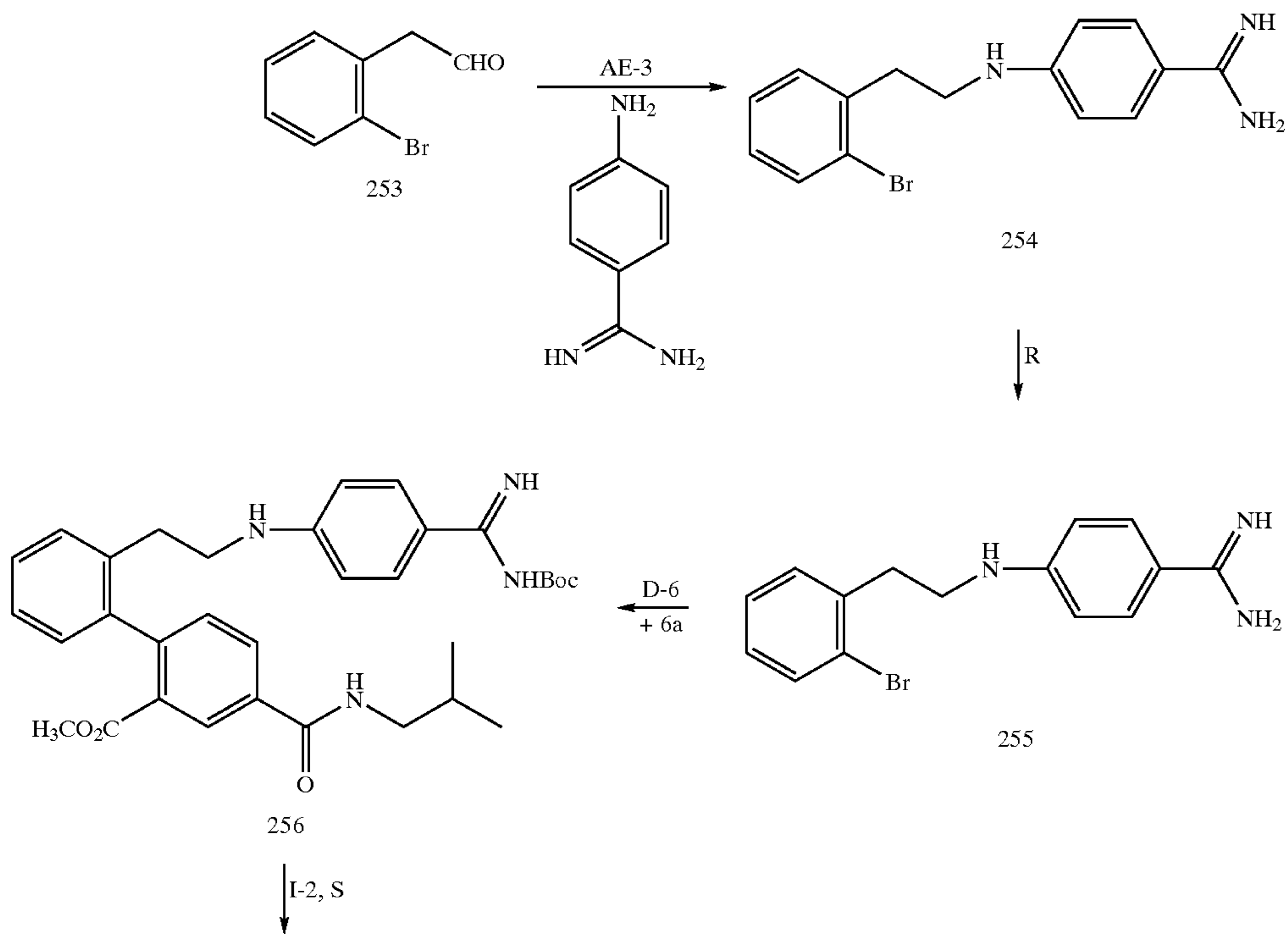
Scheme 36
