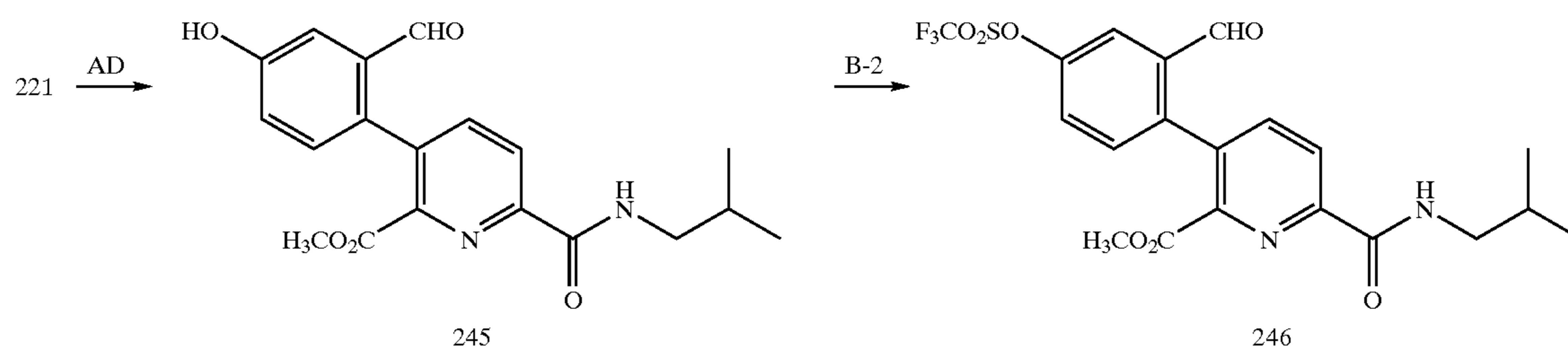
Scheme 35
