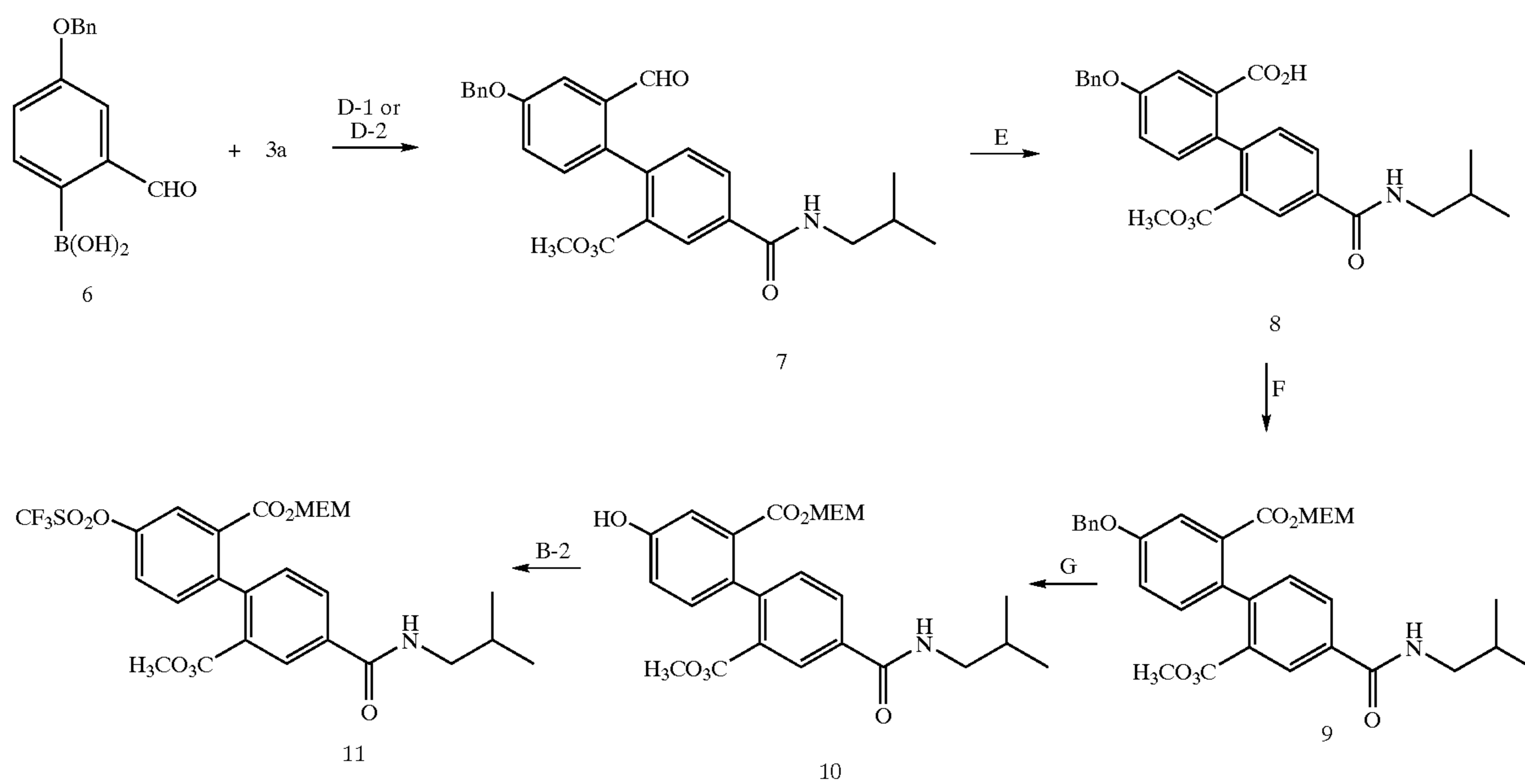
Scheme 2
