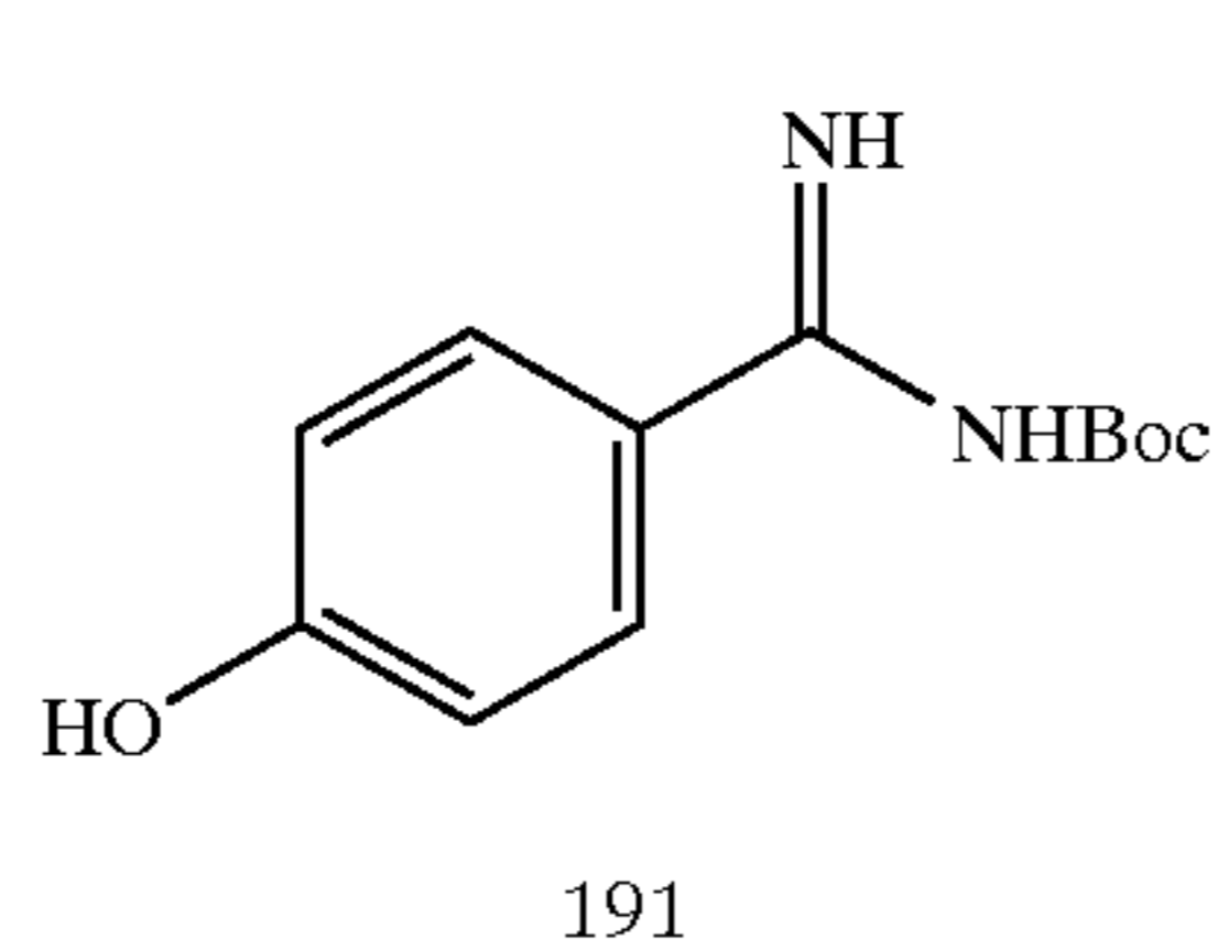
Scheme 26
