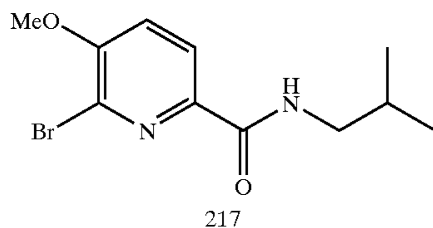
Scheme 31
