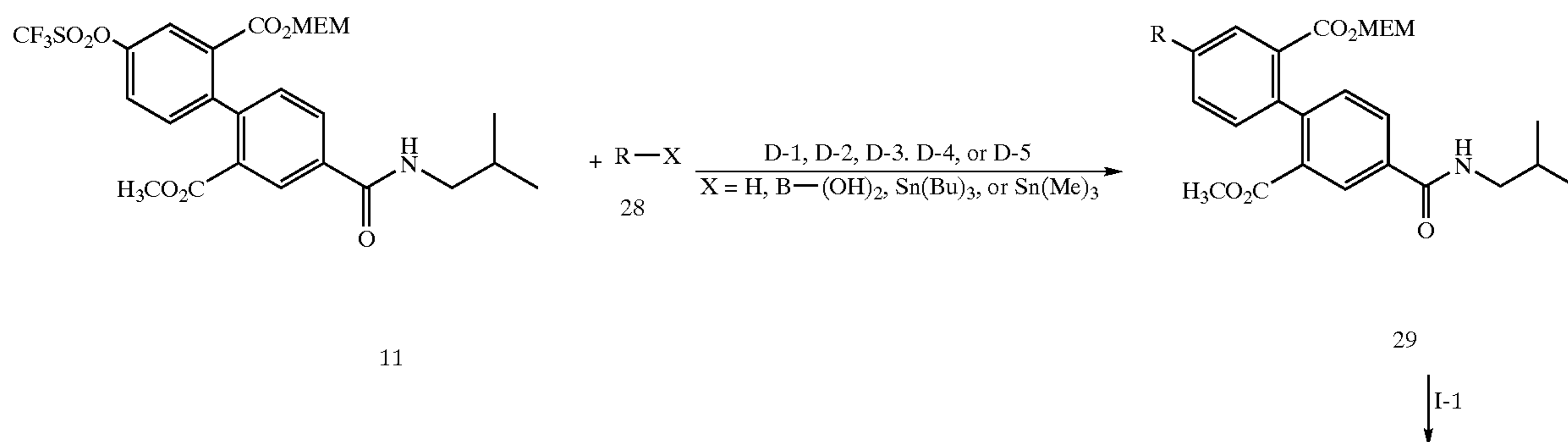
Scheme 6
