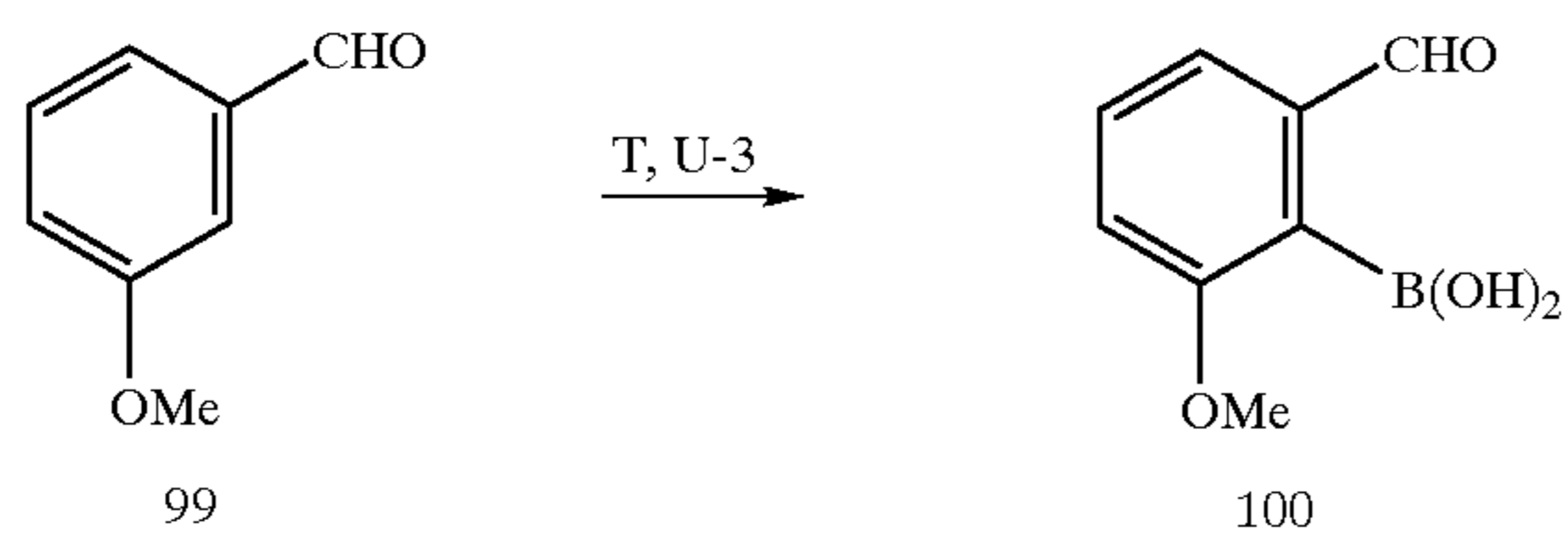
Scheme 14
