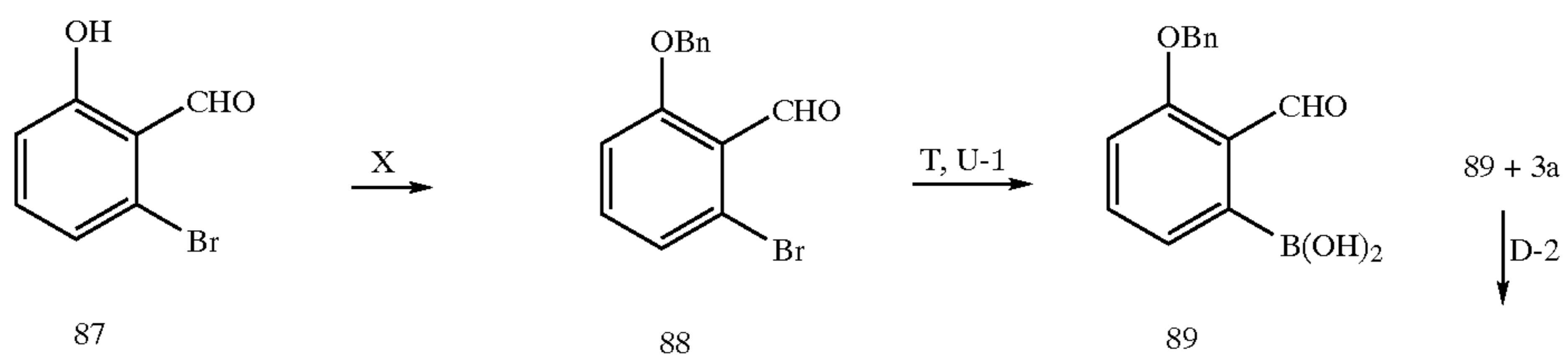
Scheme 13
