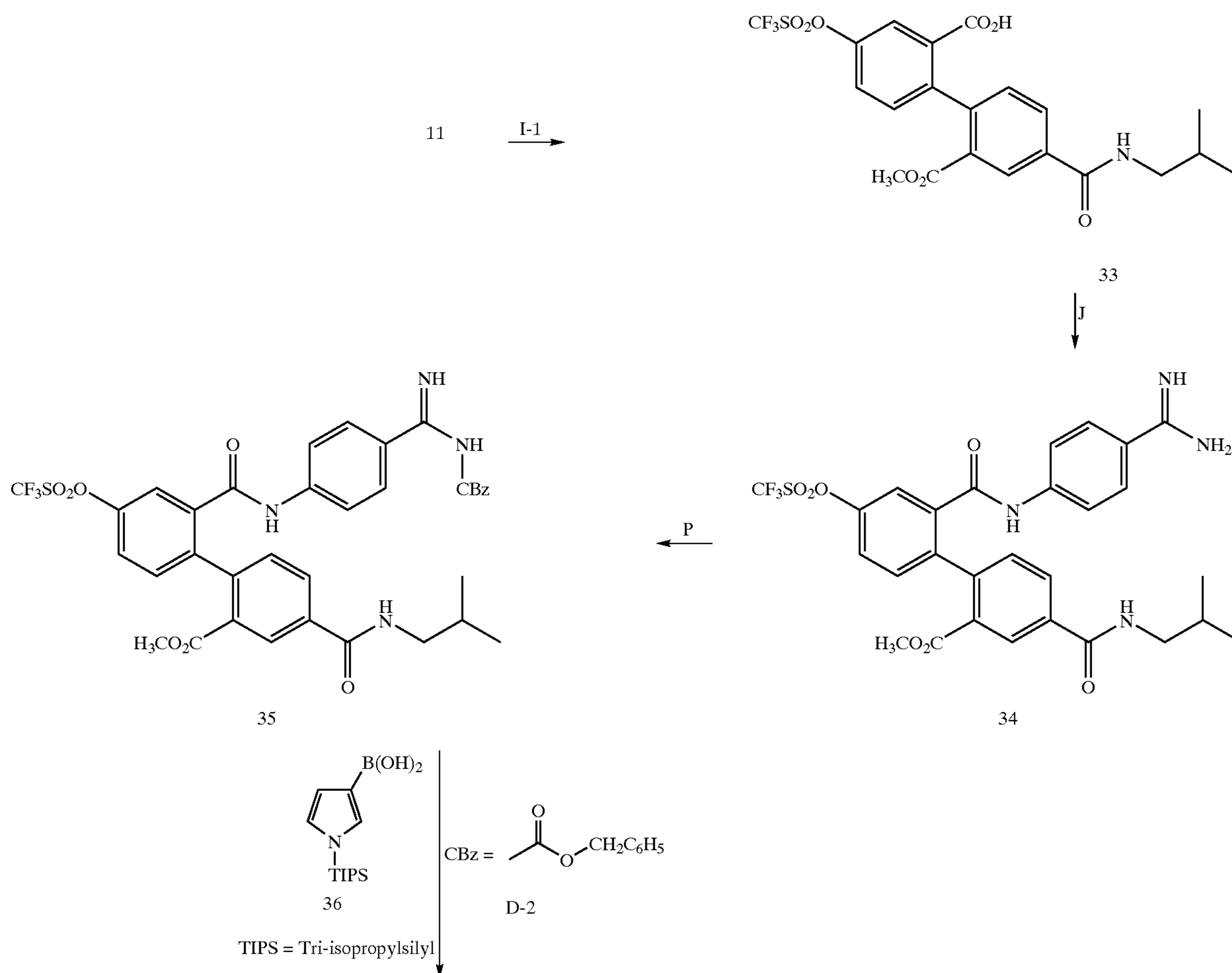
Scheme 7
