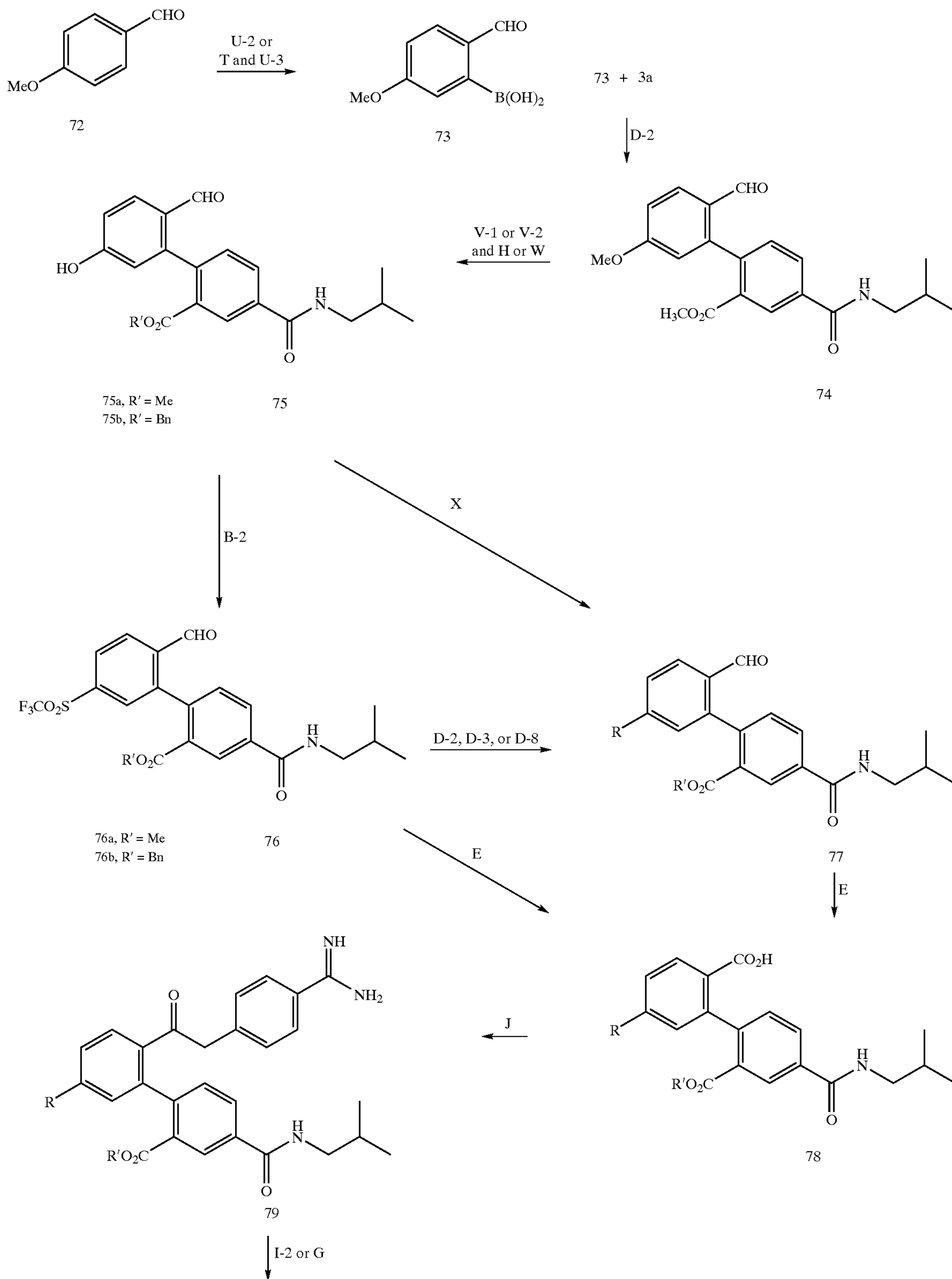
Scheme 11
