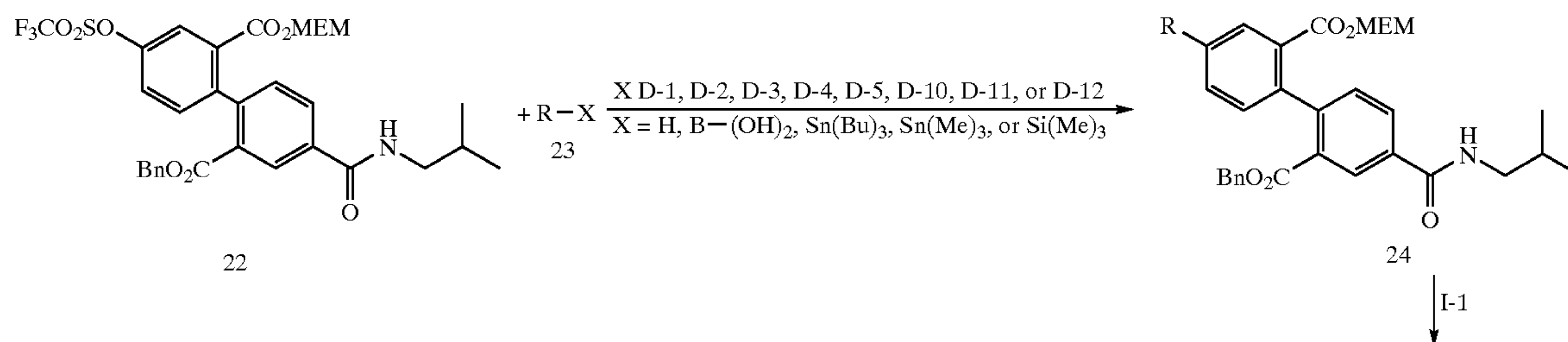
Scheme 5
