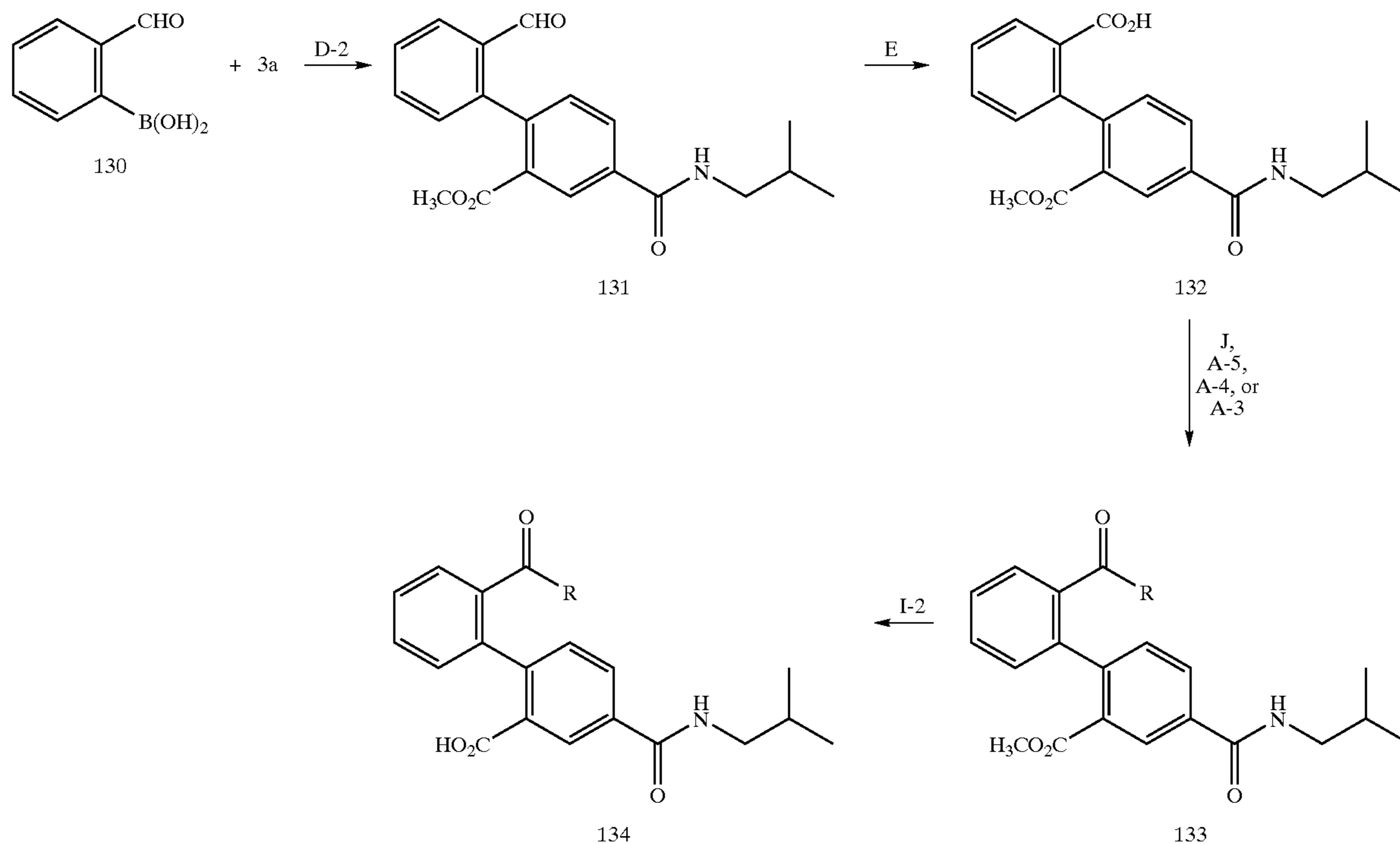
Scheme 17
