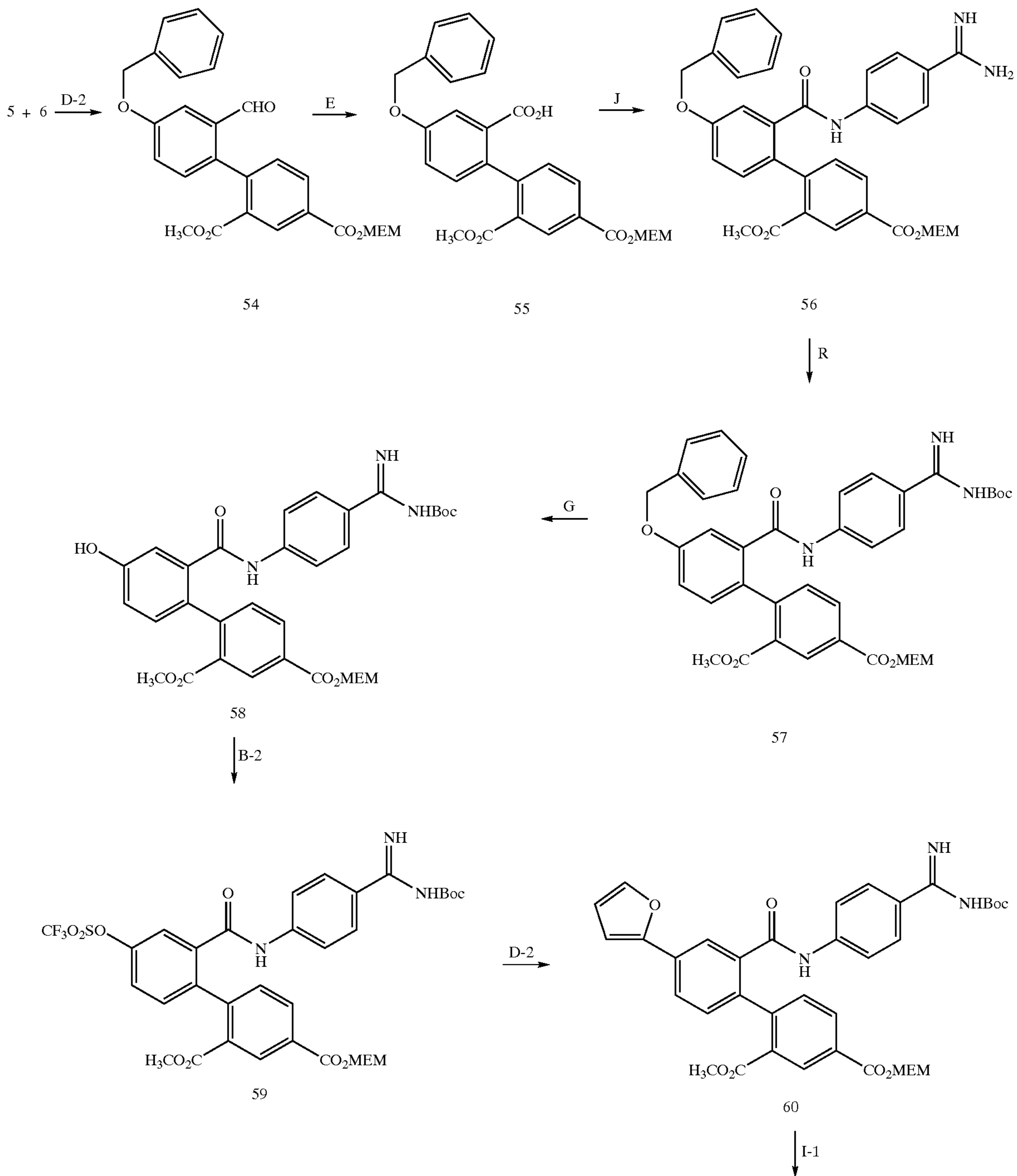
Scheme 9
