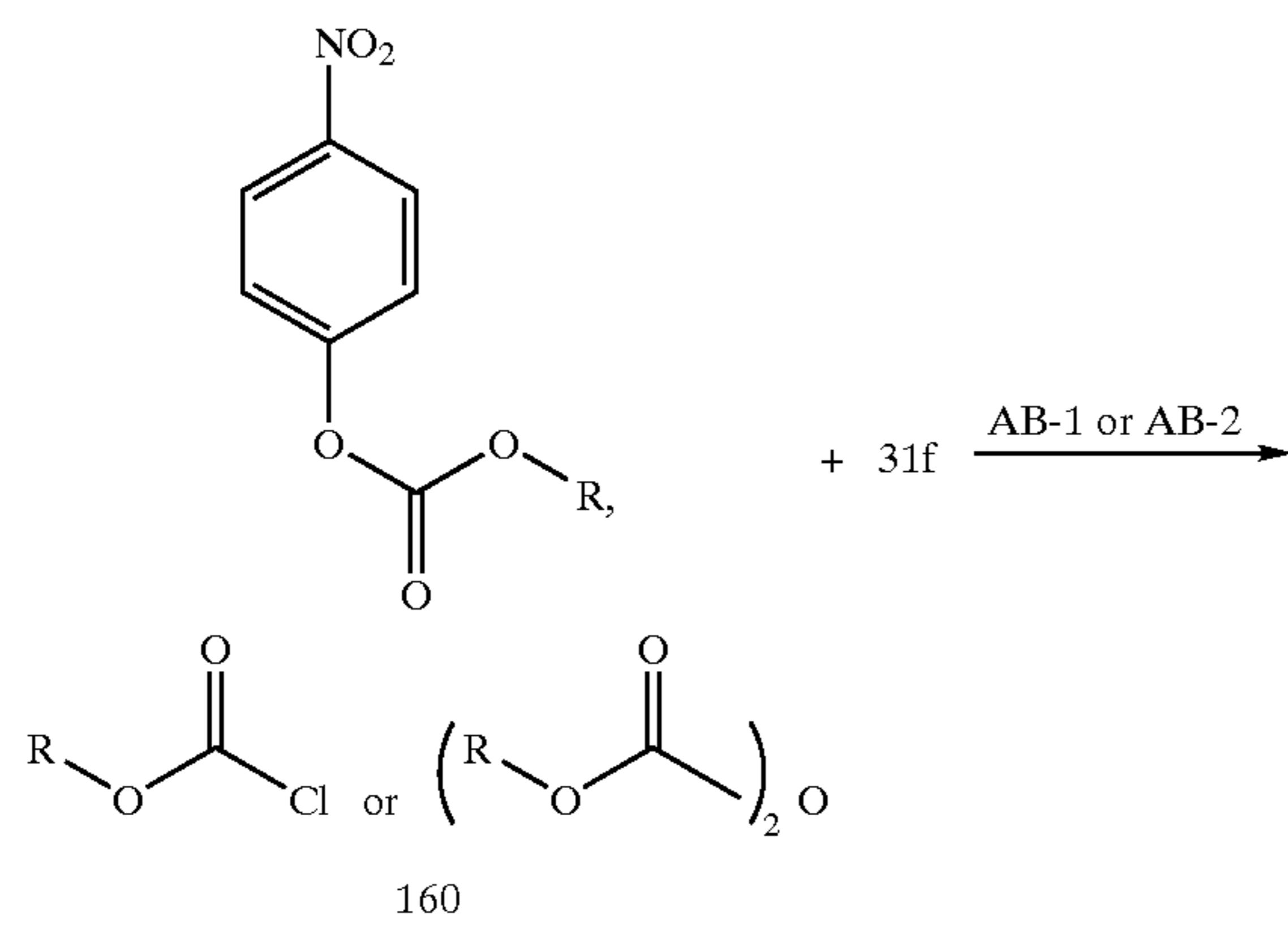
Scheme 20
