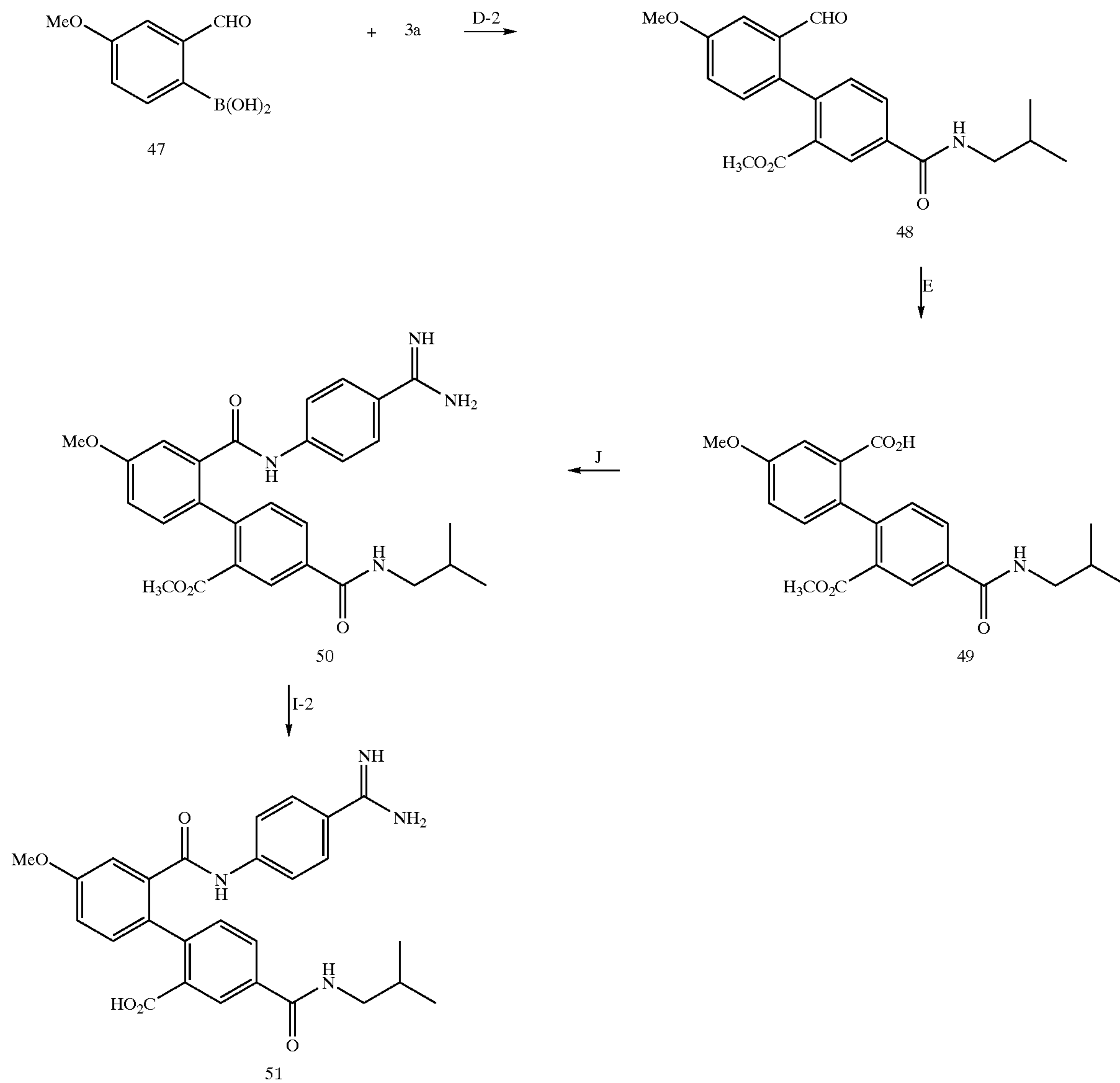
Scheme 8C
