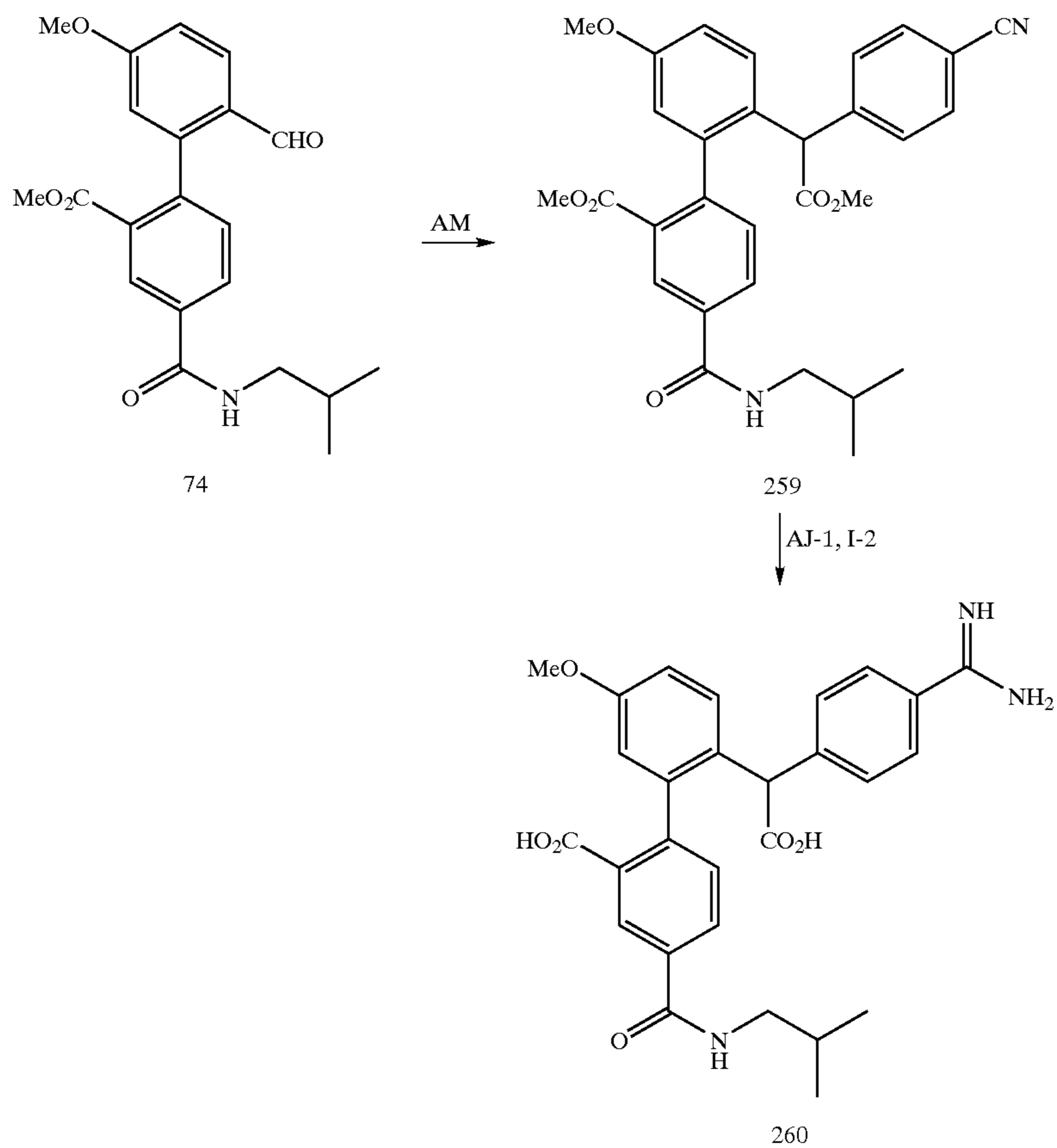
Scheme 38
