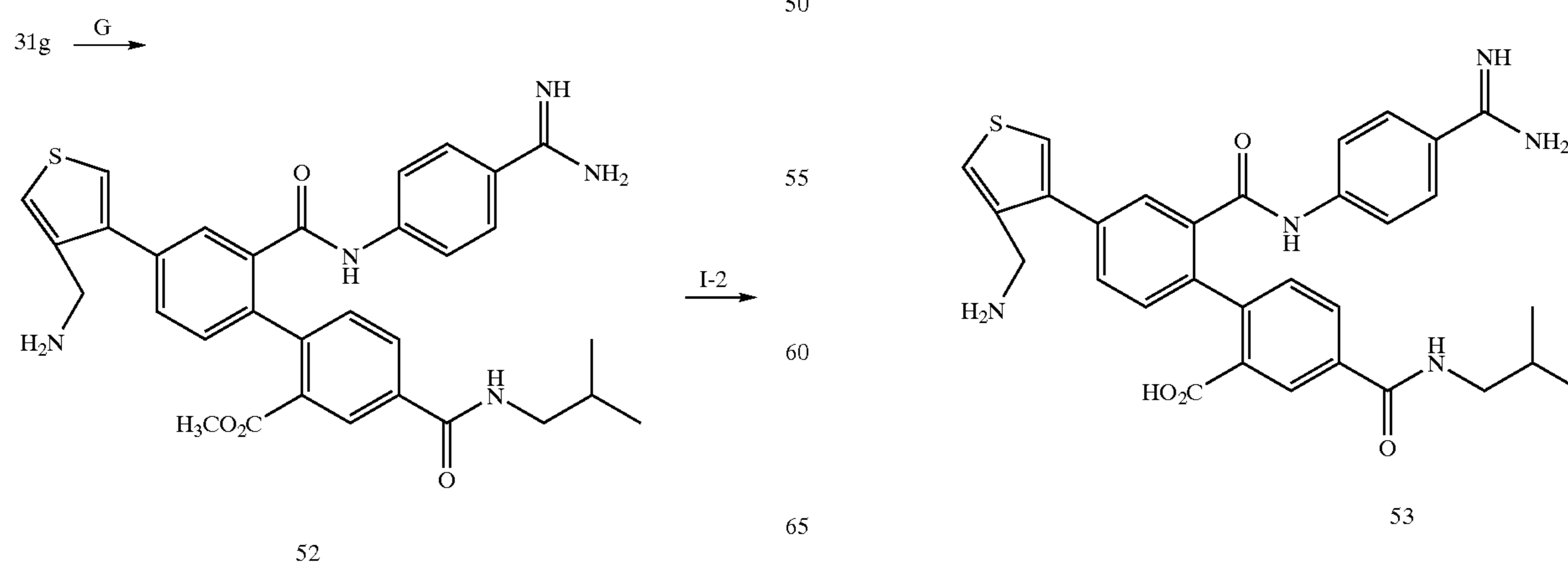
Scheme 8D
