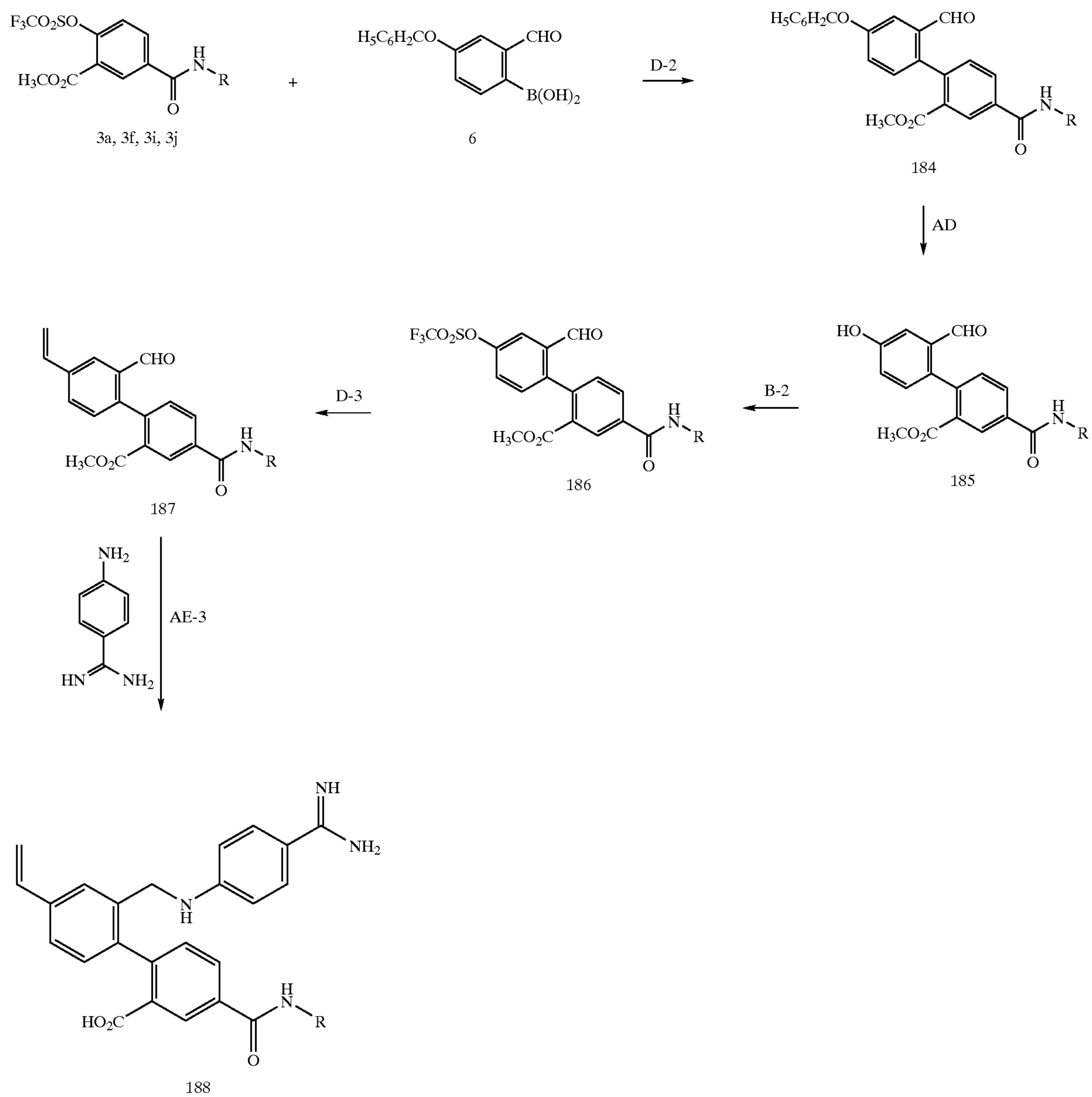
Scheme 24
