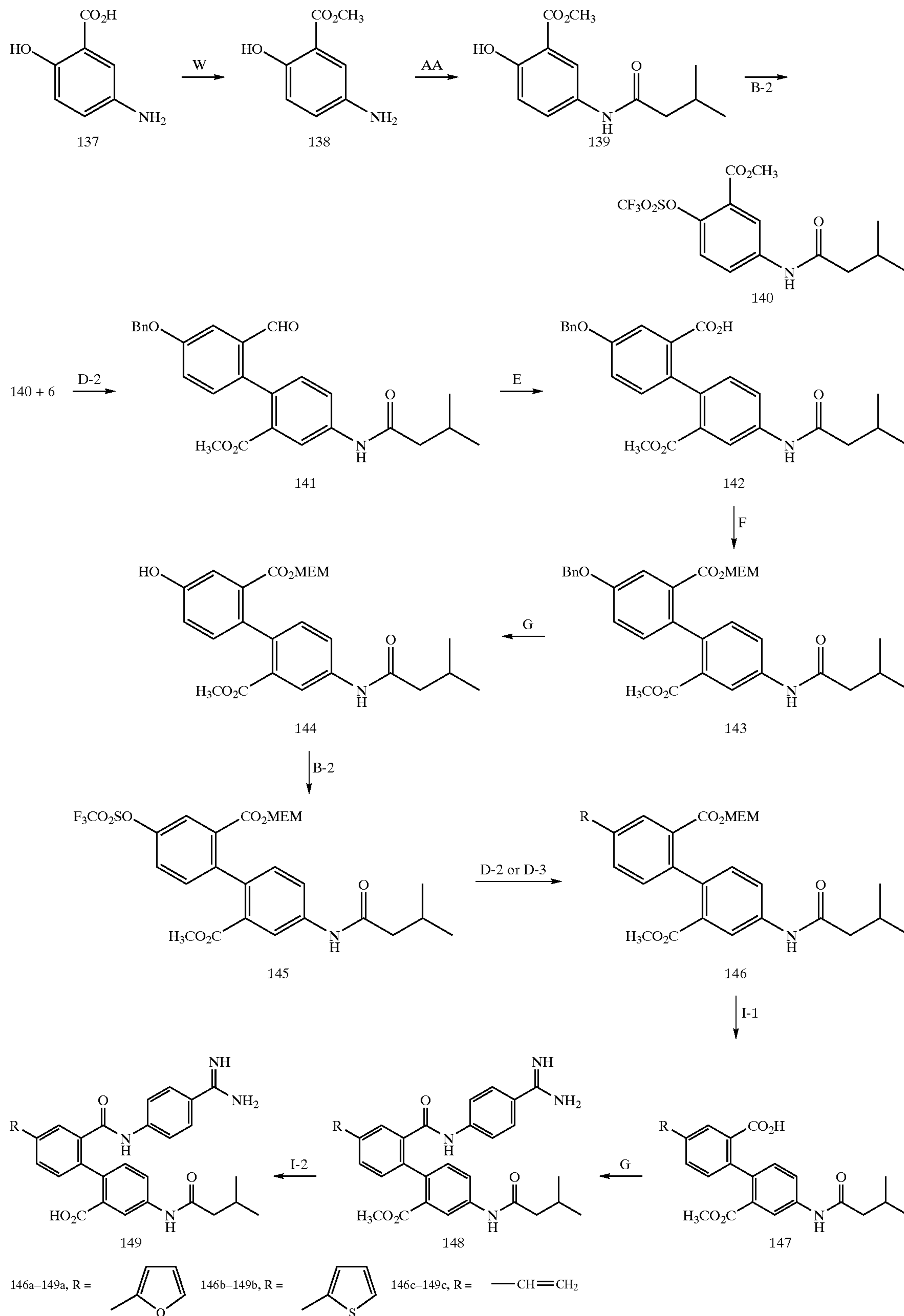
Scheme 18
