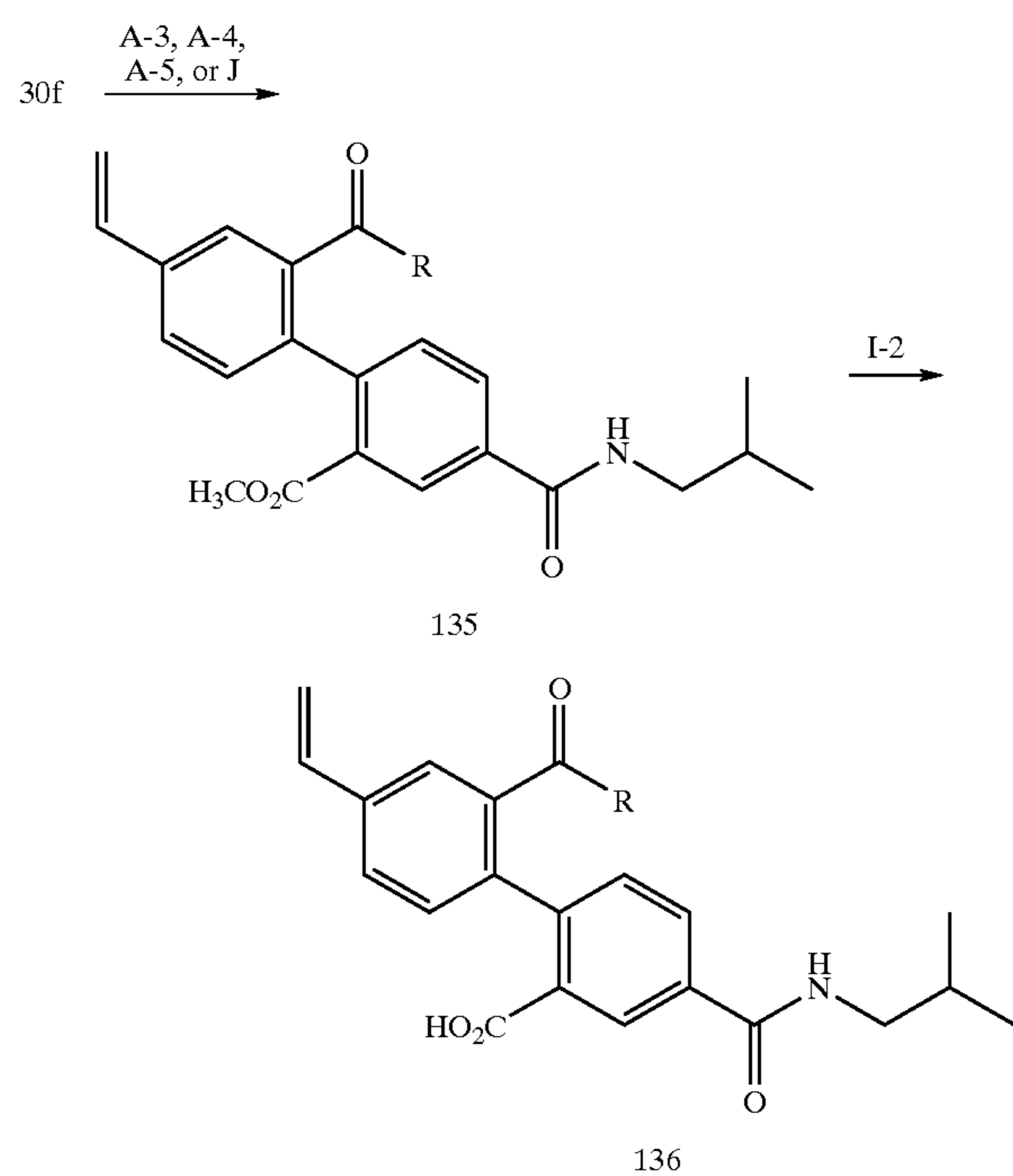
Scheme 17a
