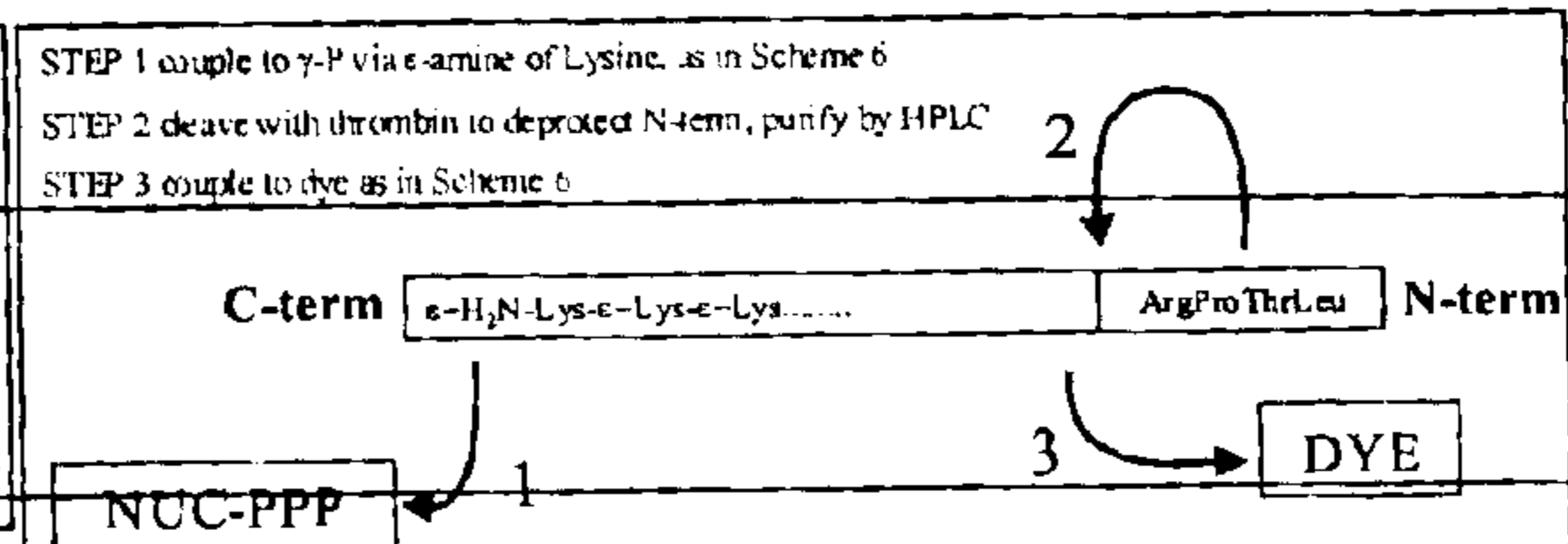
Scheme 8 - Peptide Deprotection By Thrombin Cleavage
