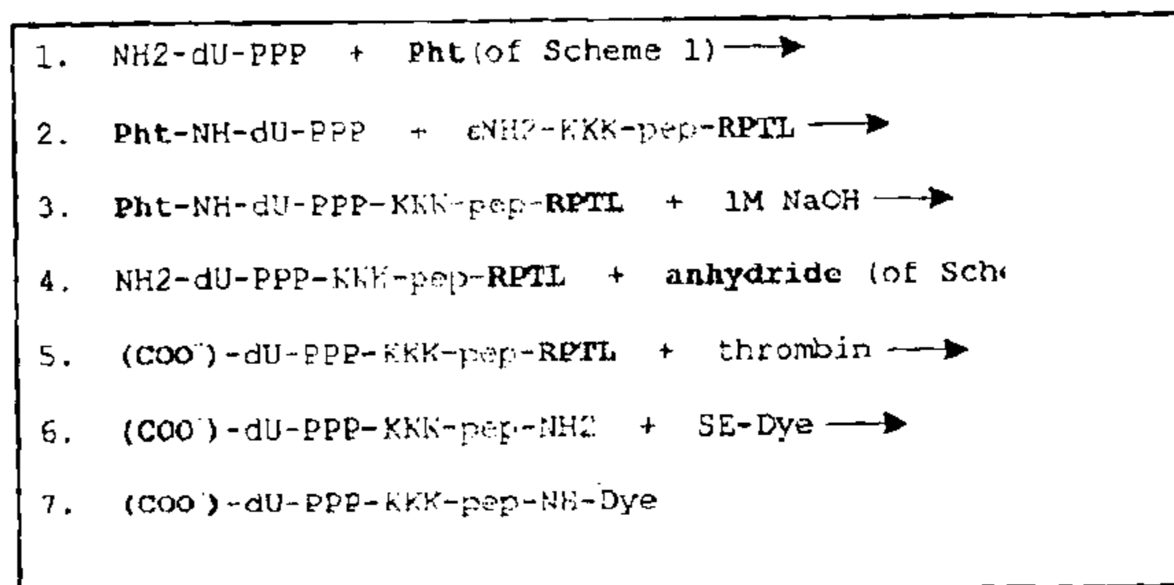
Scheme 10 - \gamma -dNTP With Carboxylated Base
