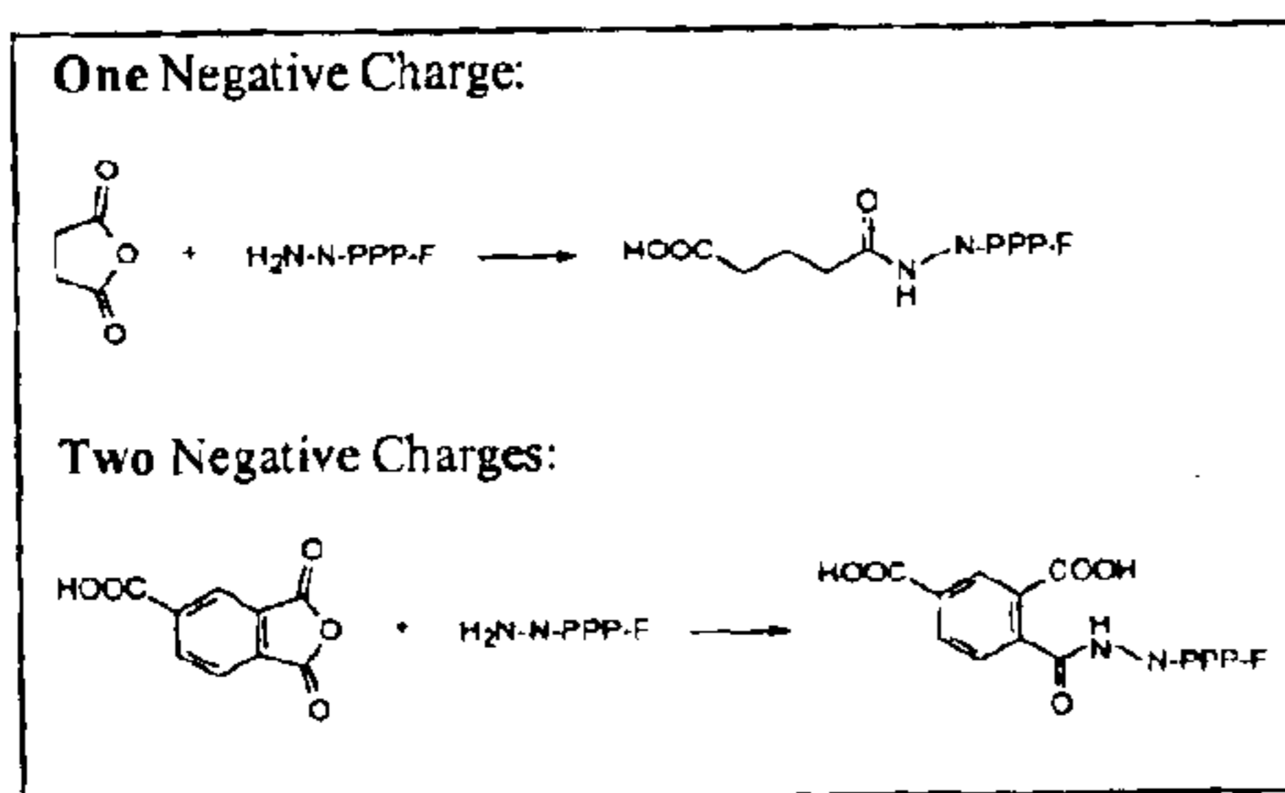
Scheme 9 - Add carboxylate to aminoallyl-dUTP
