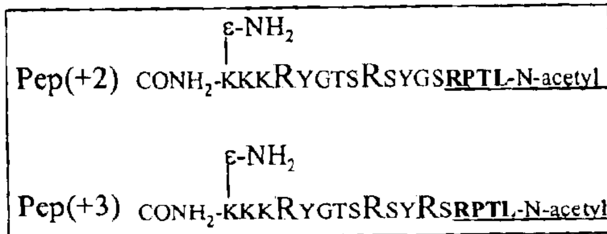
Scheme 7 - Peptide linkers (shown in C-to-N direction)
