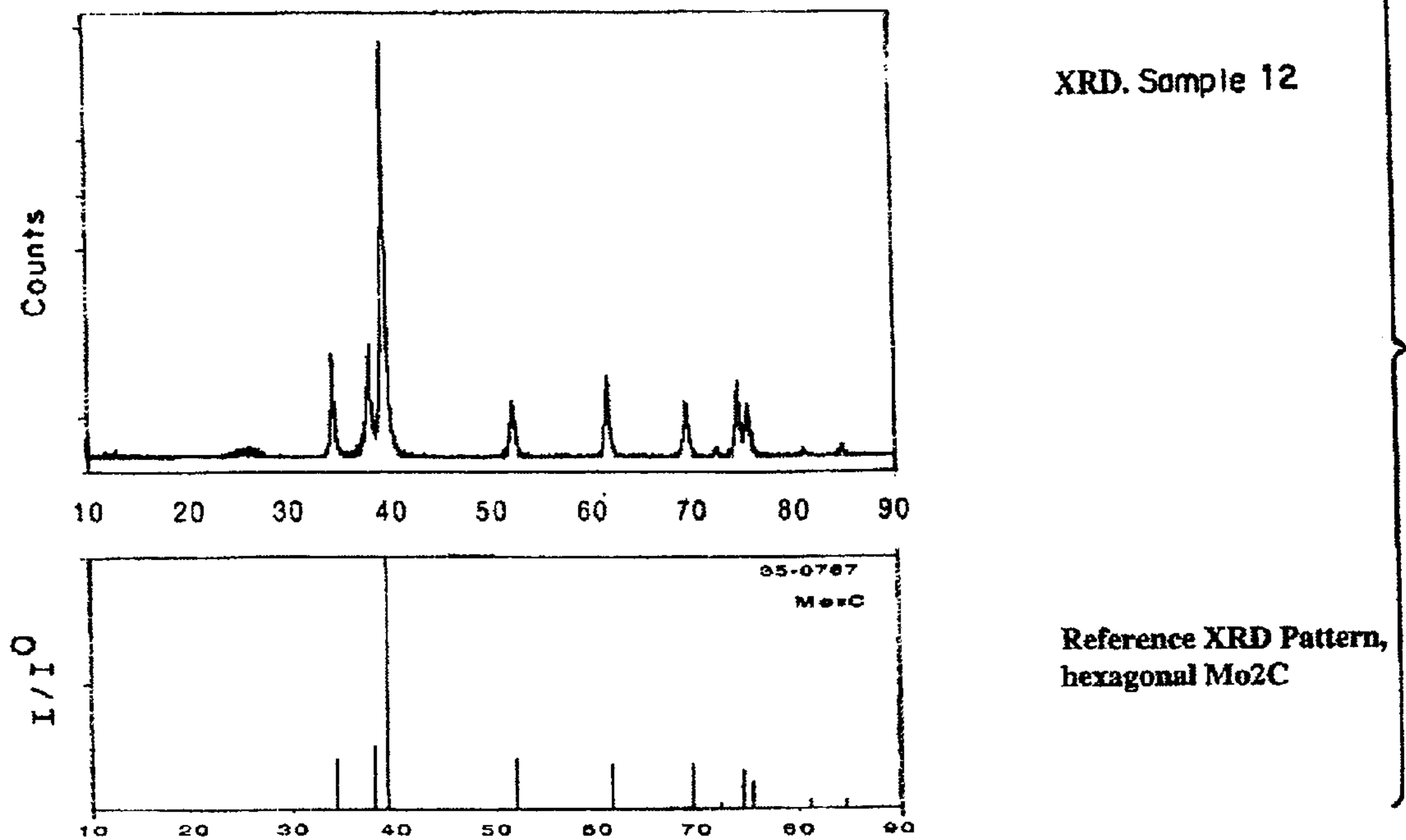
FIG.2A XRD and HRTEM of CARBIDE NANORODS
