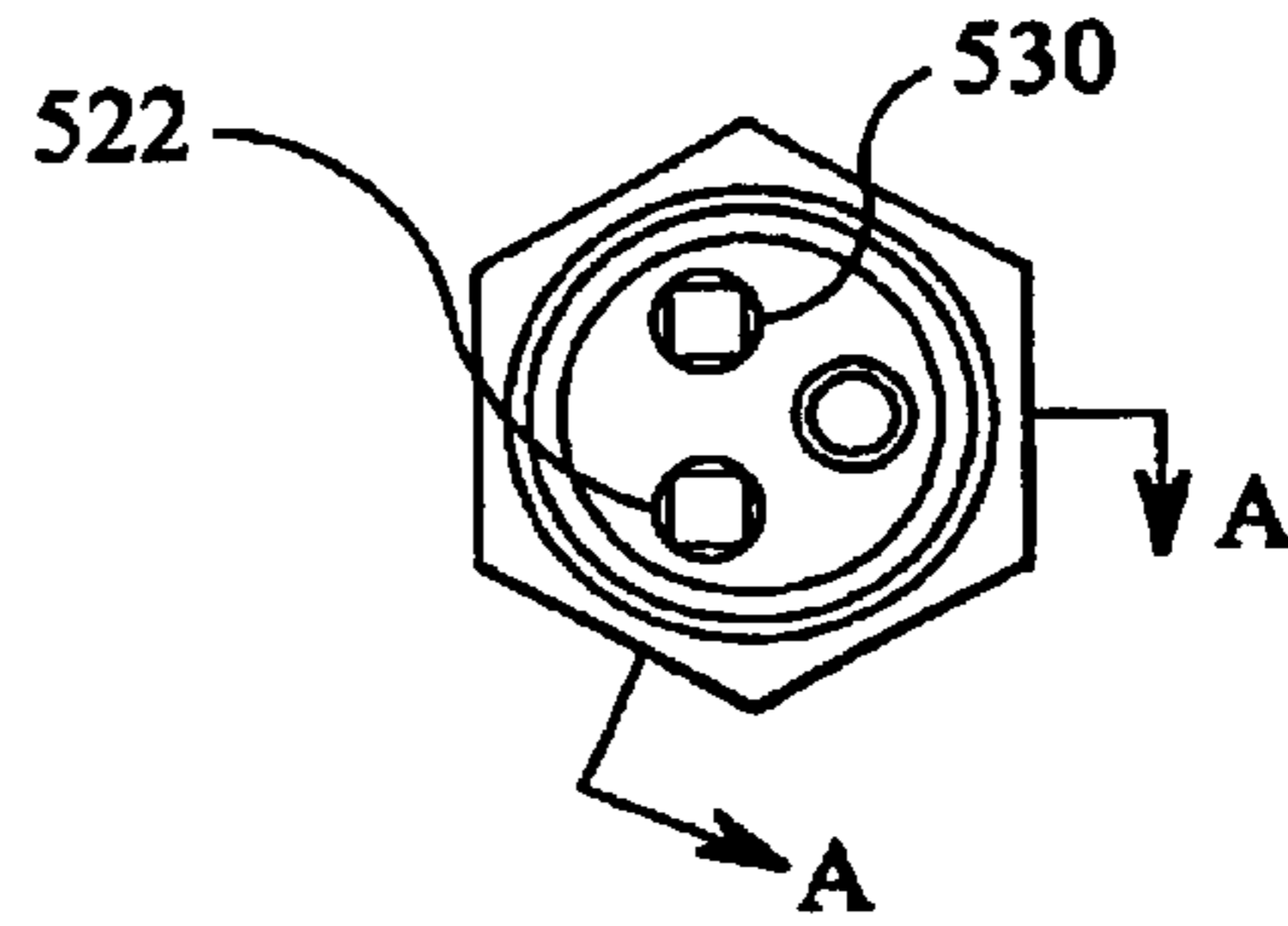
FIG 3 bottom view
