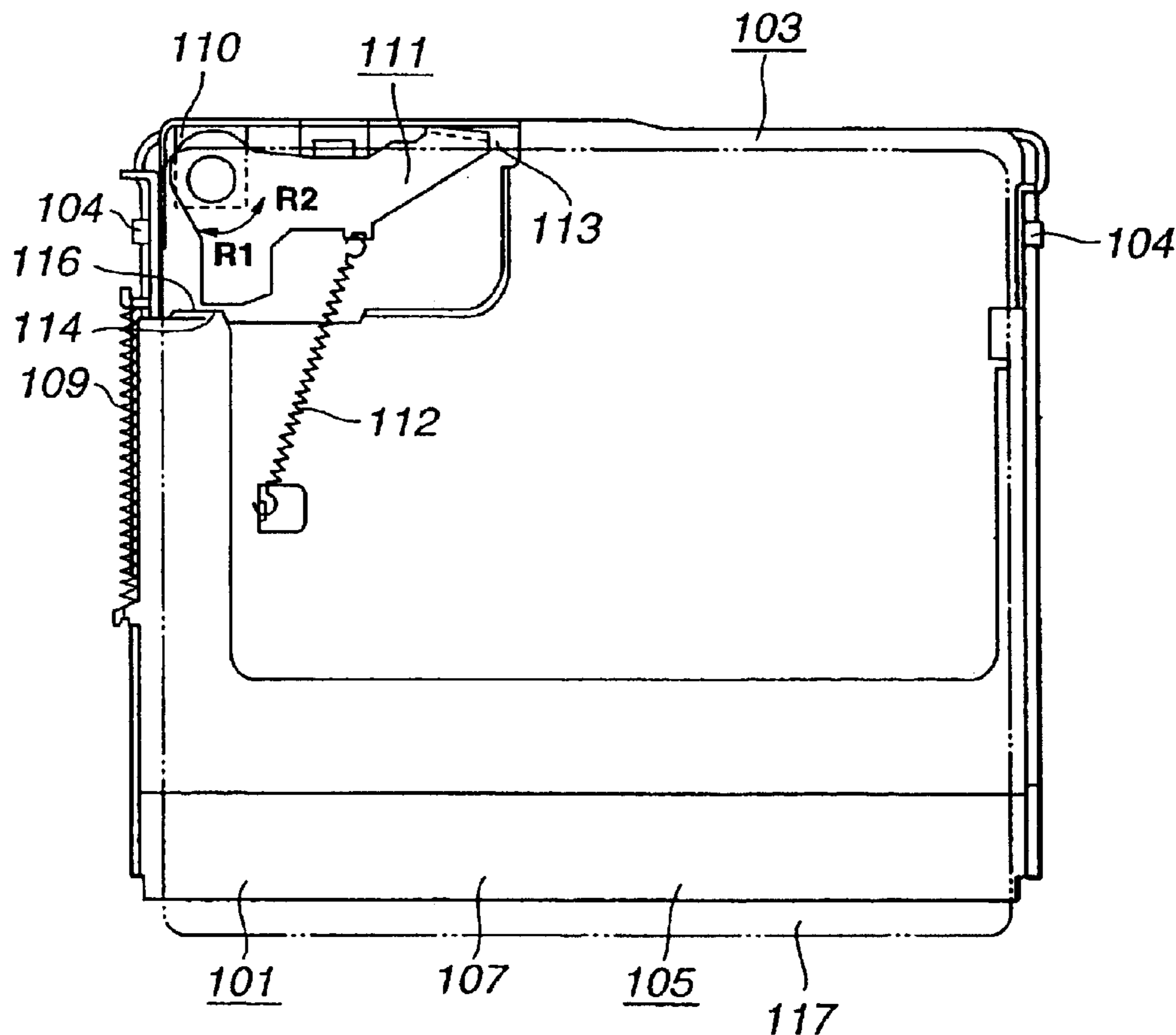
FIG. 3 (PRIOR ART)
