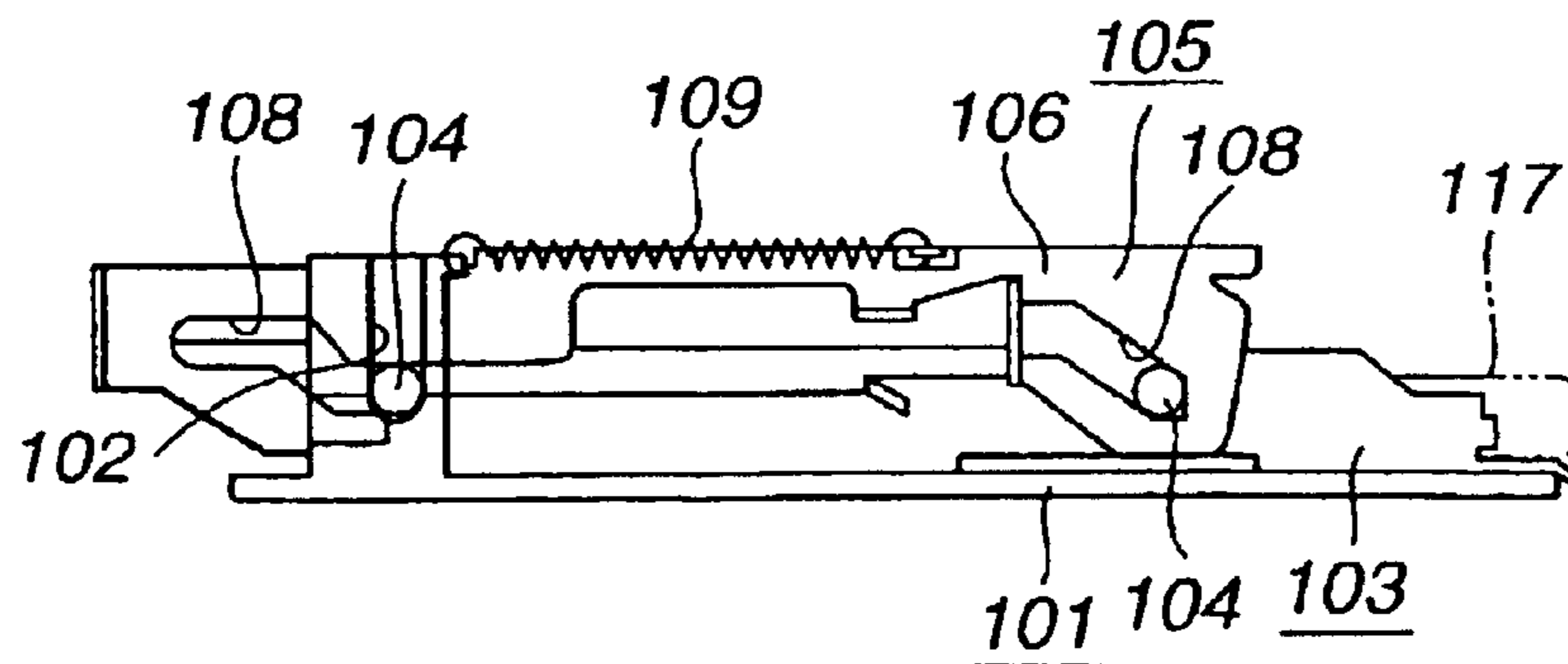
FIG. 5 (PRIOR ART)
