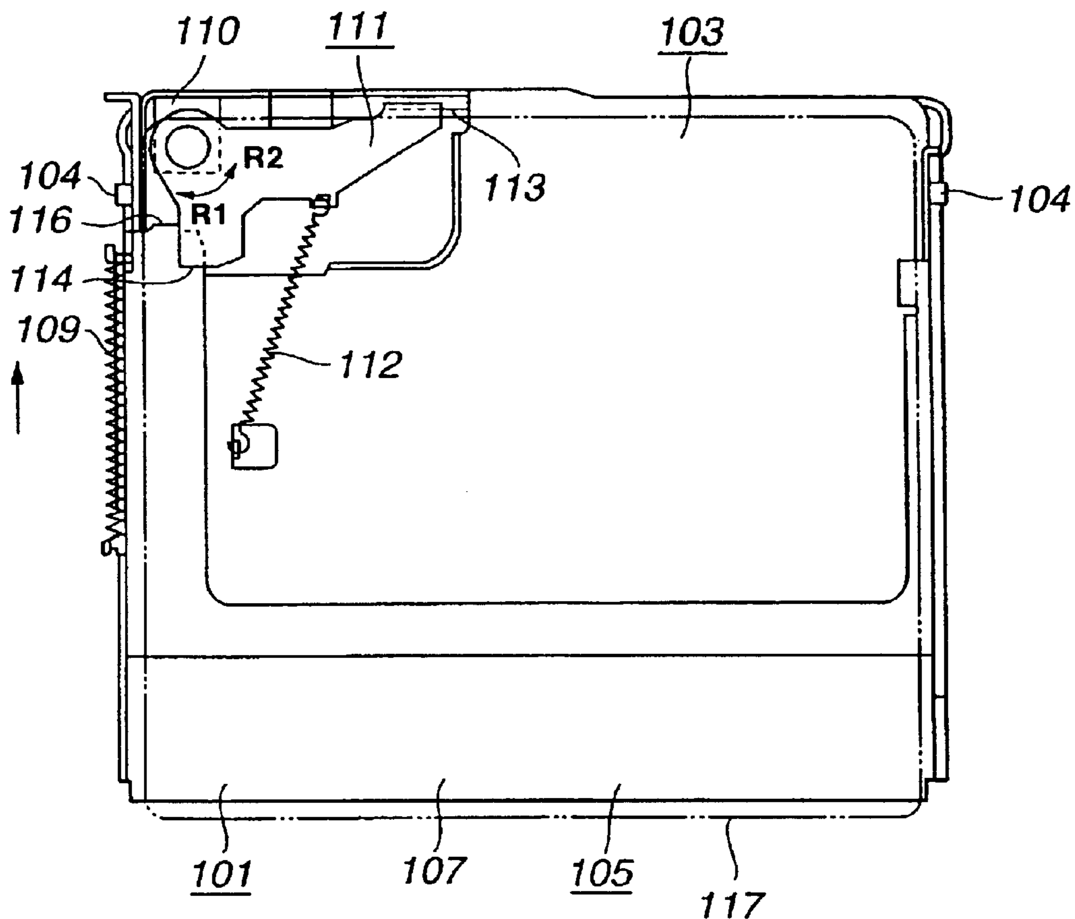
FIG. 4 (PRIOR ART)
