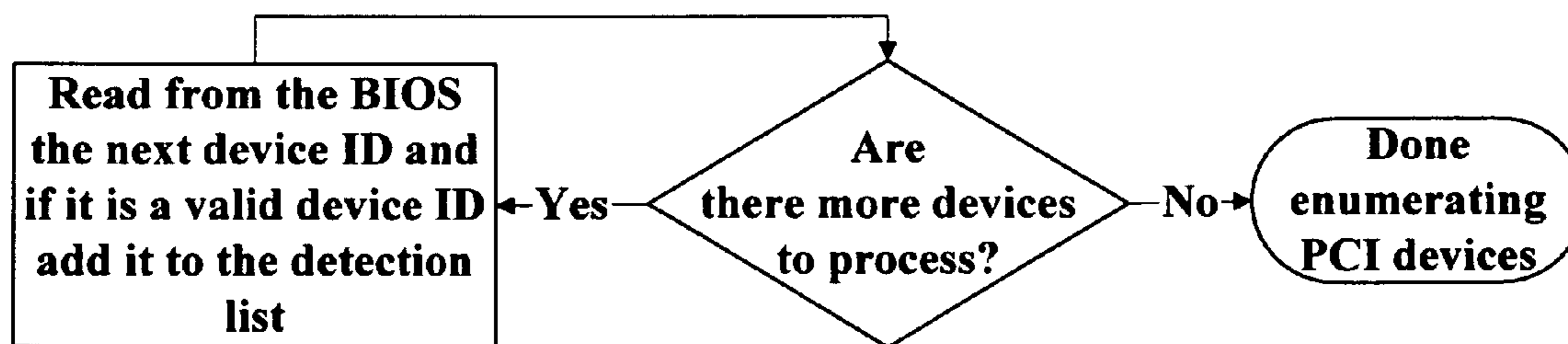
Figure 6C
