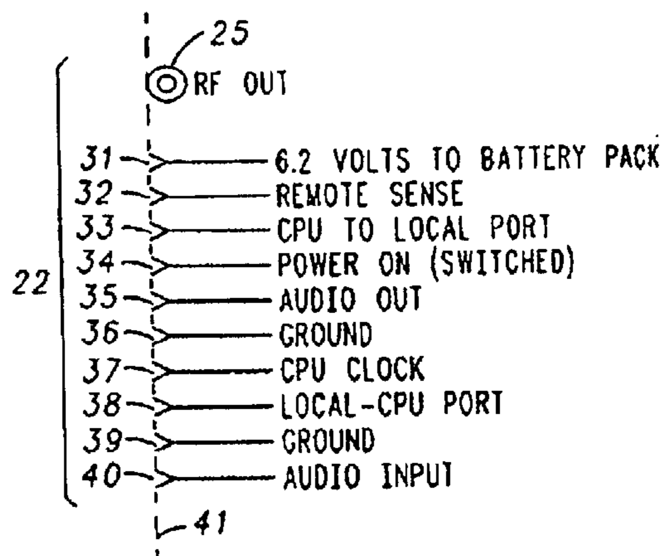
-PRIOR ART-
