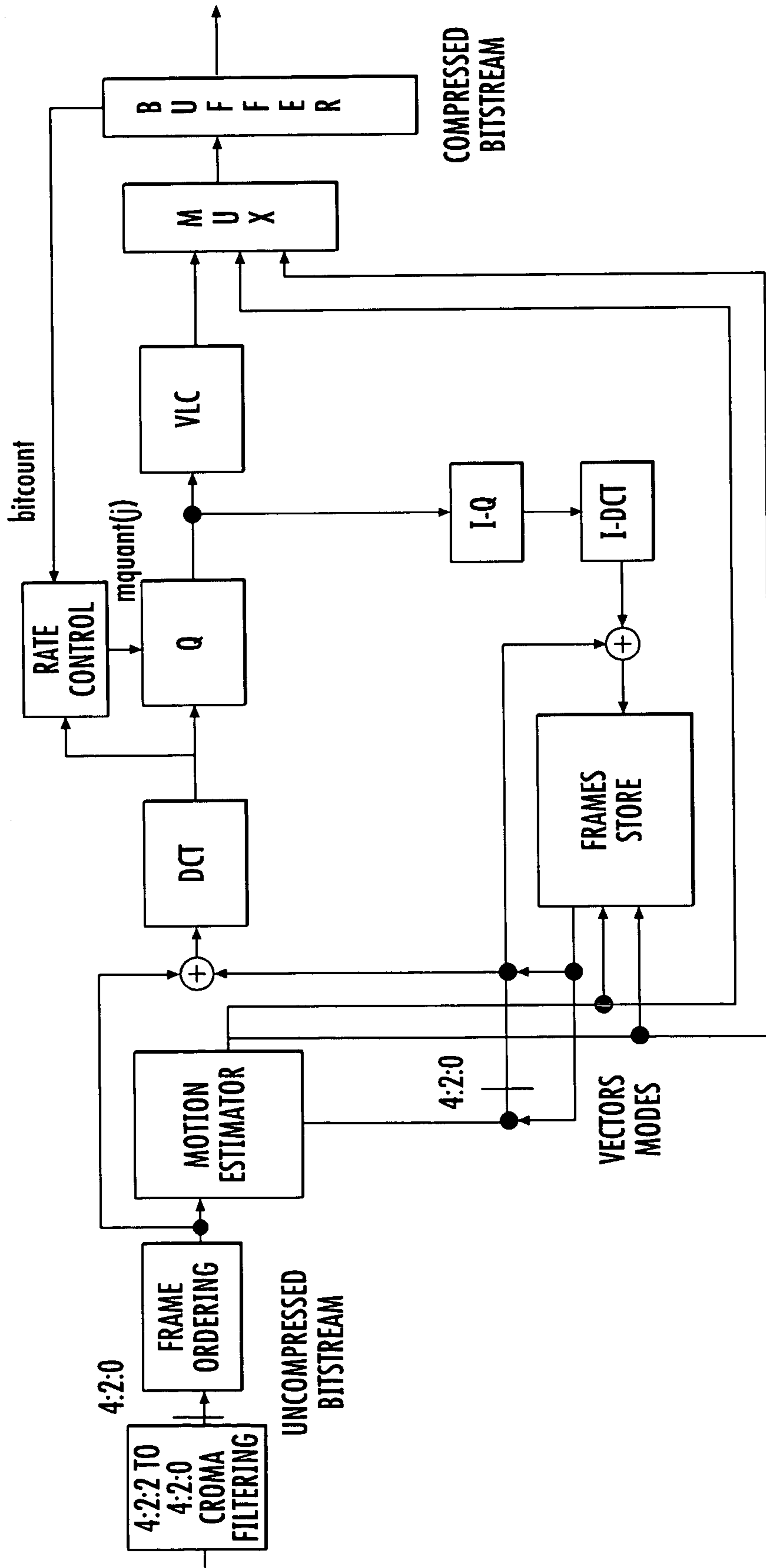
FIG. 2 (PRIOR ART)
