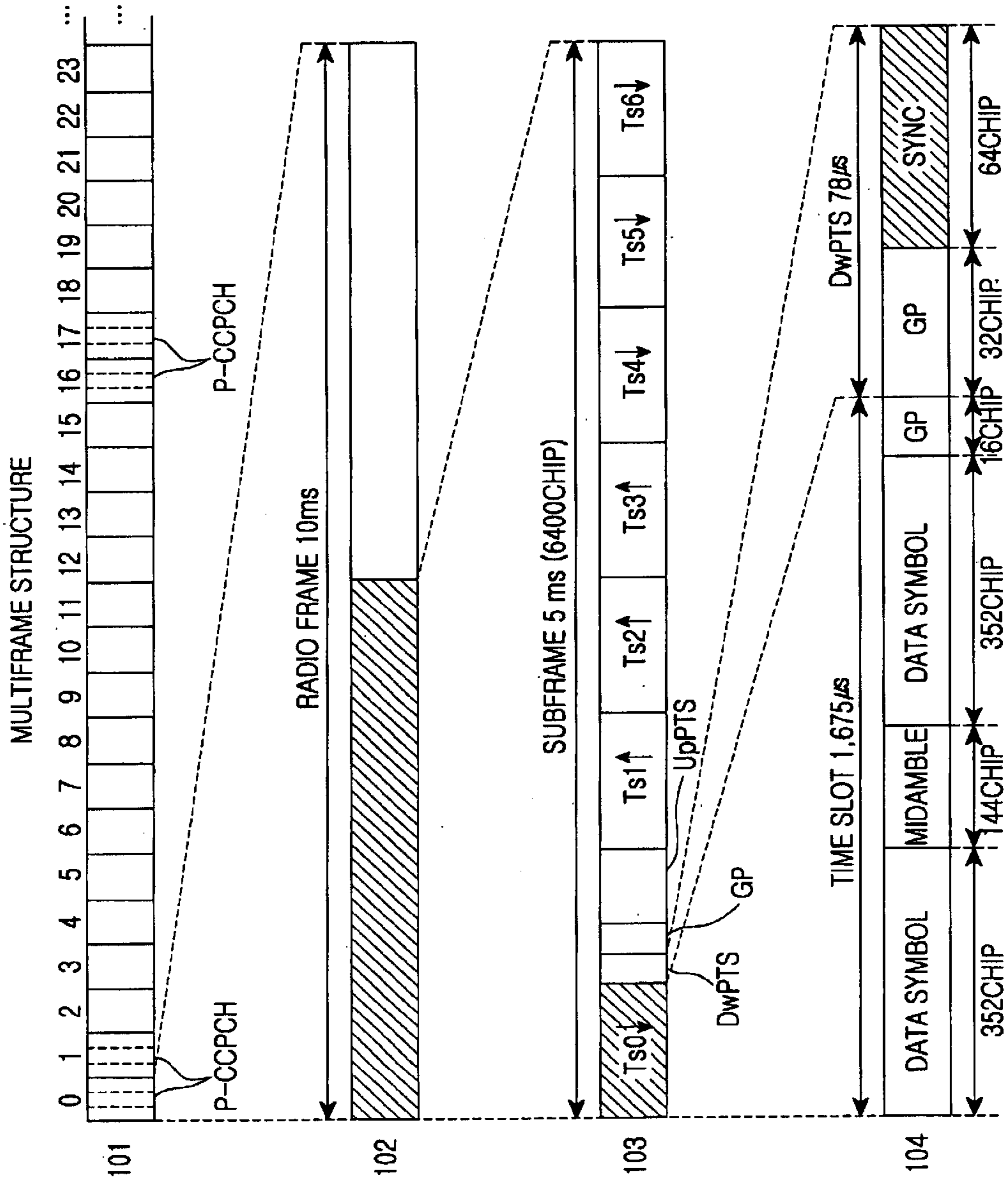
FIG. 1 (PRIOR ART)
