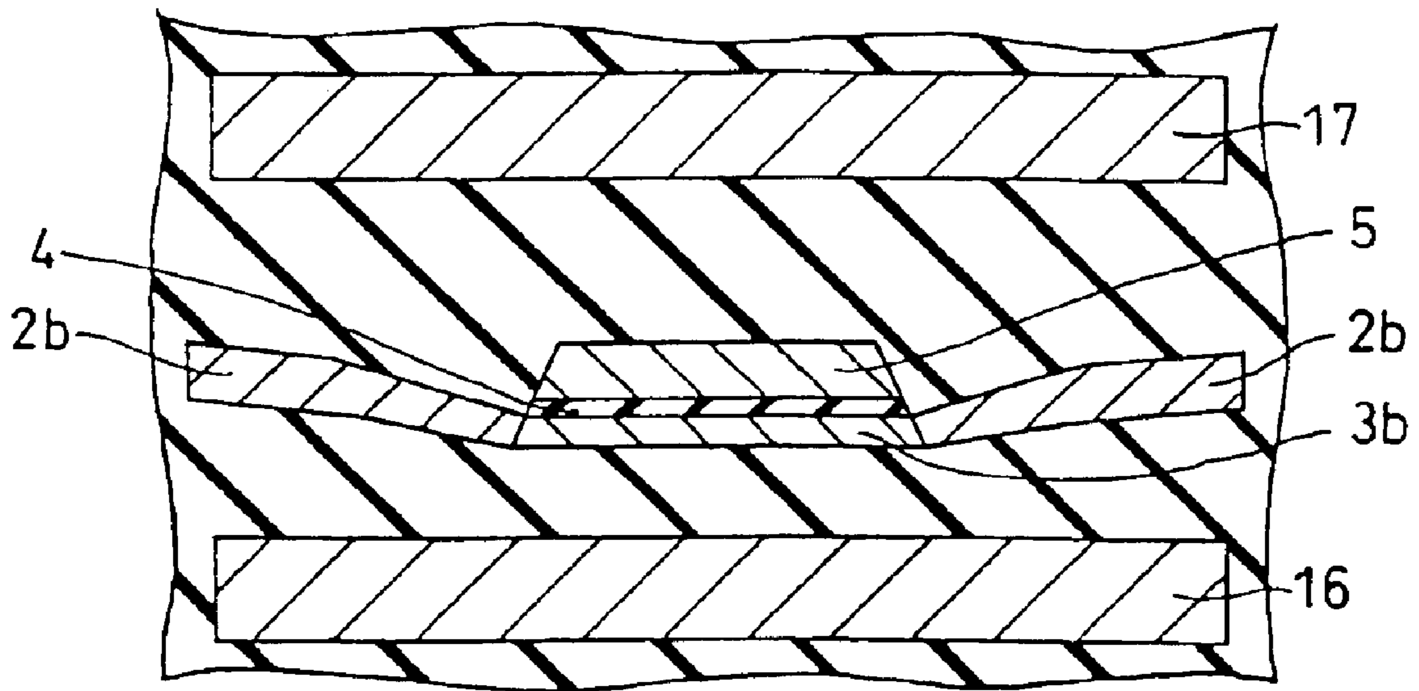
FIG. 3 (PRIOR ART)
