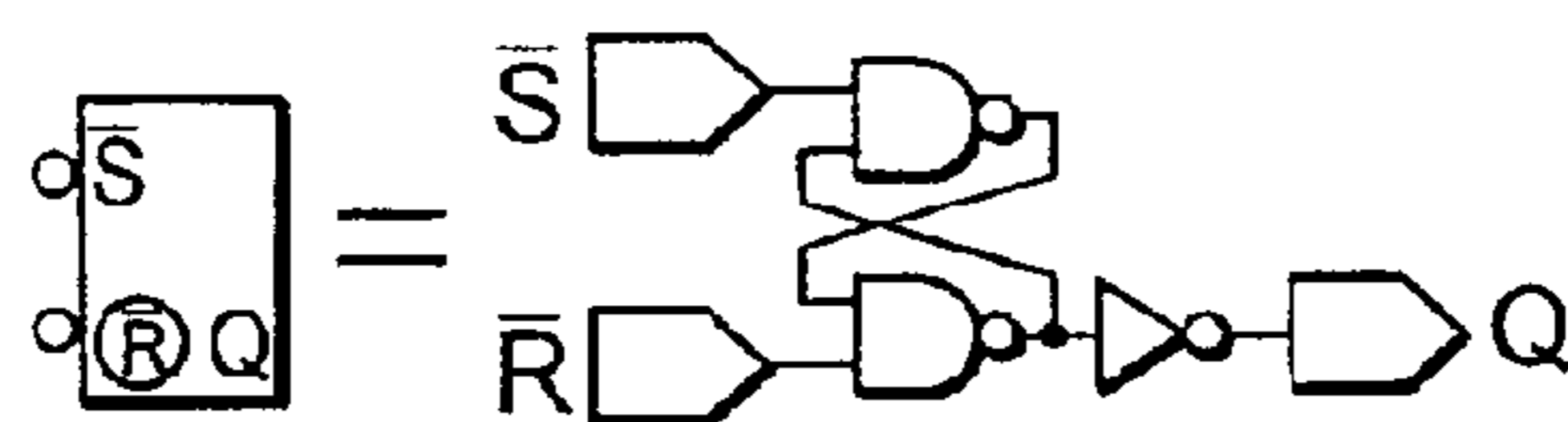
R-S FLIP-FLOP
