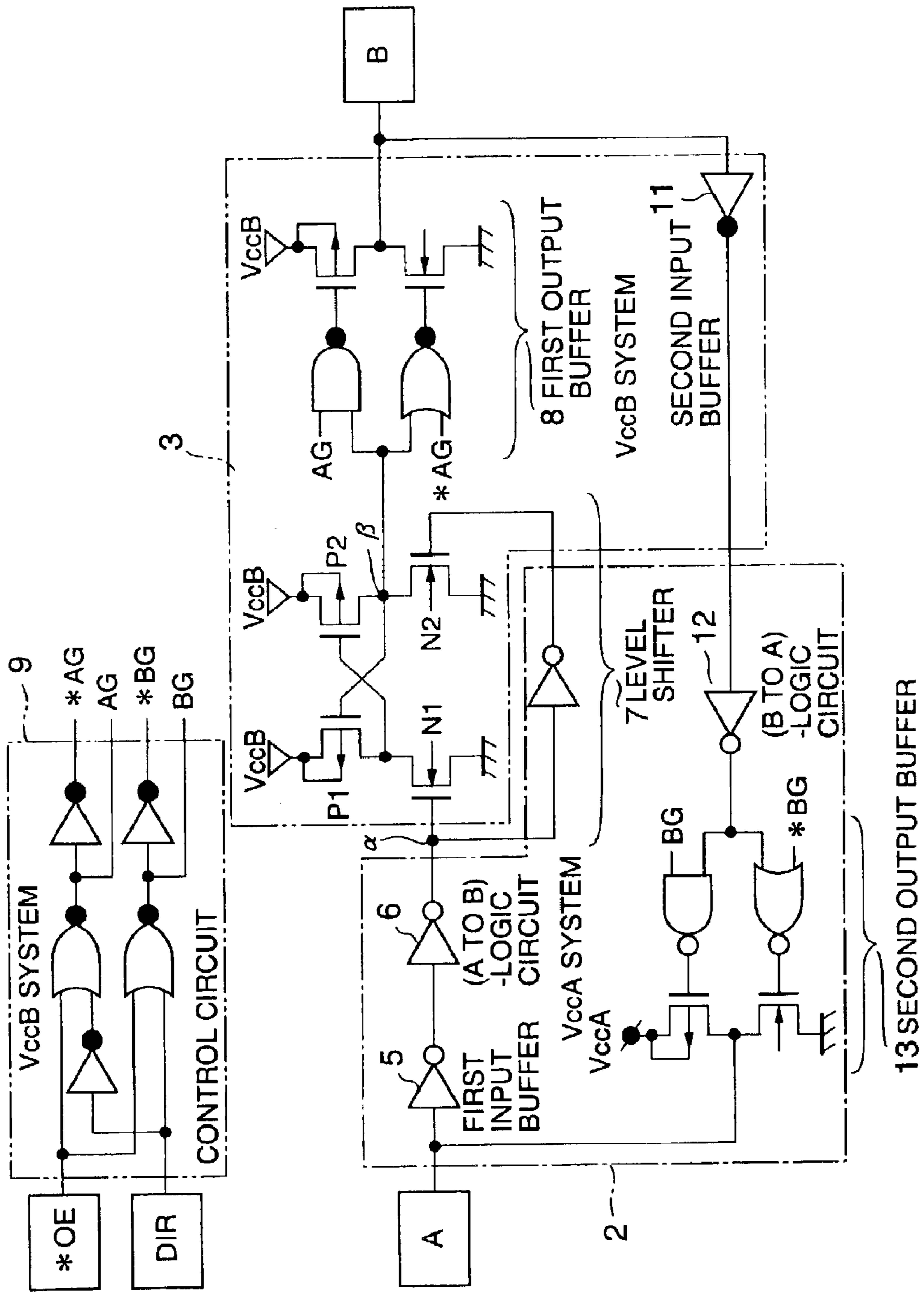
FIG. 21 PRIOR ART
