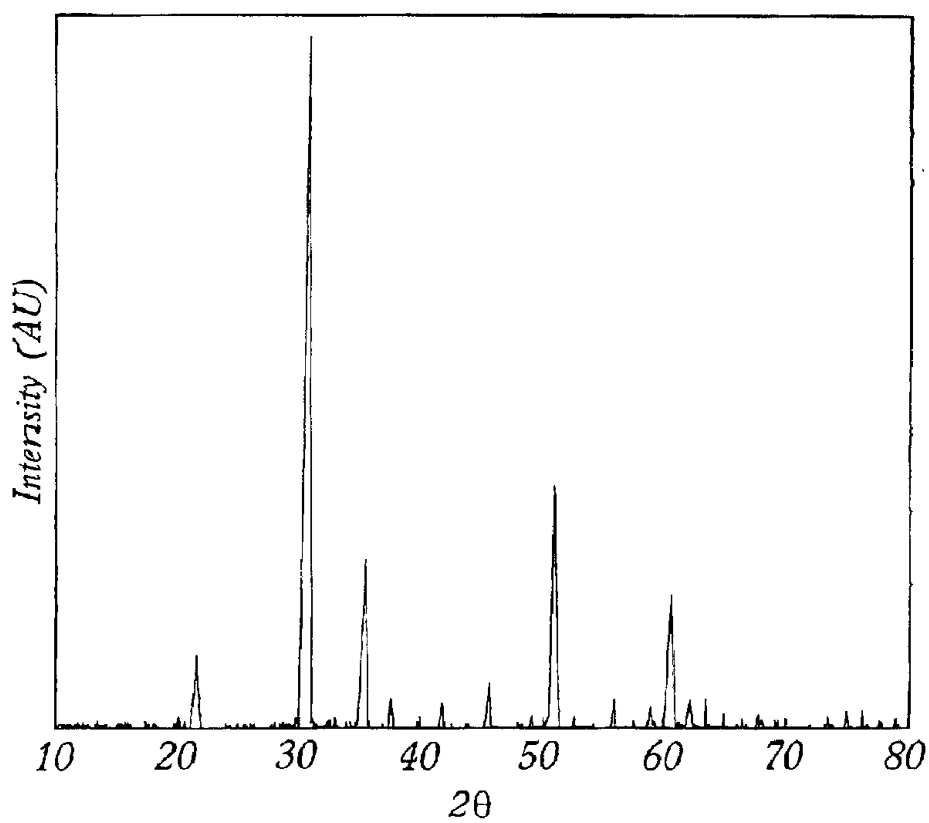
XDR spectrum of the indium tin oxide nanopowder
