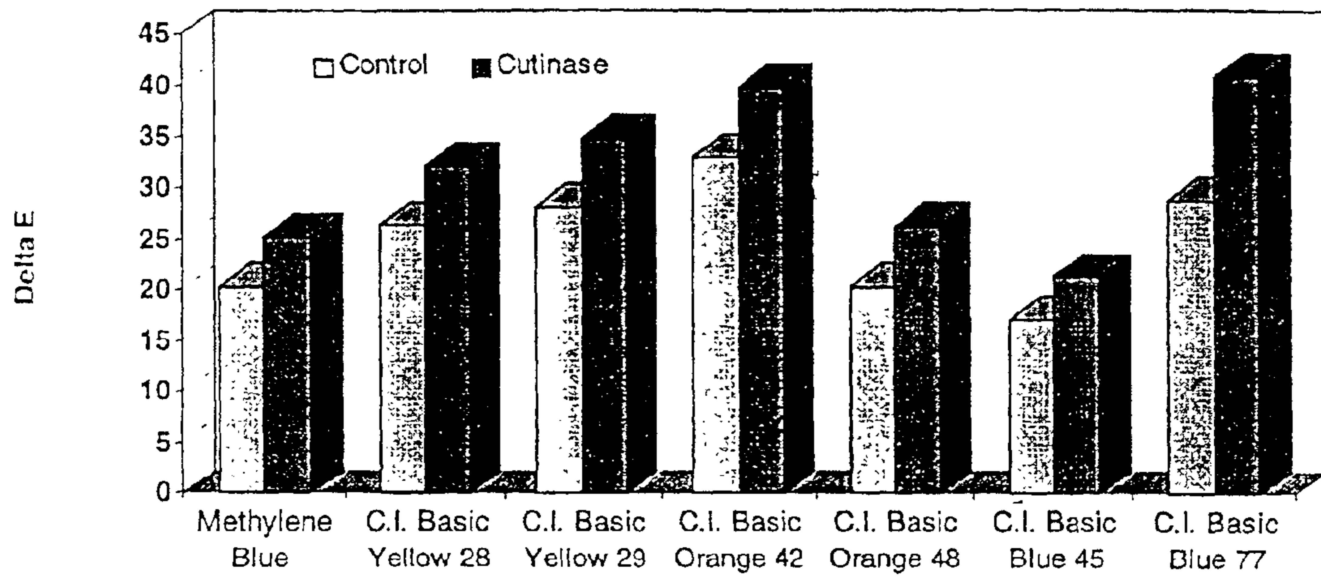
Total Color Difference after Dyeing with Basic Dyes on Dacron® 64
