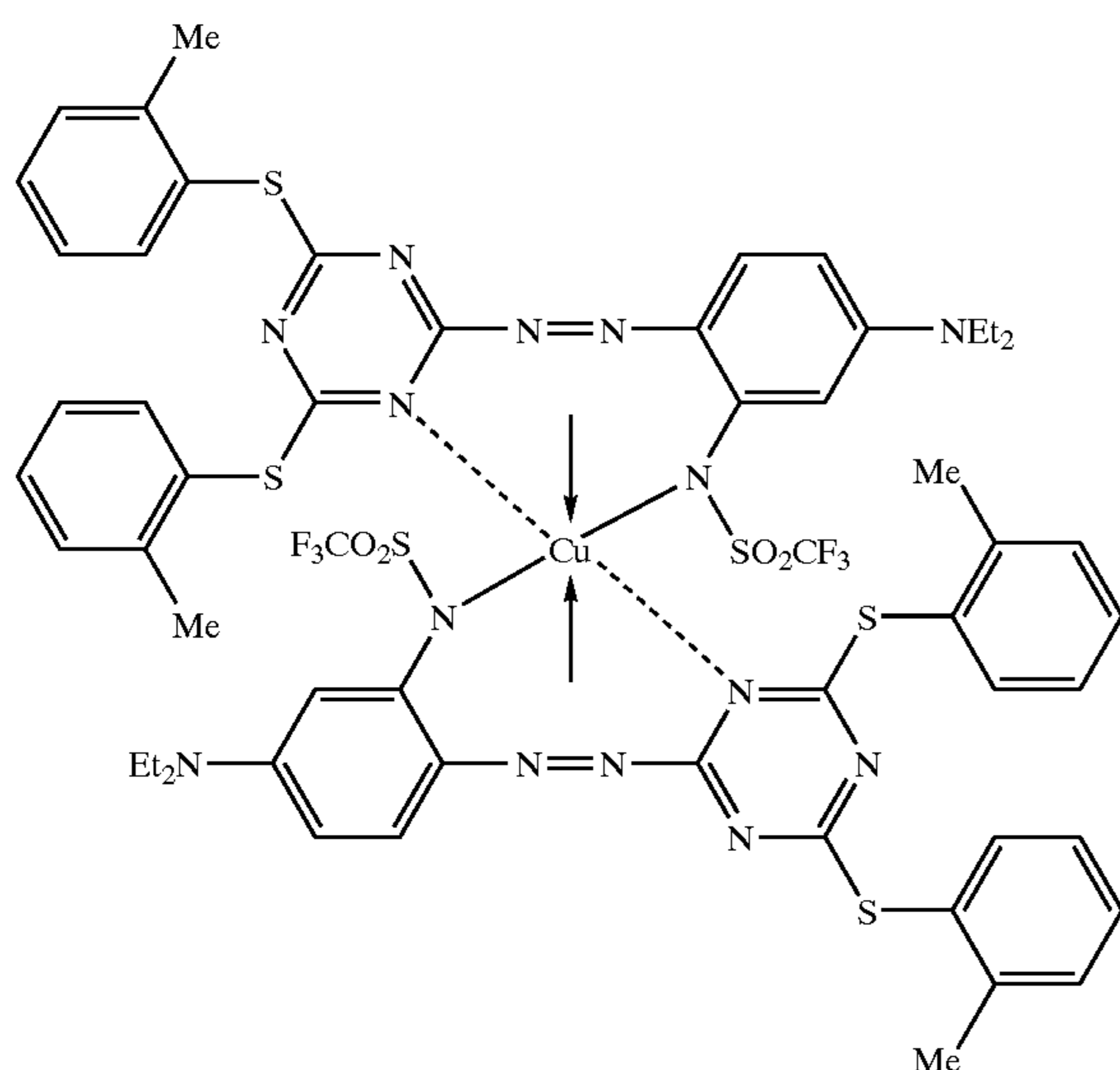
Structural Formula (1)
