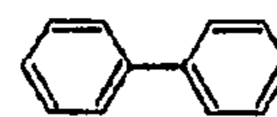
Biphenyl (BP)
