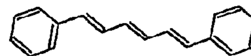
1,6-Diphenylhexatriene (DPH)
