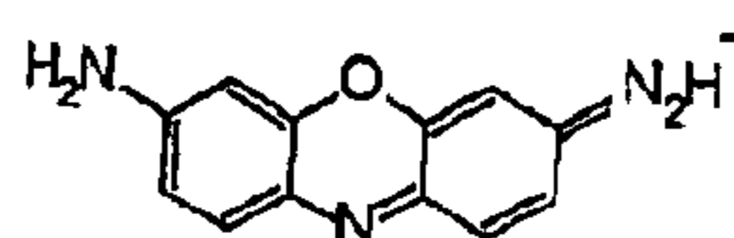
Oxonine (Ox) -
