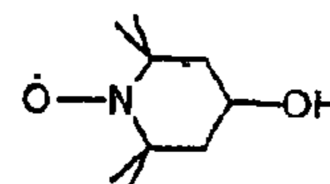
Hydroxy-TEMPO
