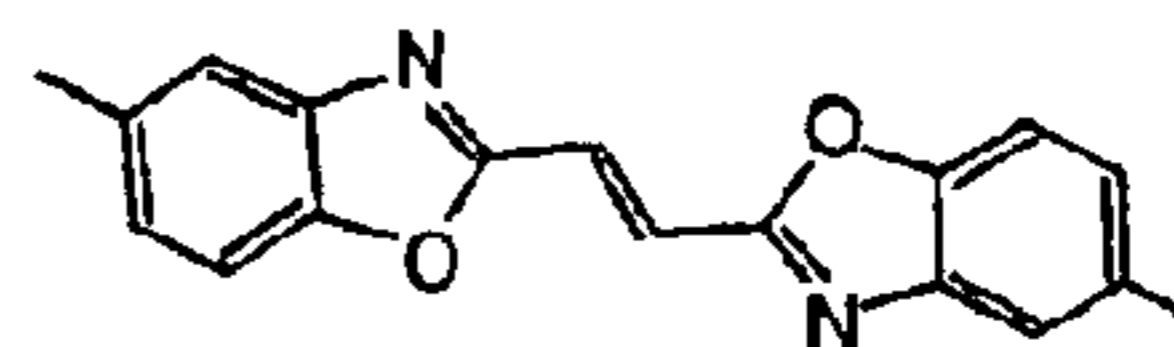
1,2-bis-<5-methyl-benzoxazol-2-yl>-ethene (MBOXE)
