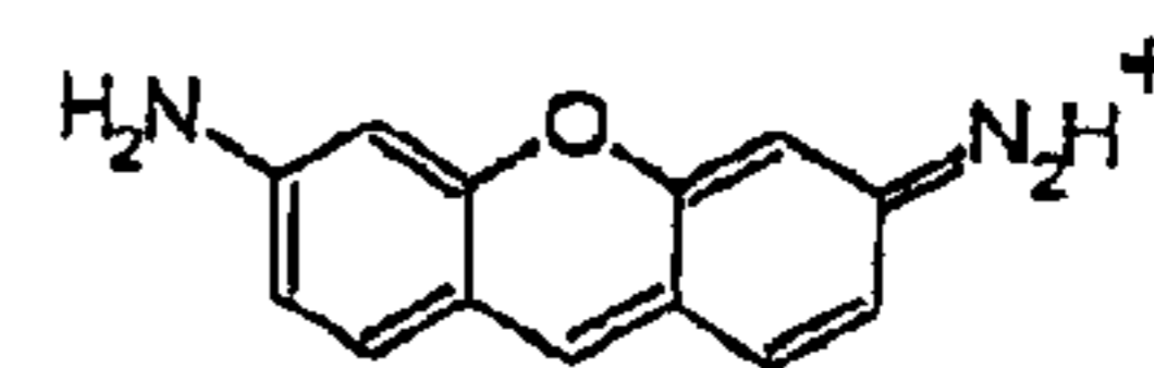
Pyronine (Py)
