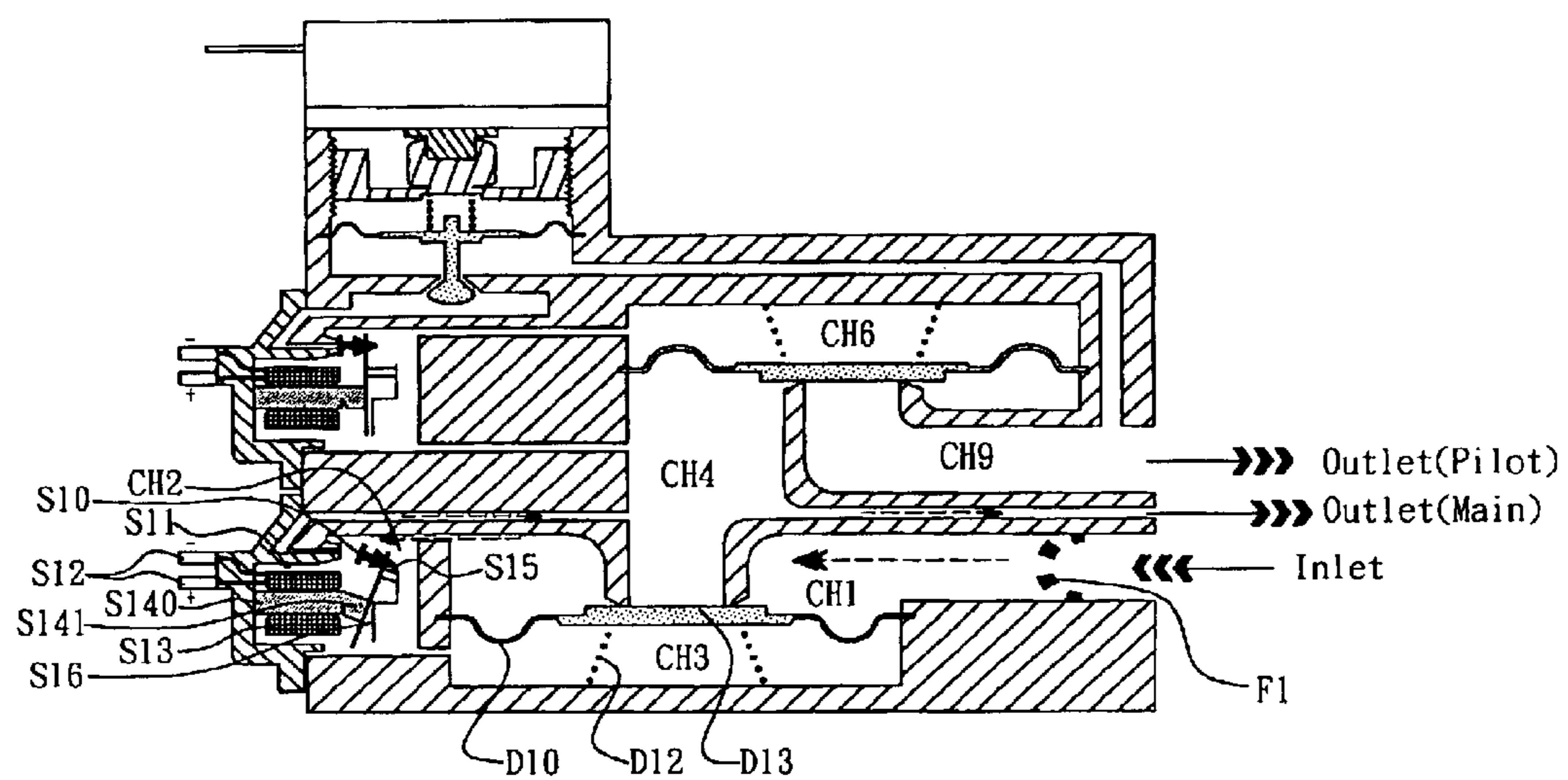
FIG. 4 -First Step[S1 opened]
