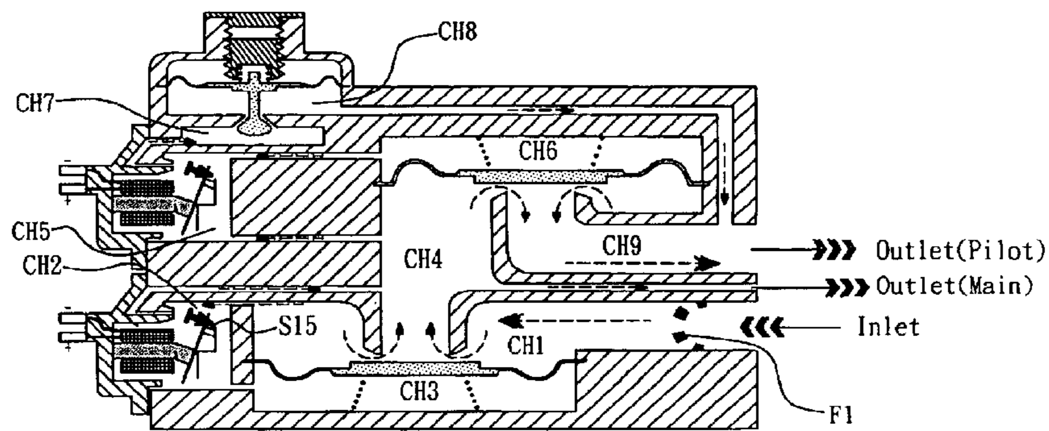
FIG. 9 -Final Step of the opening/closing gas supply
