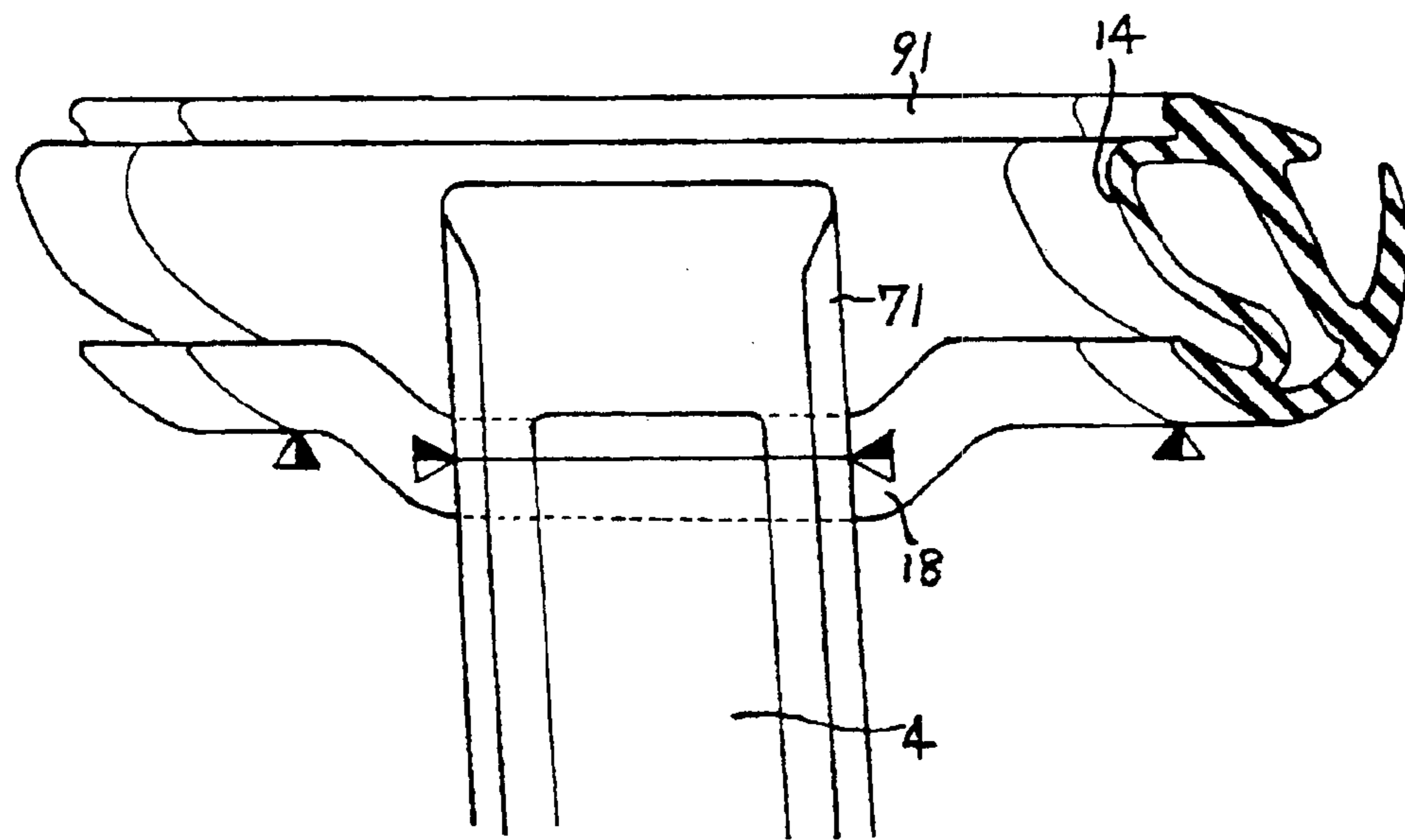
FIG. 12 (PRIOR ART)
