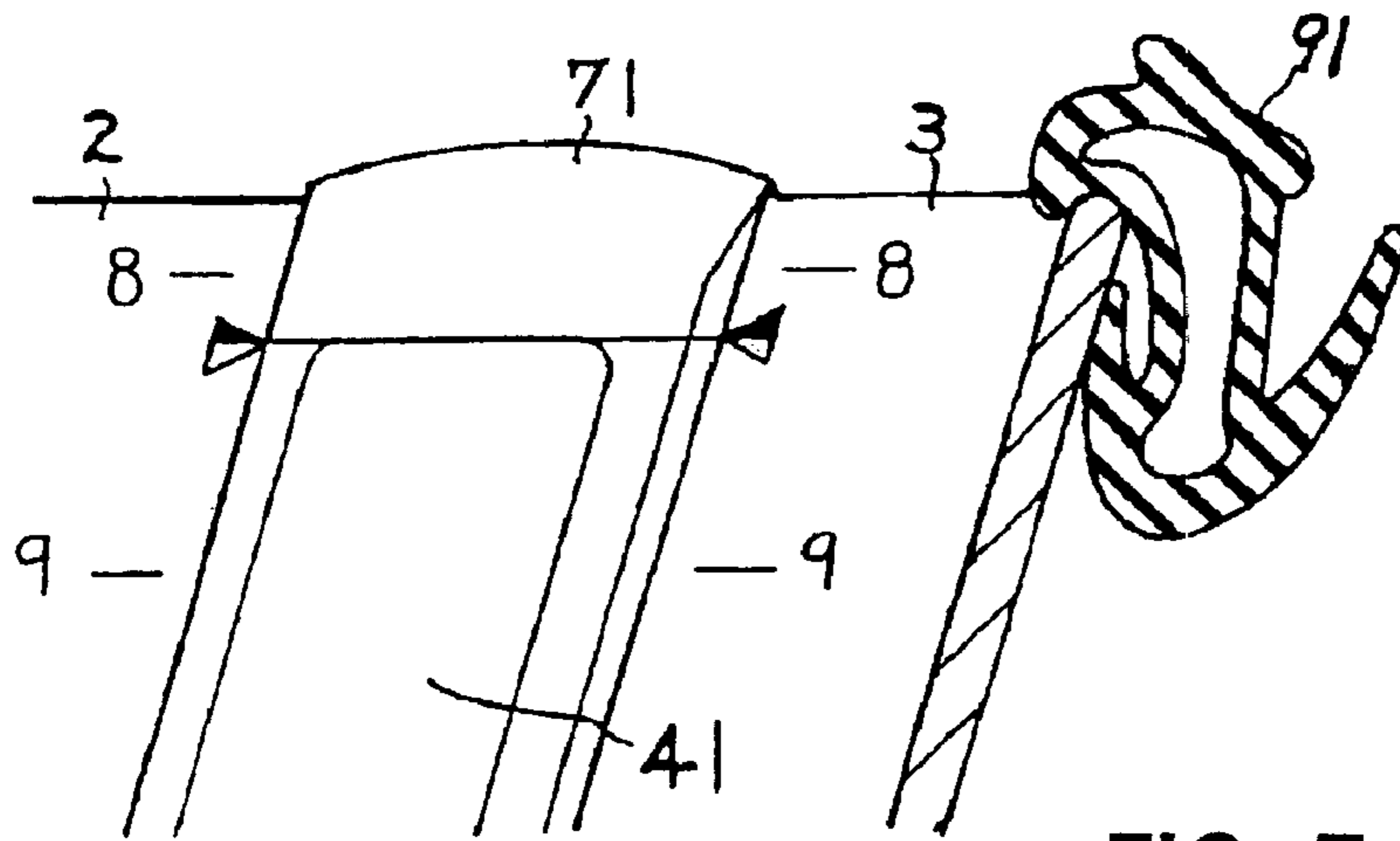
FIG. 7 (PRIOR ART)
