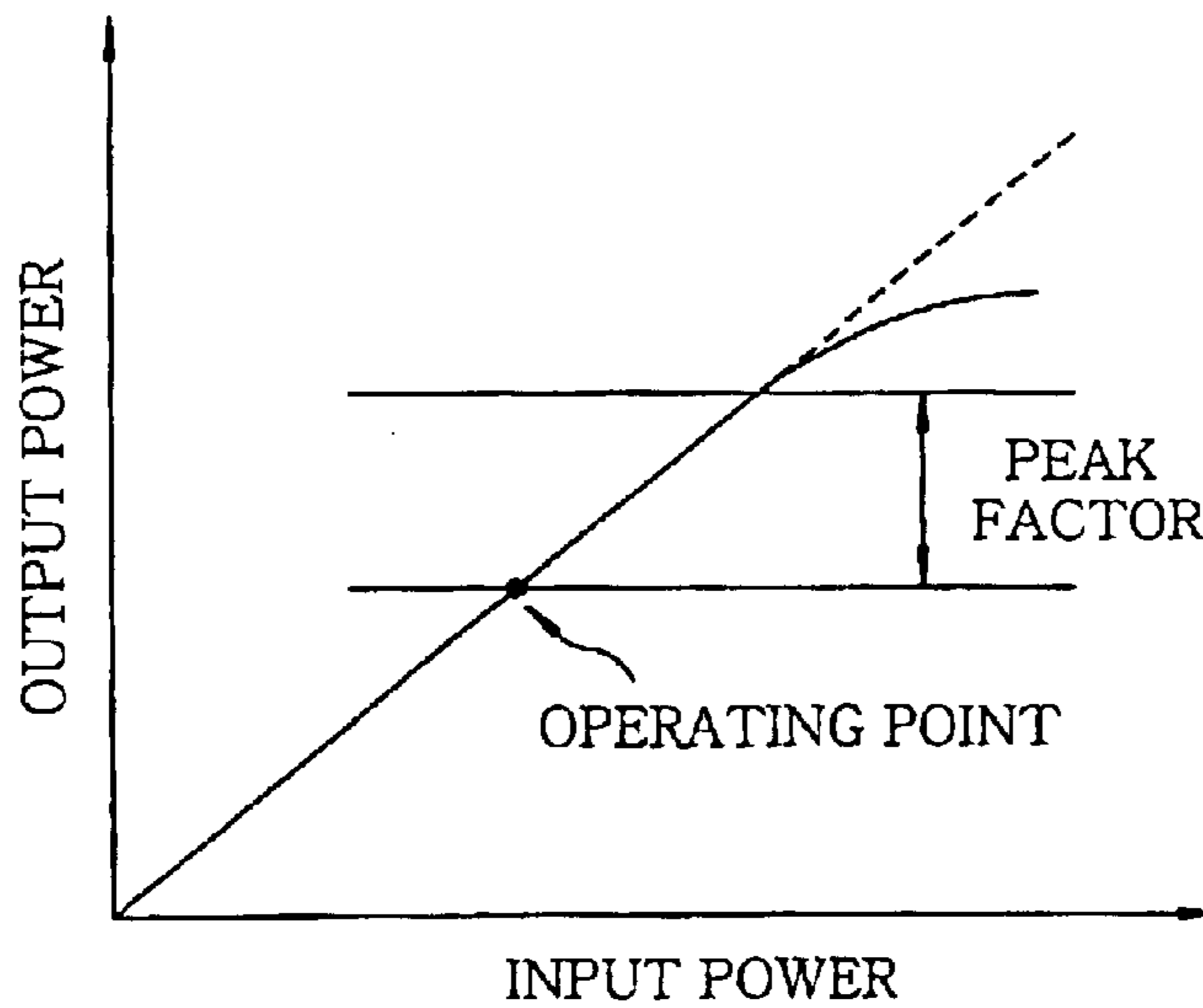
BACK OFF METHOD
