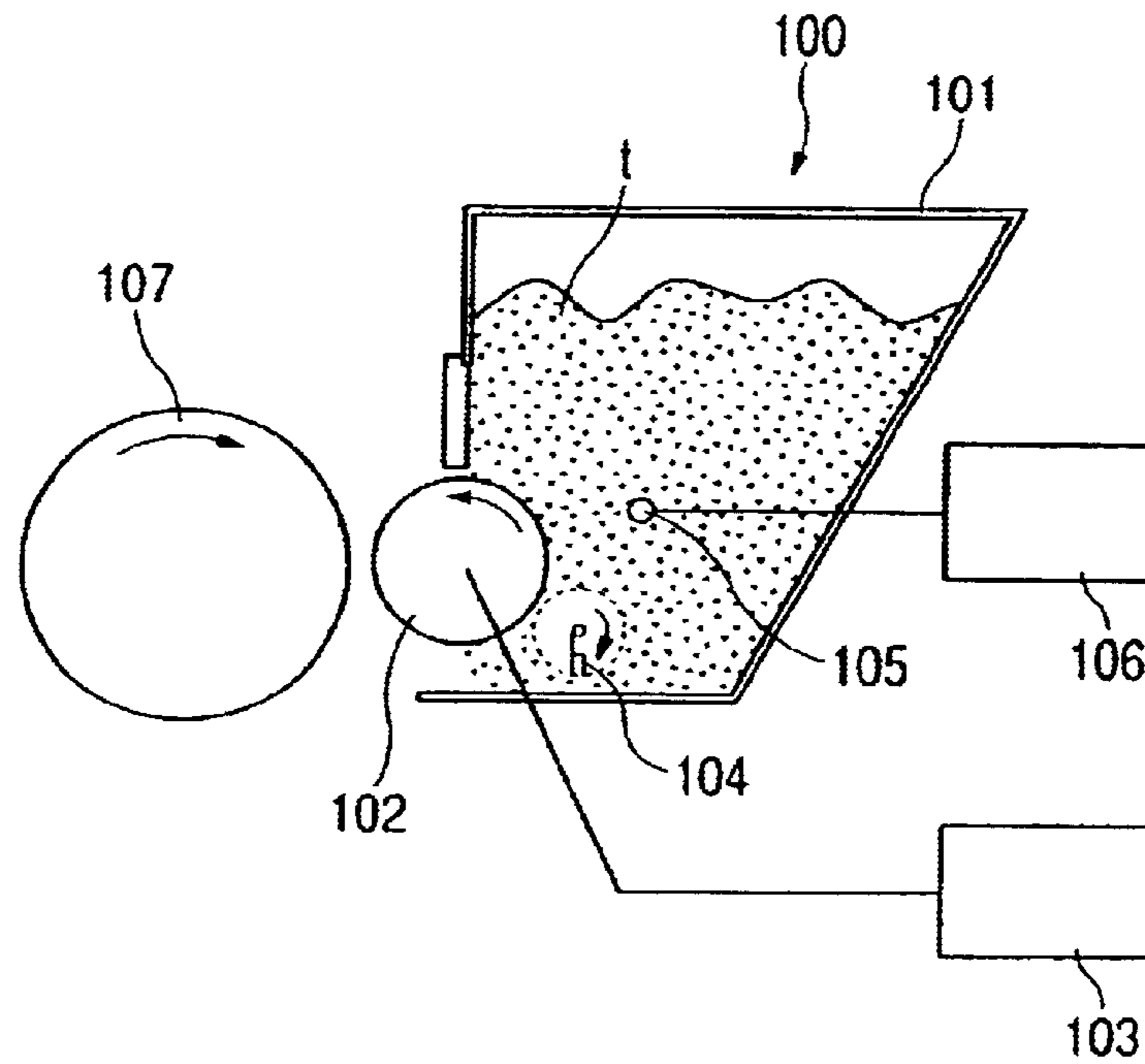
FIG. 6 PRIOR ART
