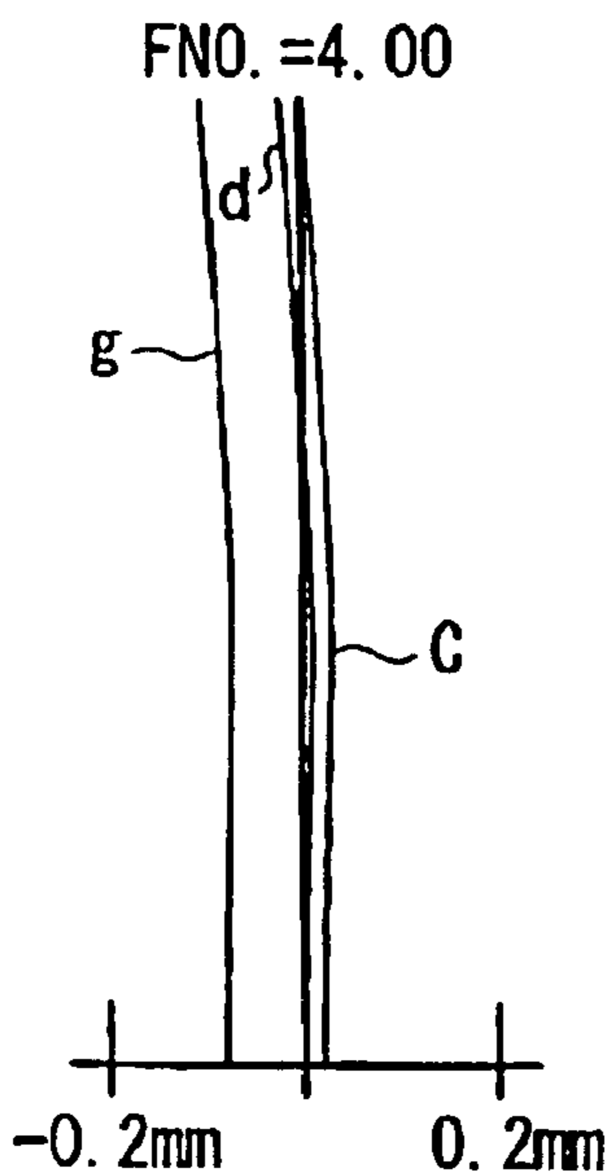
Spherical Aberration Fig. 5A
