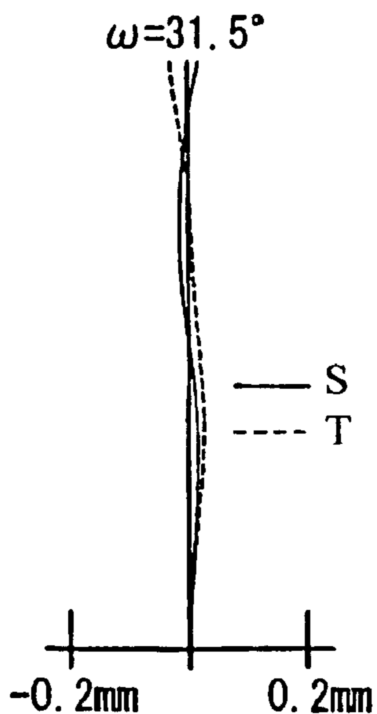
Astigmatism Fig. 5B
