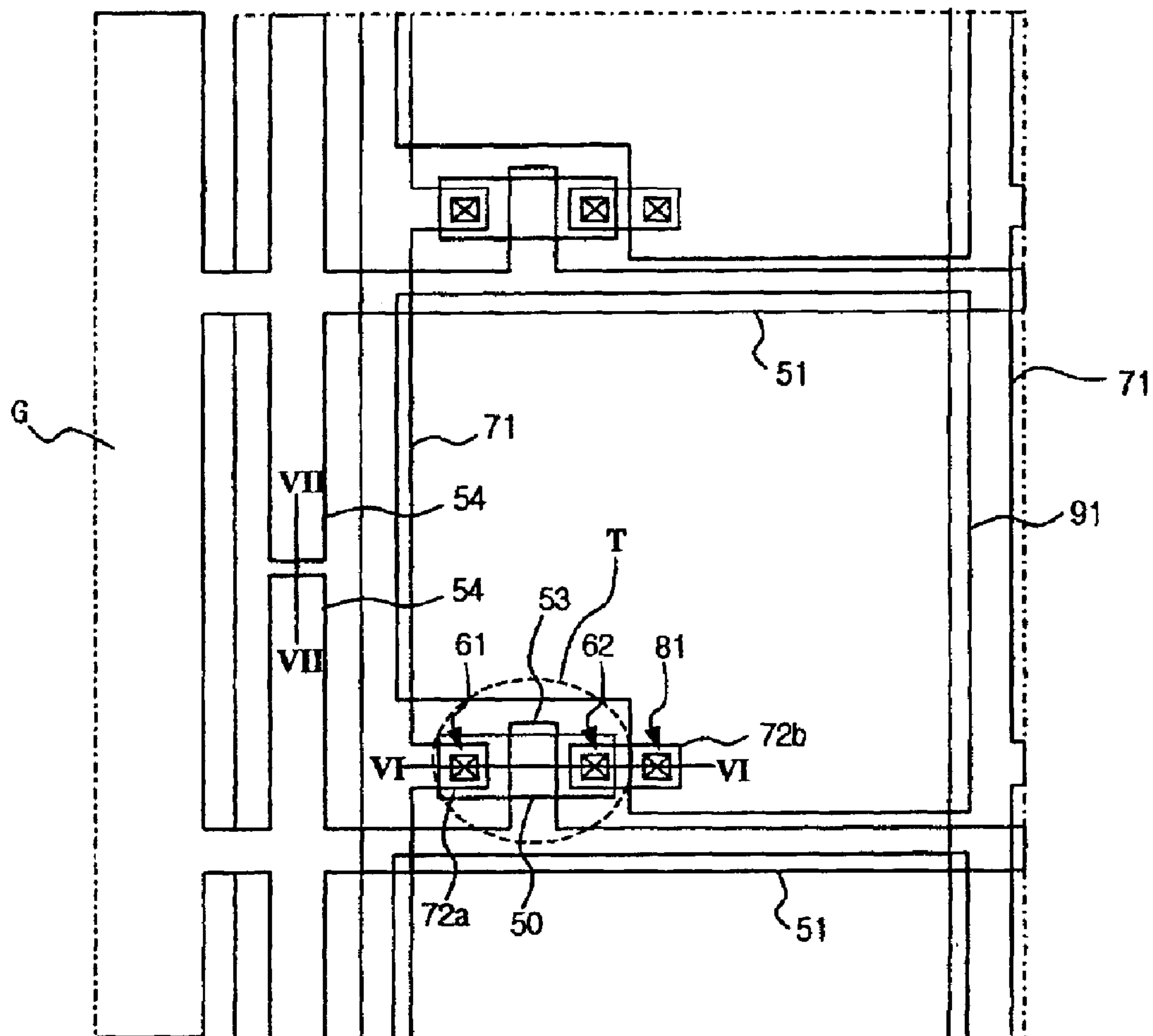
FIG. 5 (RELATED ART)
