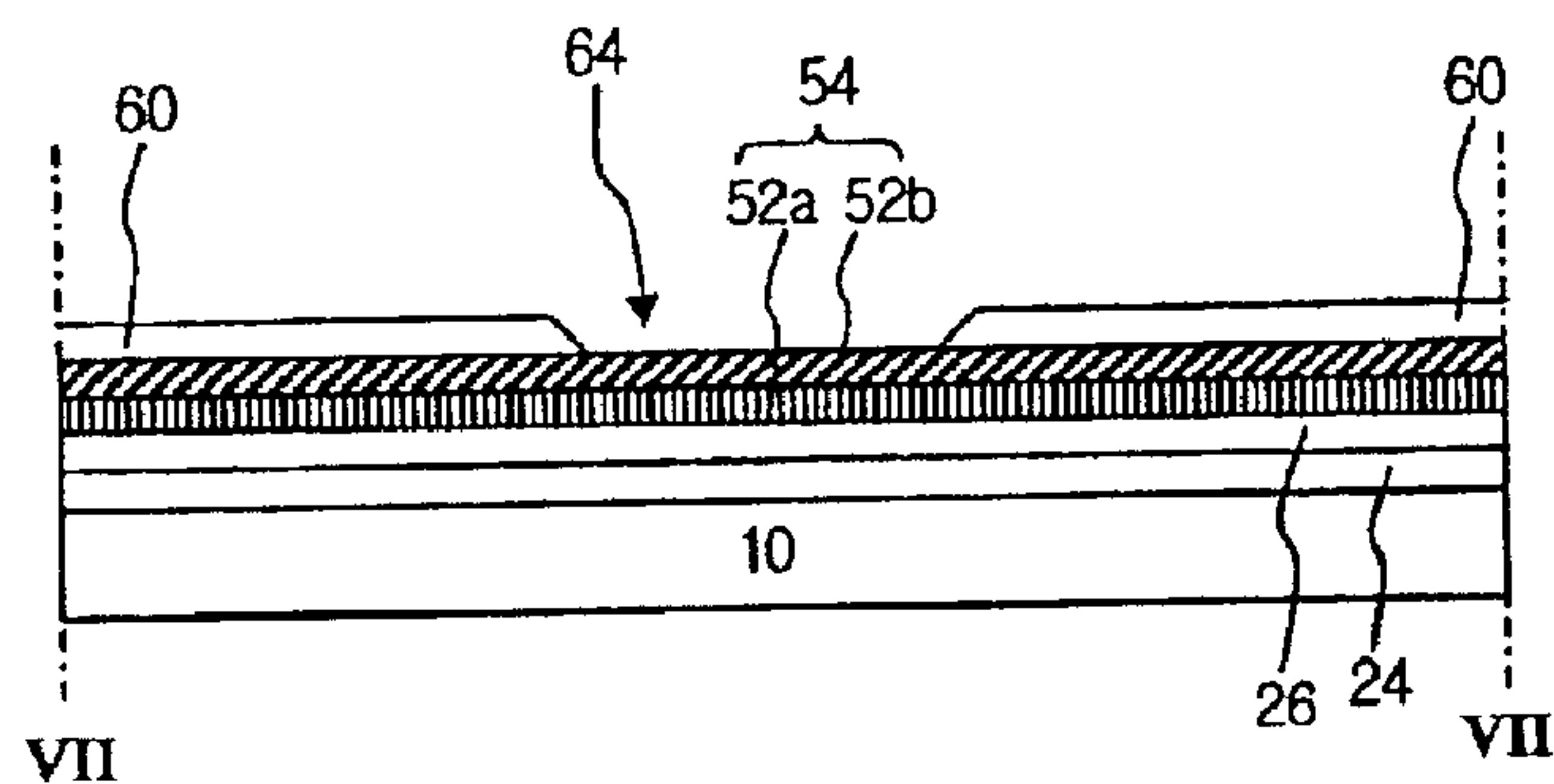
FIG. 7C (RELAED ART)
