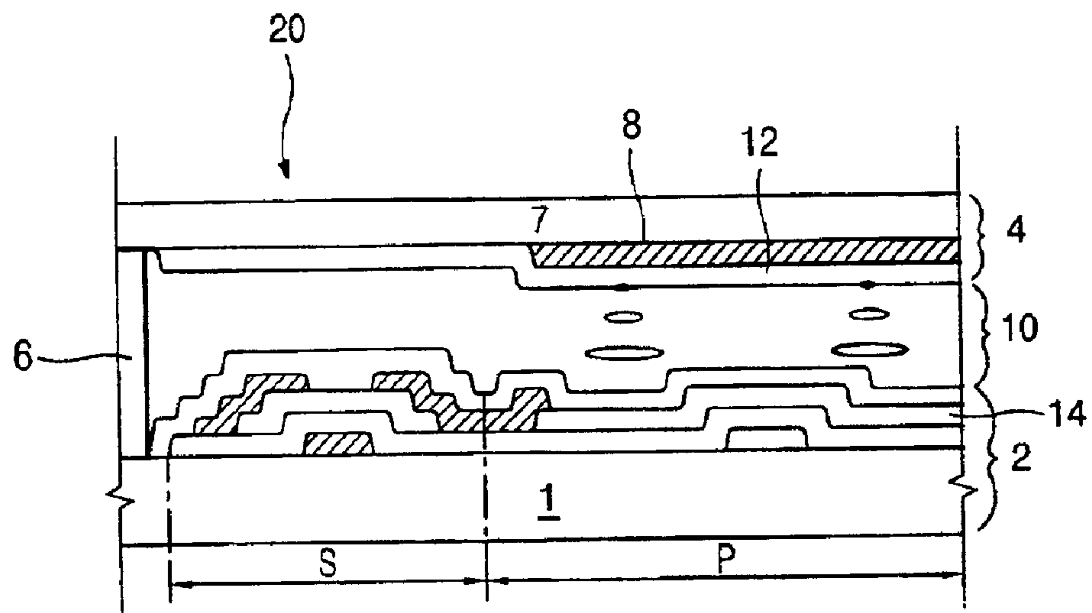
FIG. 2 (RELATED ART)
