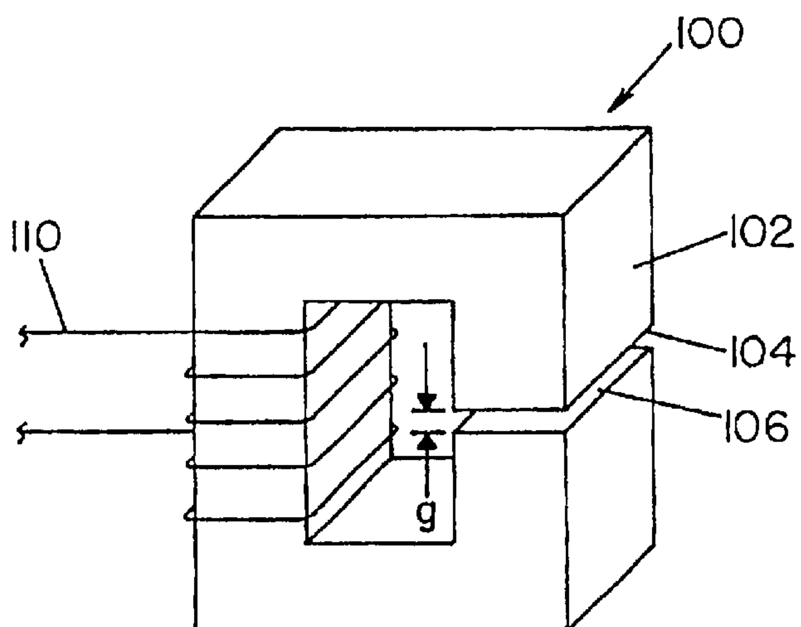
FIG. 2 (PRIOR ART)
