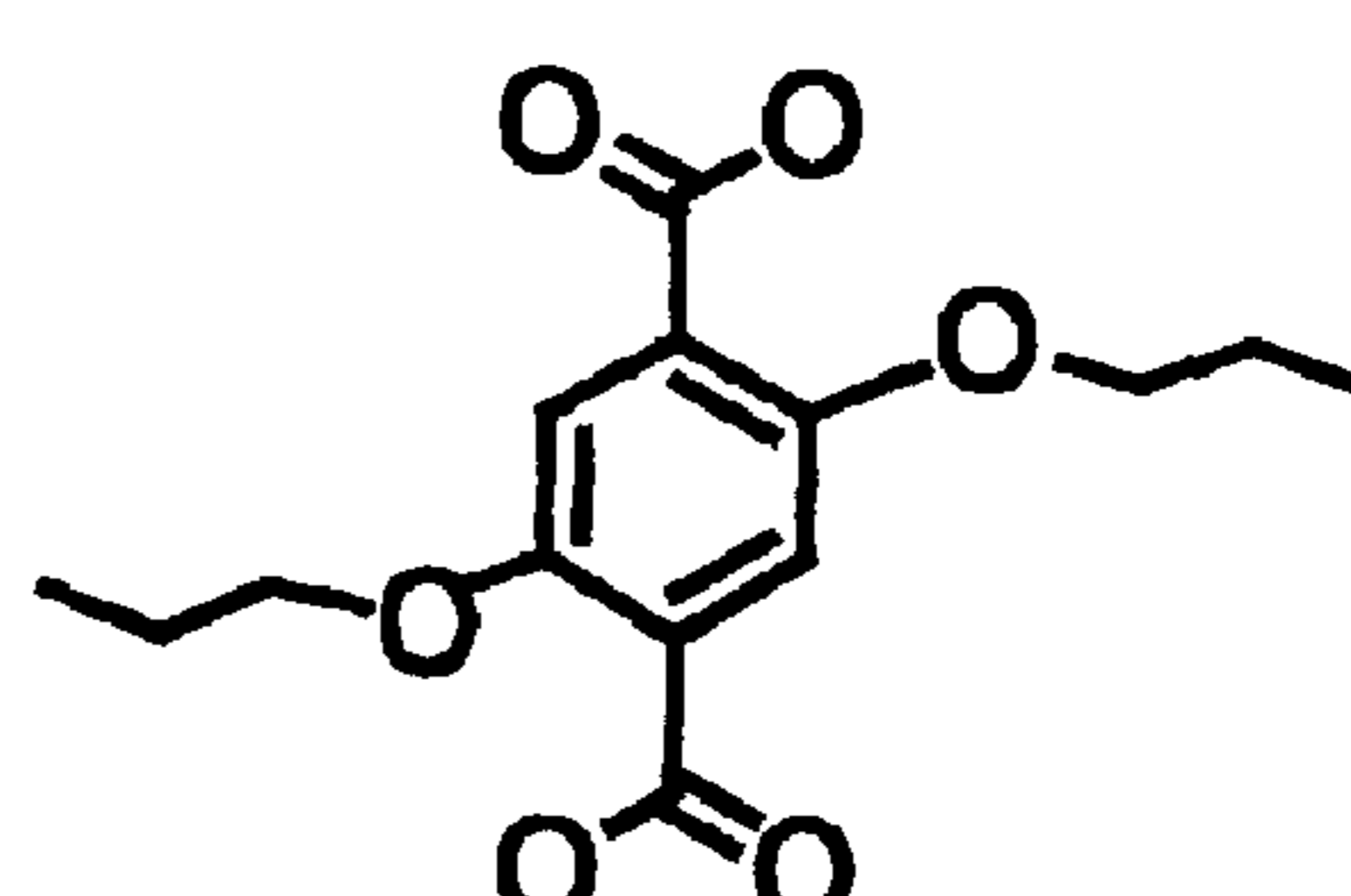
R 4 -BDC
