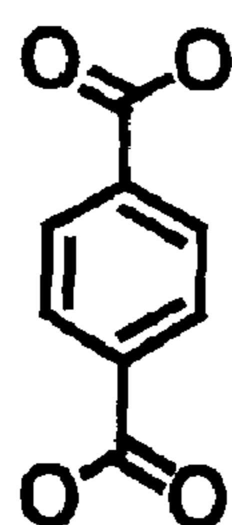
R 1 -BDC
