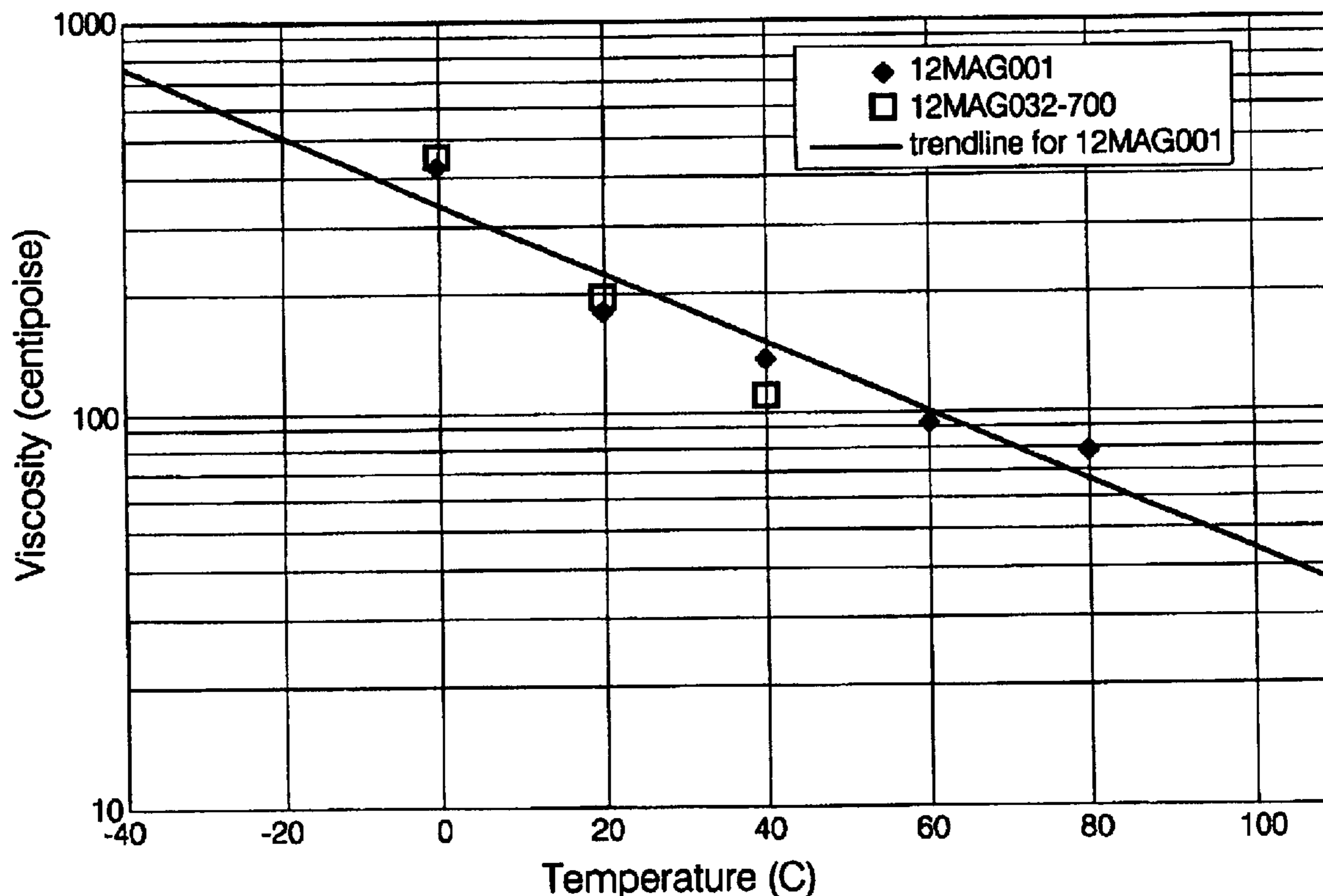
Viscosity versus Temperature for 12MAG001
