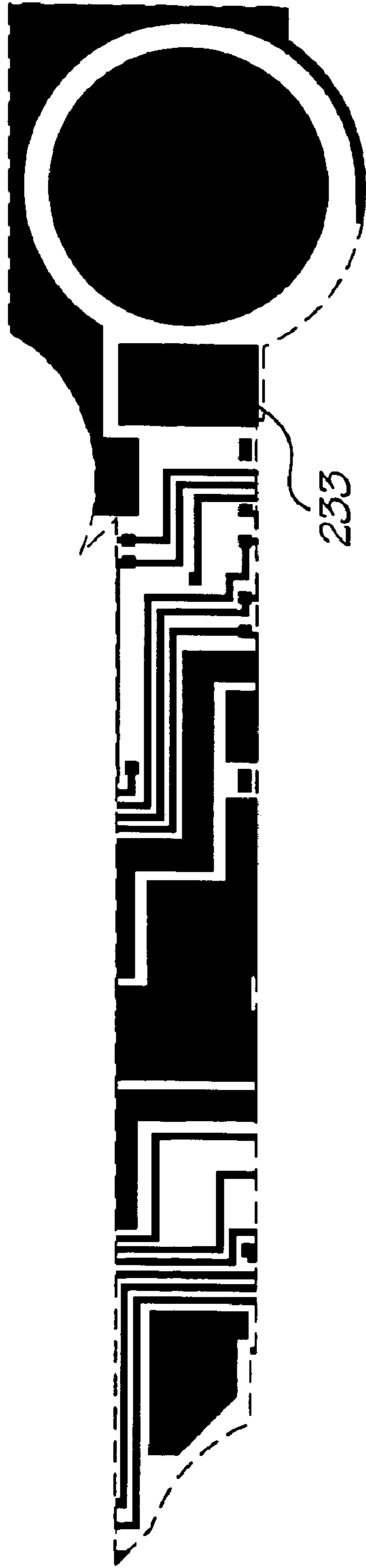
Metal 2 mask
