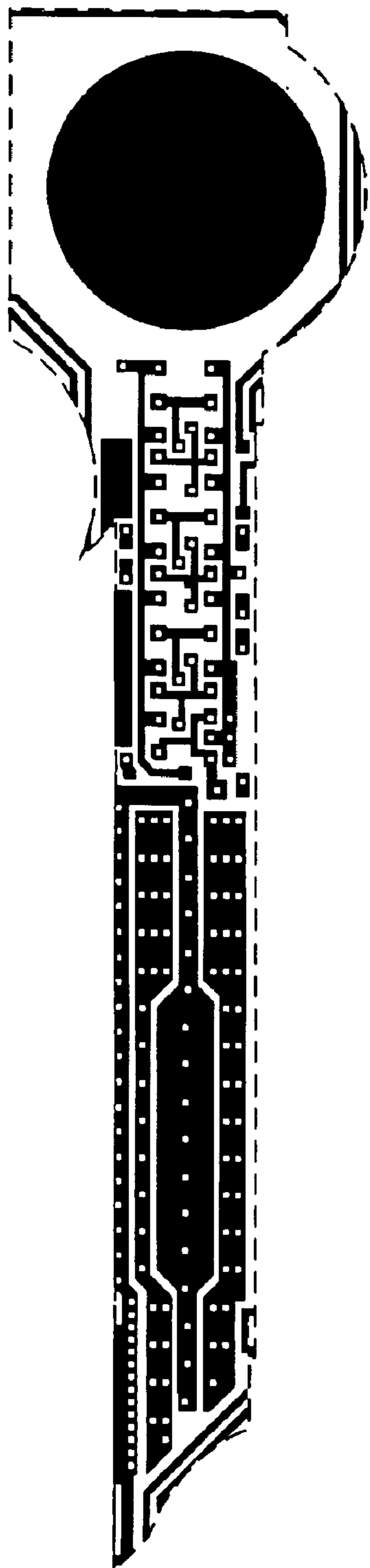
Metal 1 mask
