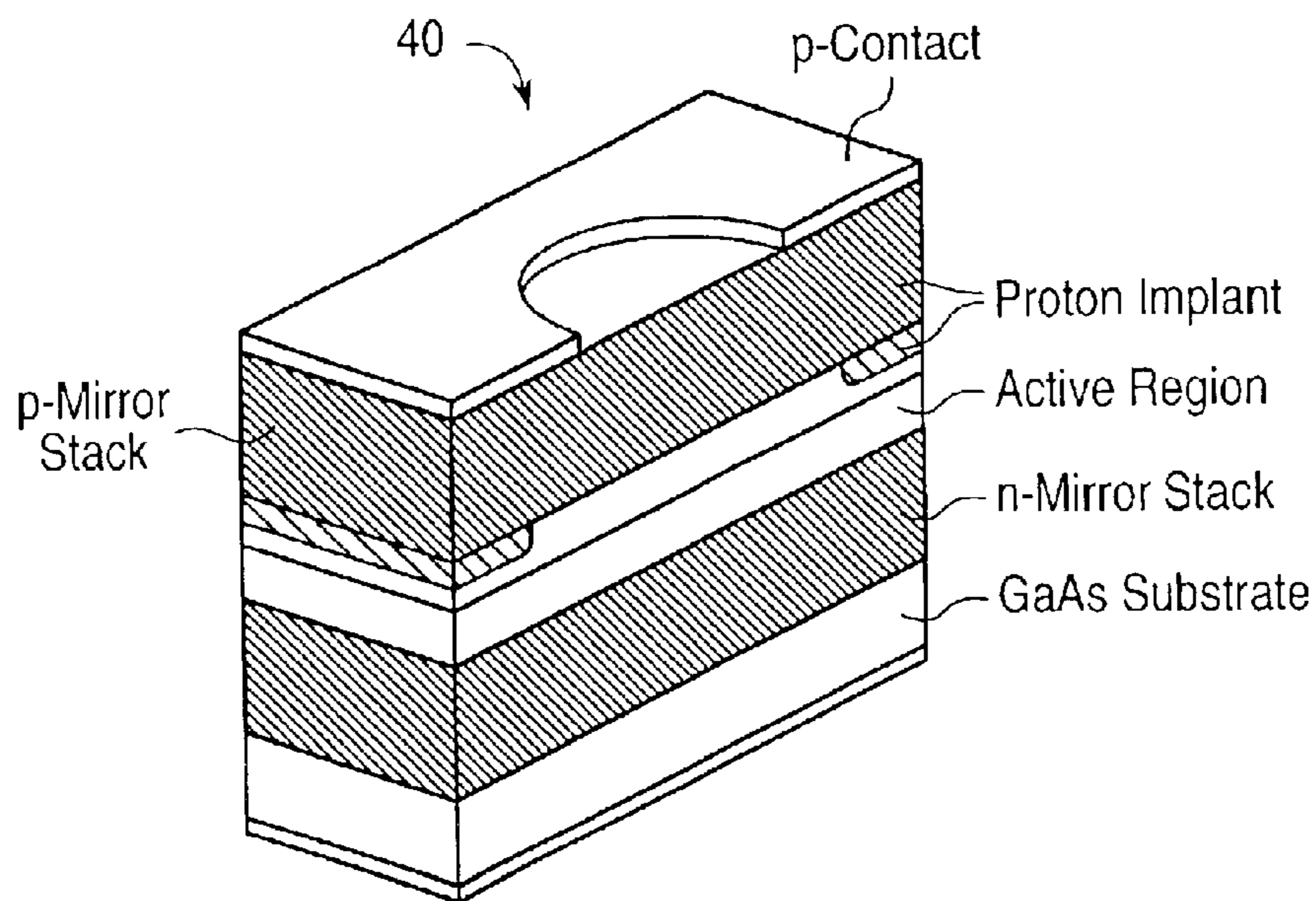
FIG. 4 (Prior Art)
