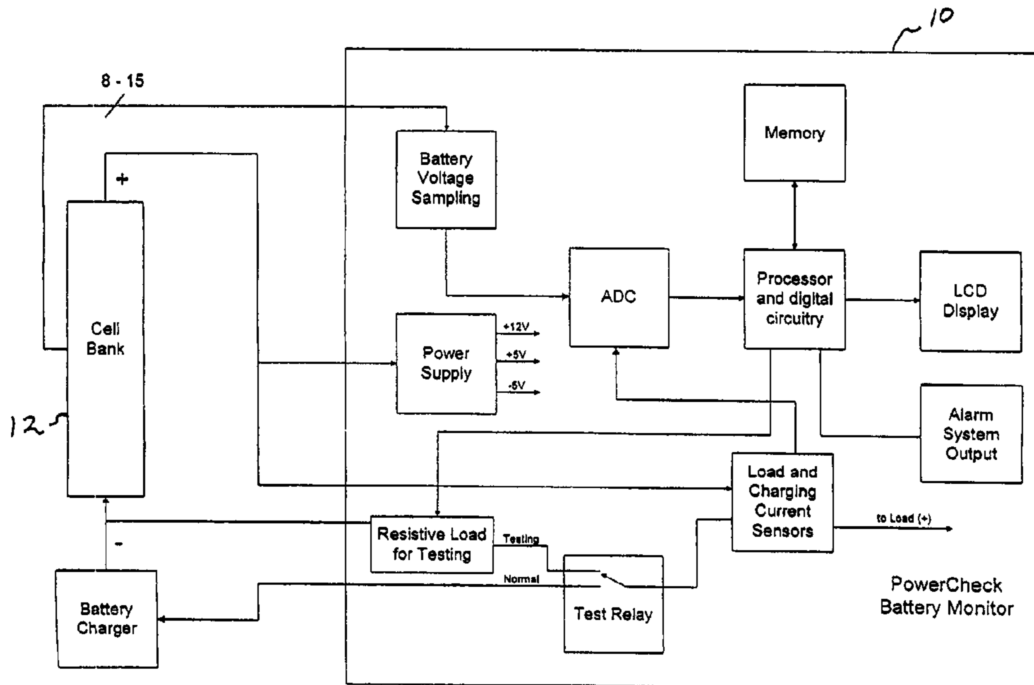
Block Diagram for PowerCheck Battery Monitoring System
