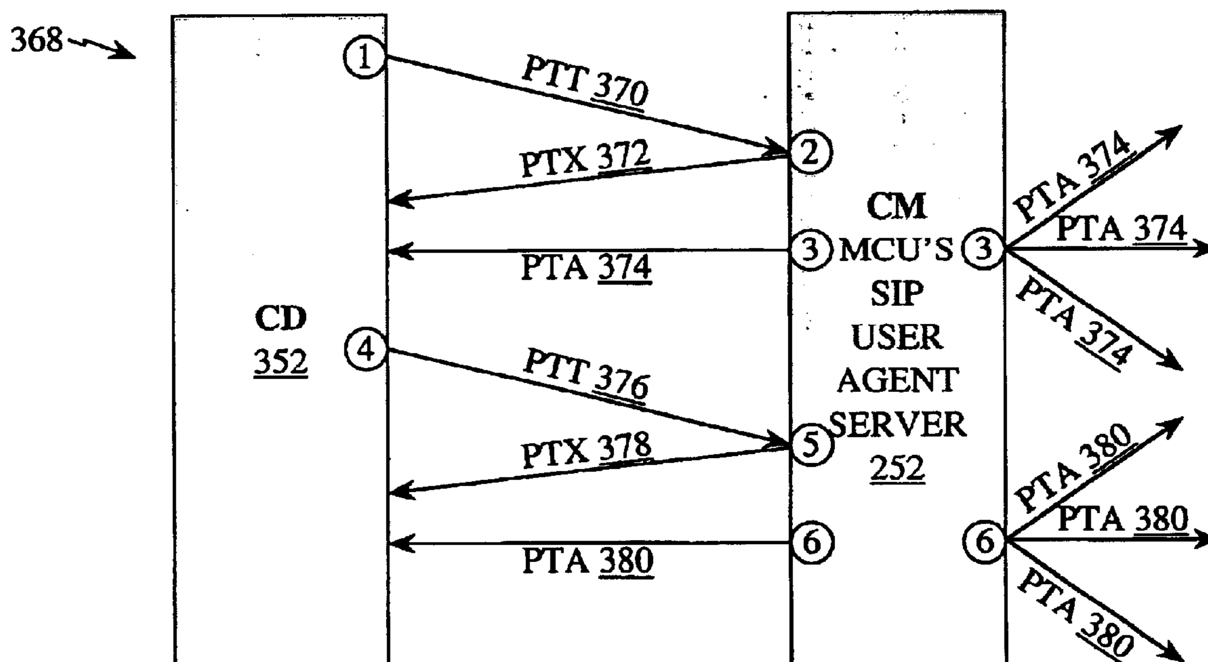
FIG. 12: MEDIA SIGNALING MESSAGE SEQUENCE (PTT)
