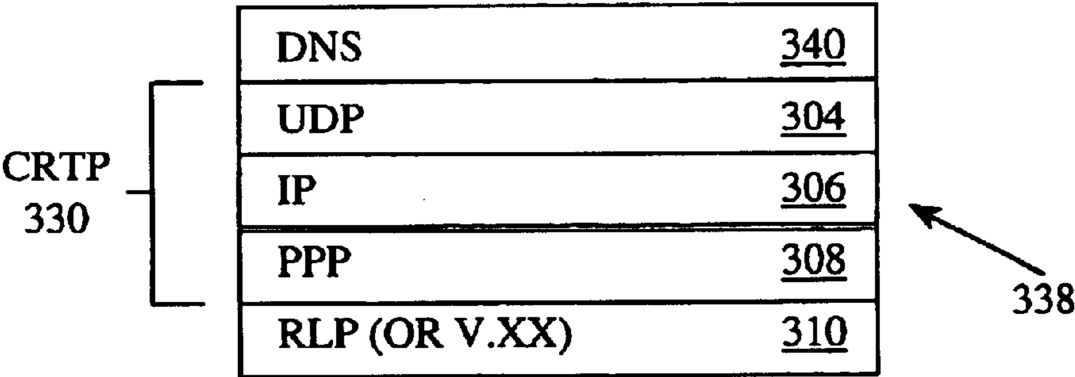
FIG. 9: DNS CLIENT PROTOCOL STACK
