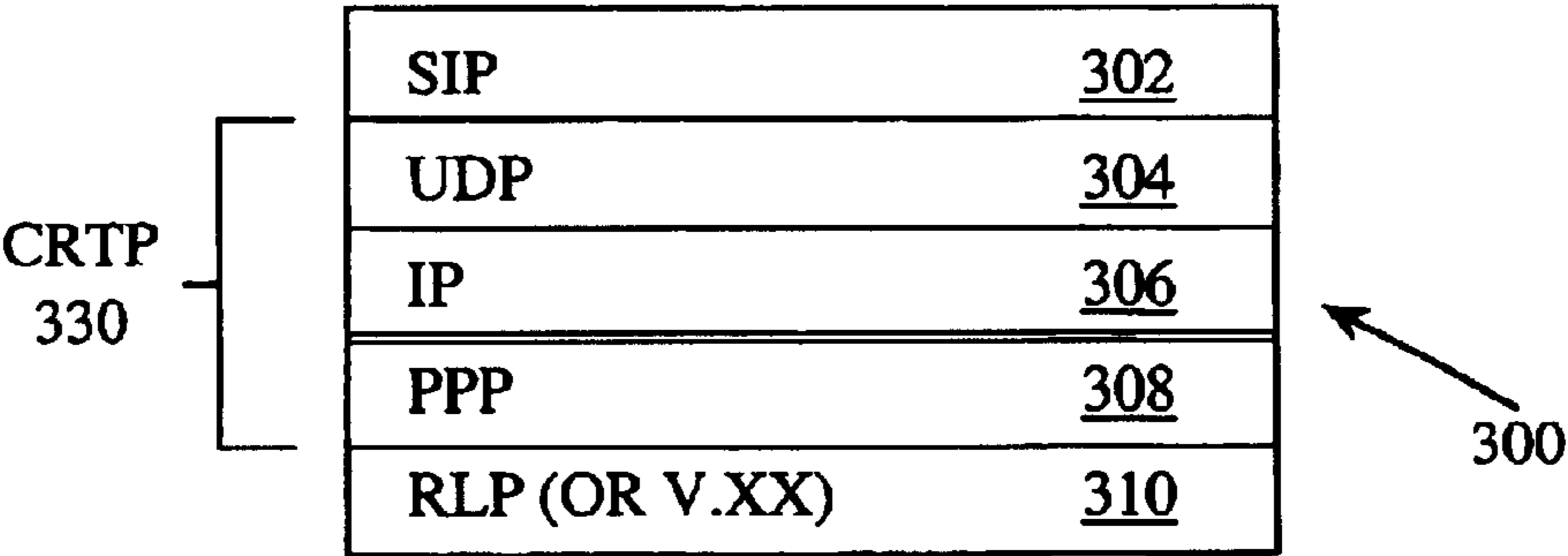
FIG. 4: NBS SIP SIGNALING PROTOCOL STACK
