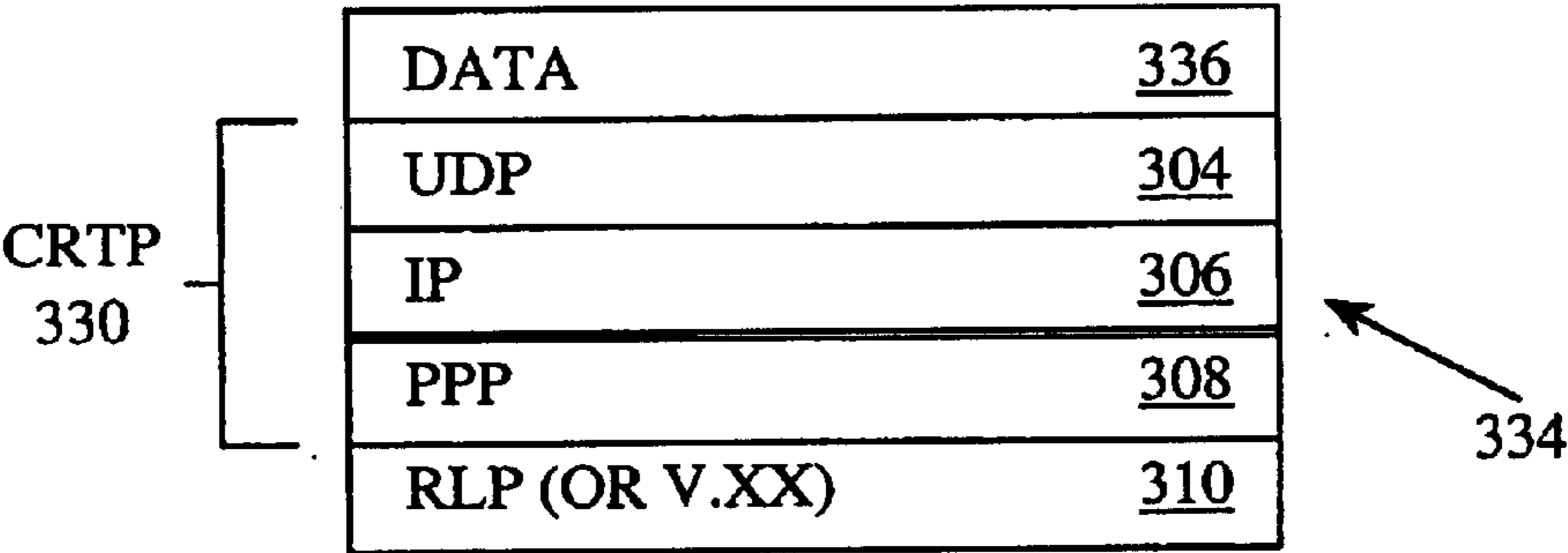
FIG. 8: MEDIA TRAFFIC (DATA) PROTOCOL STACK
