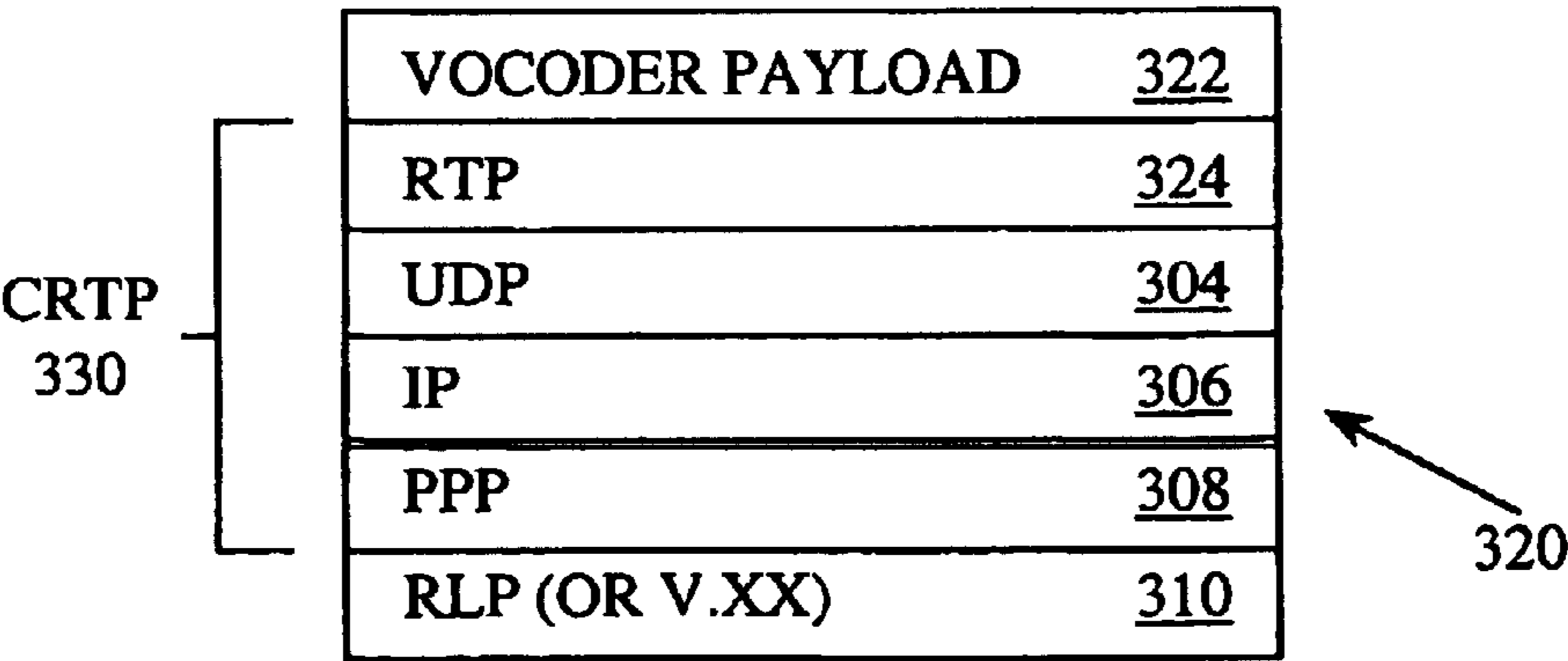
FIG. 6: RTP VOICE MEDIA PROTOCOL STACK
