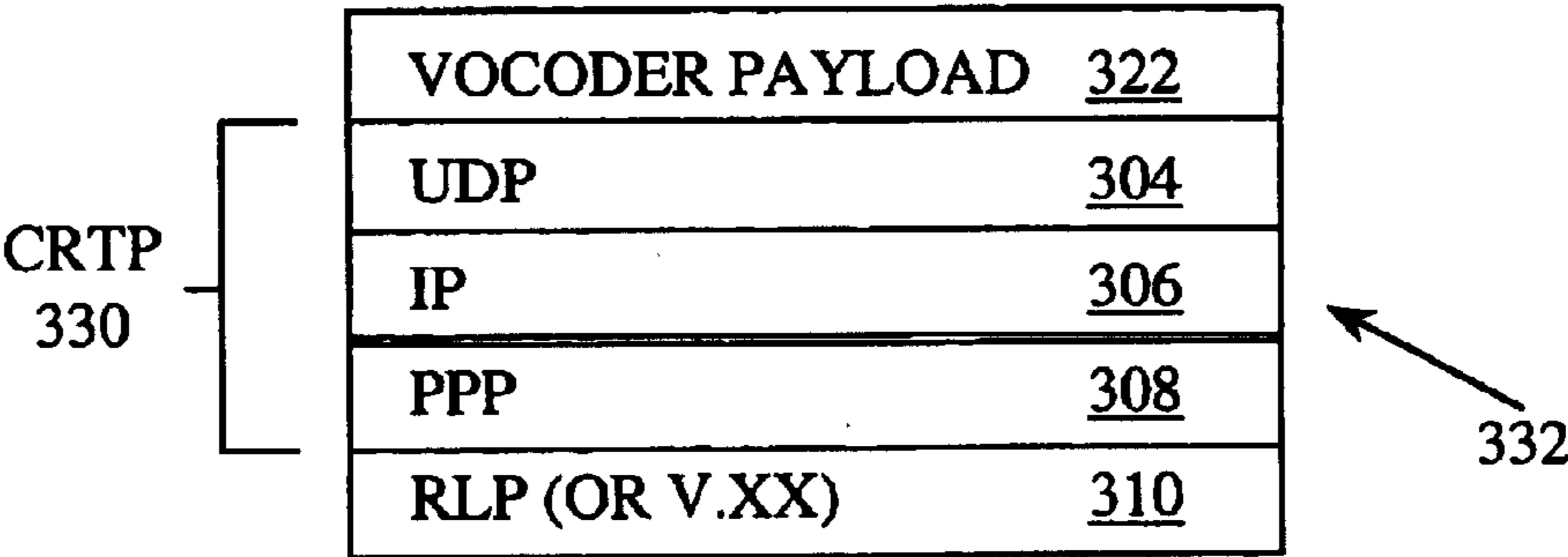
FIG. 7: UDP VOICE MEDIA PROTOCOL STACK
