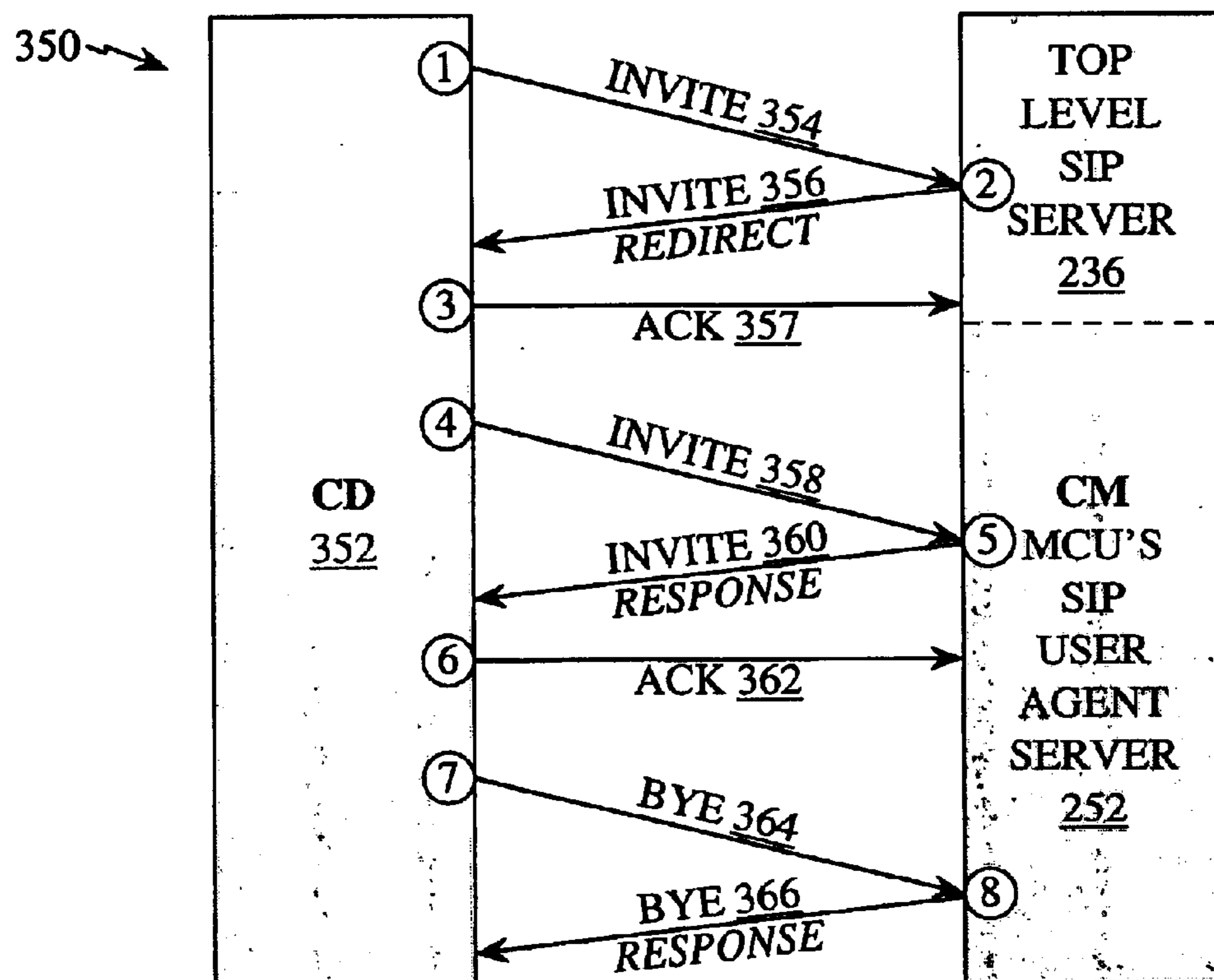
FIG. 11: SIP CALL SIGNALING
