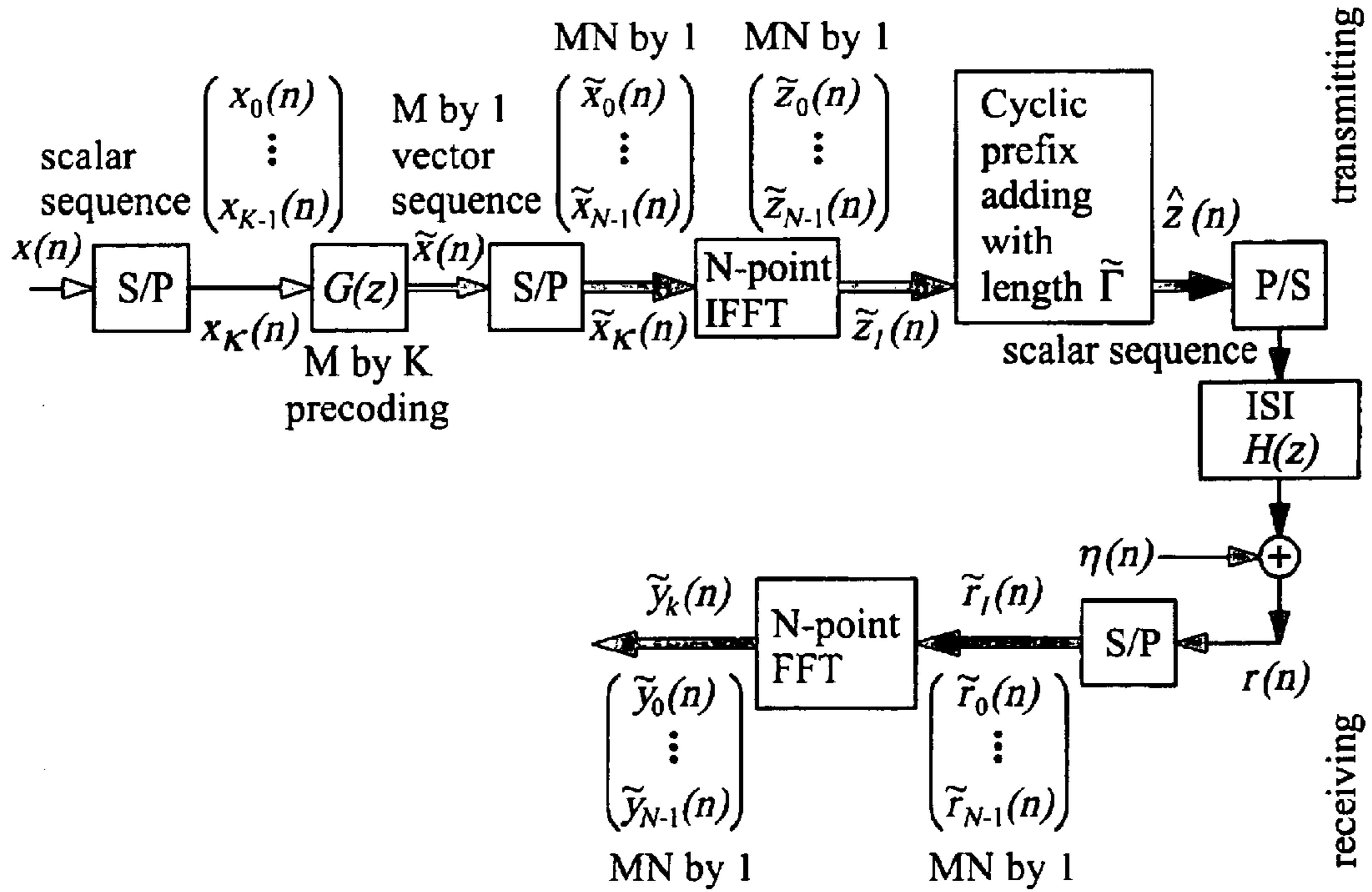
Precoded OFDM system.
