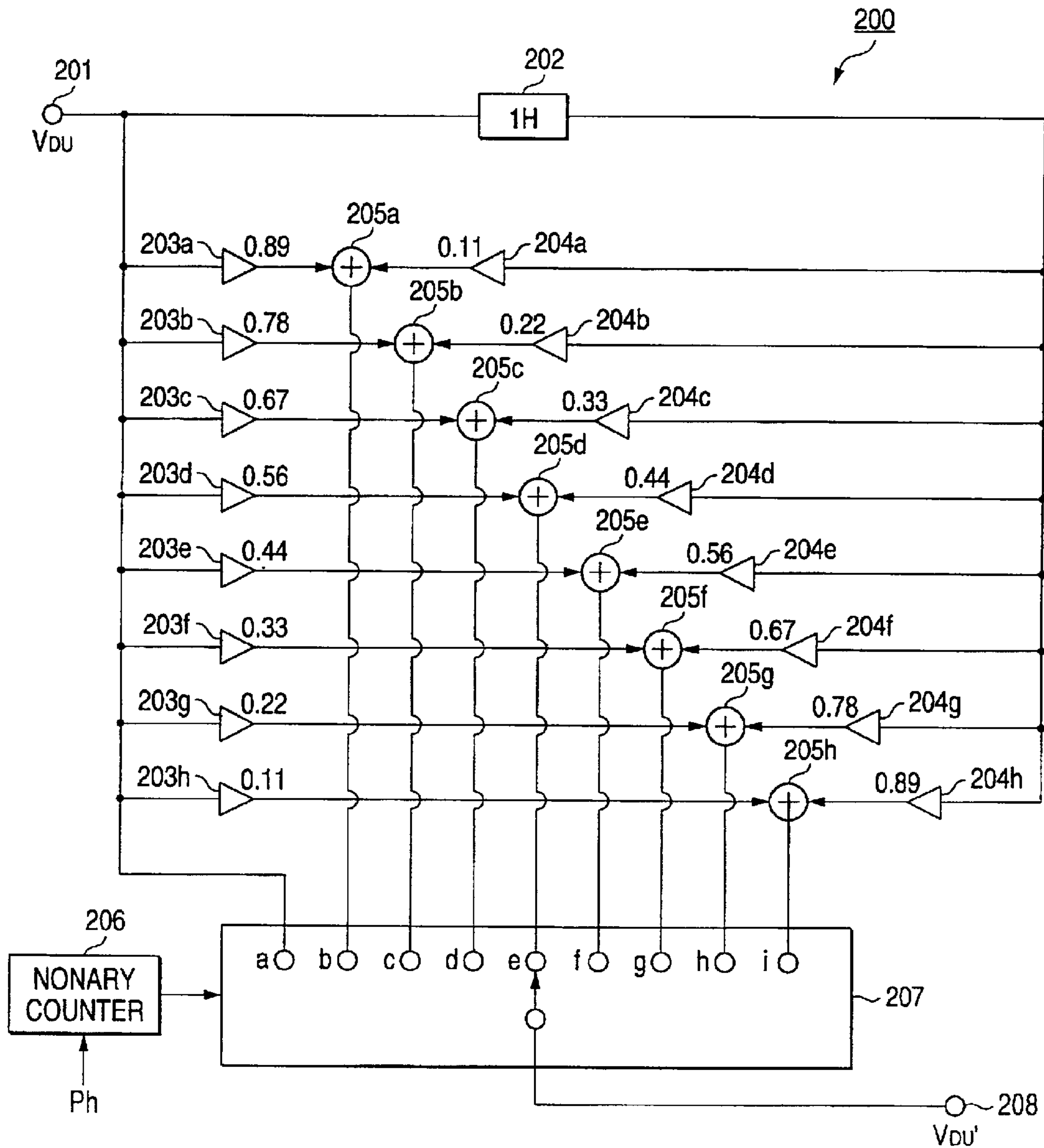
FIG. 13 PRIOR ART
