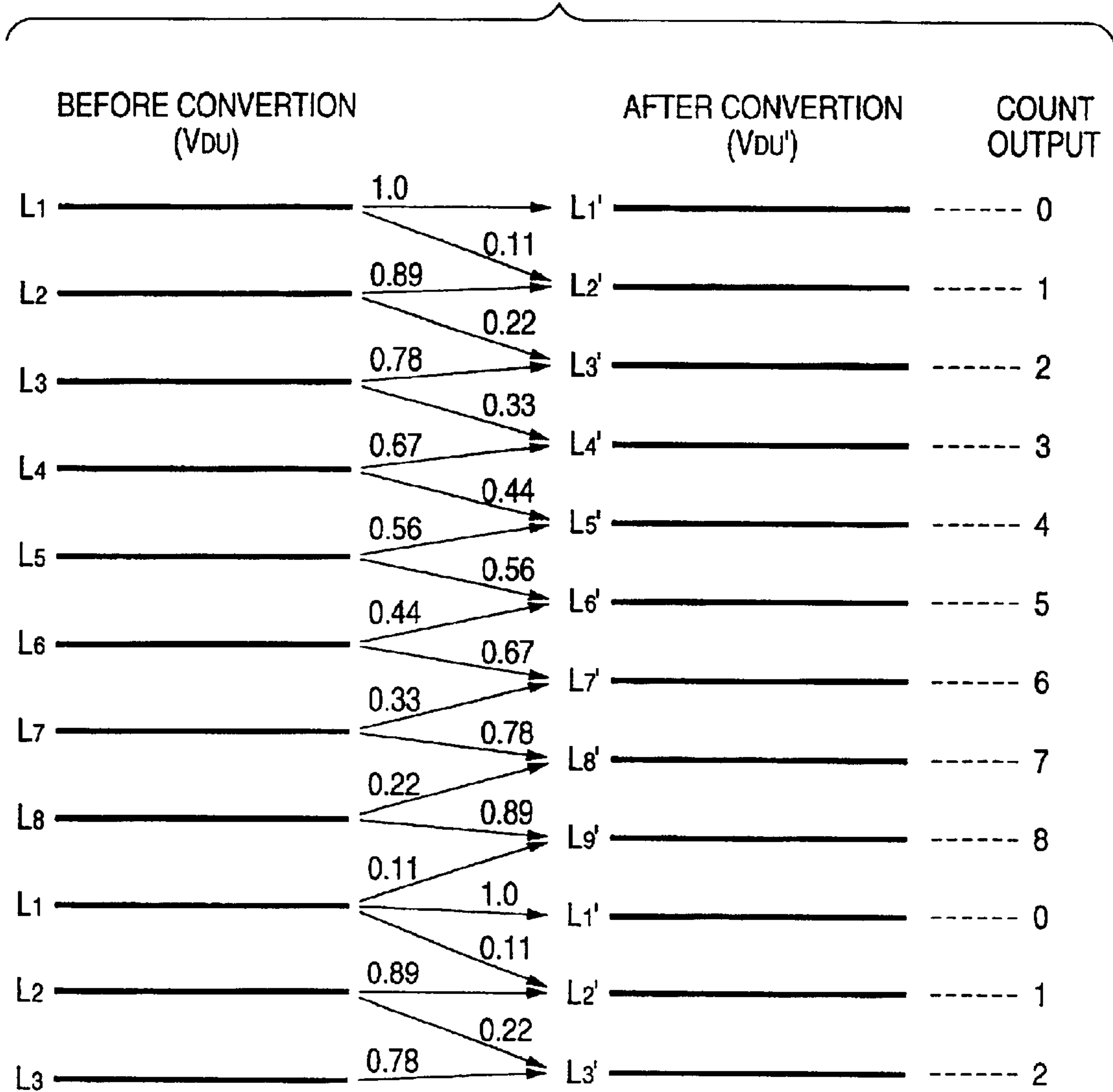
FIG. 14 PRIOR ART
