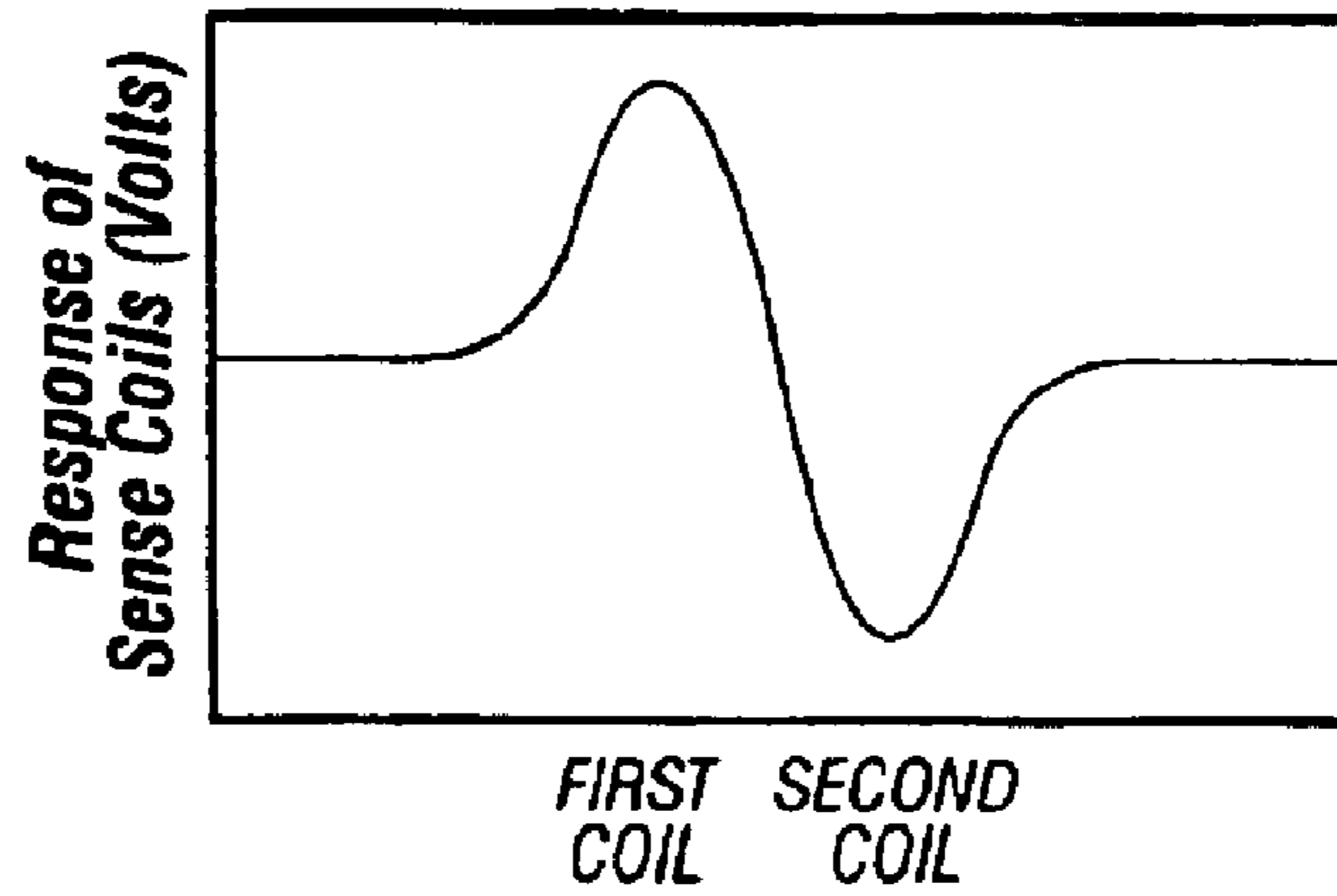
Position of Spot with Respect to Sense Coils FIG. 6
