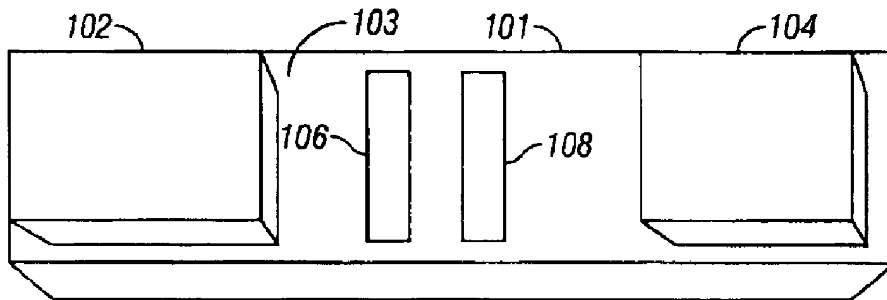
Position of Spot with Respect to Sense Coils FIG. 6
