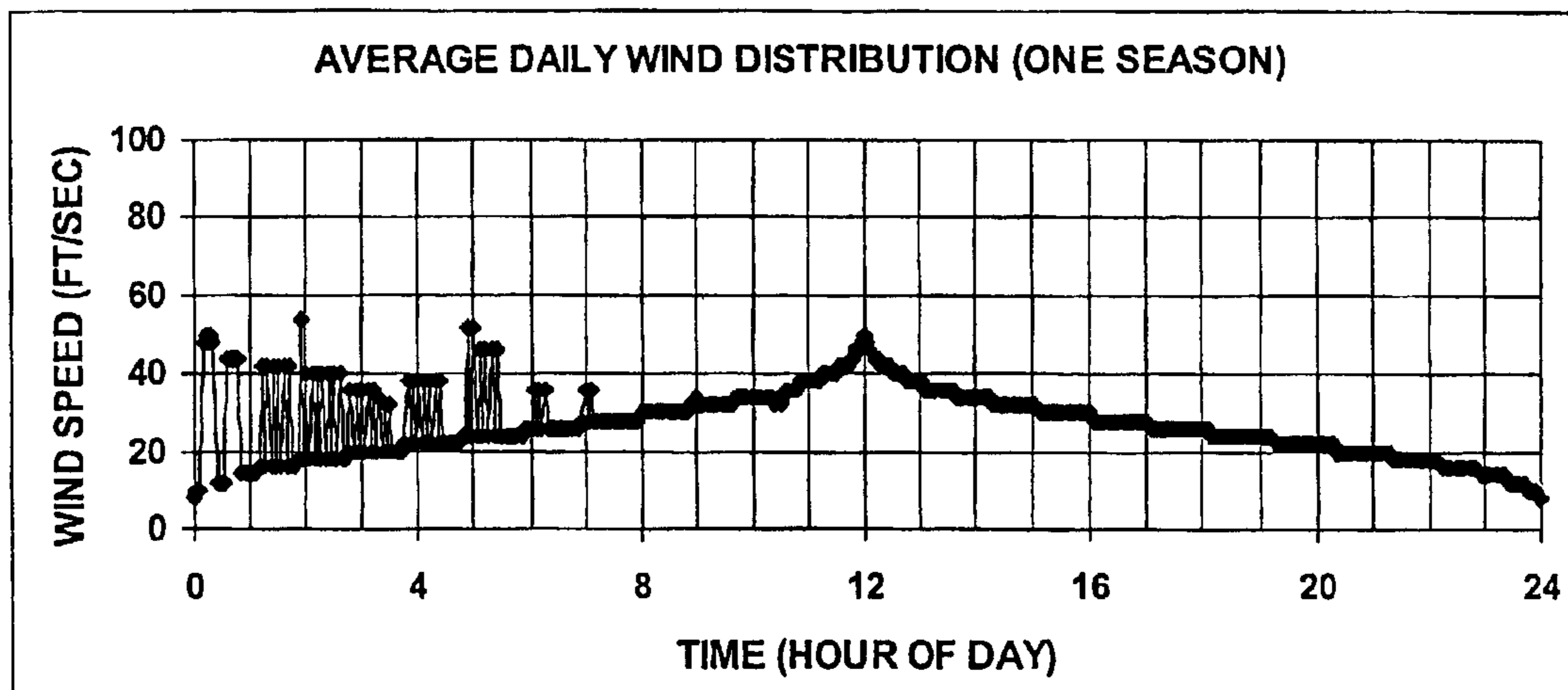
Figure 7. Example Wind History for Windy Site during One Season (CASE A)
