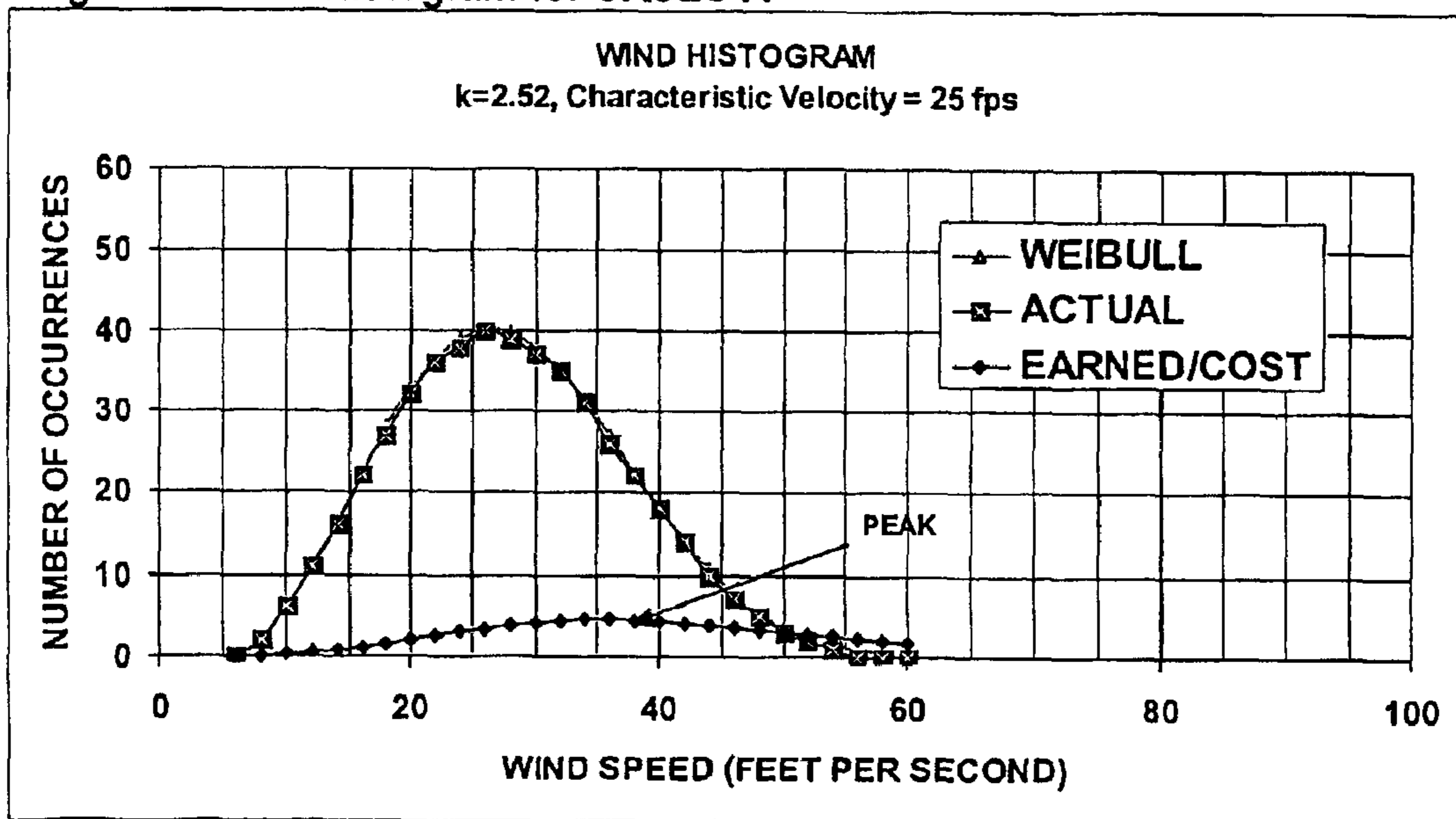
Figure 5. Wind Histogram for CASES A
