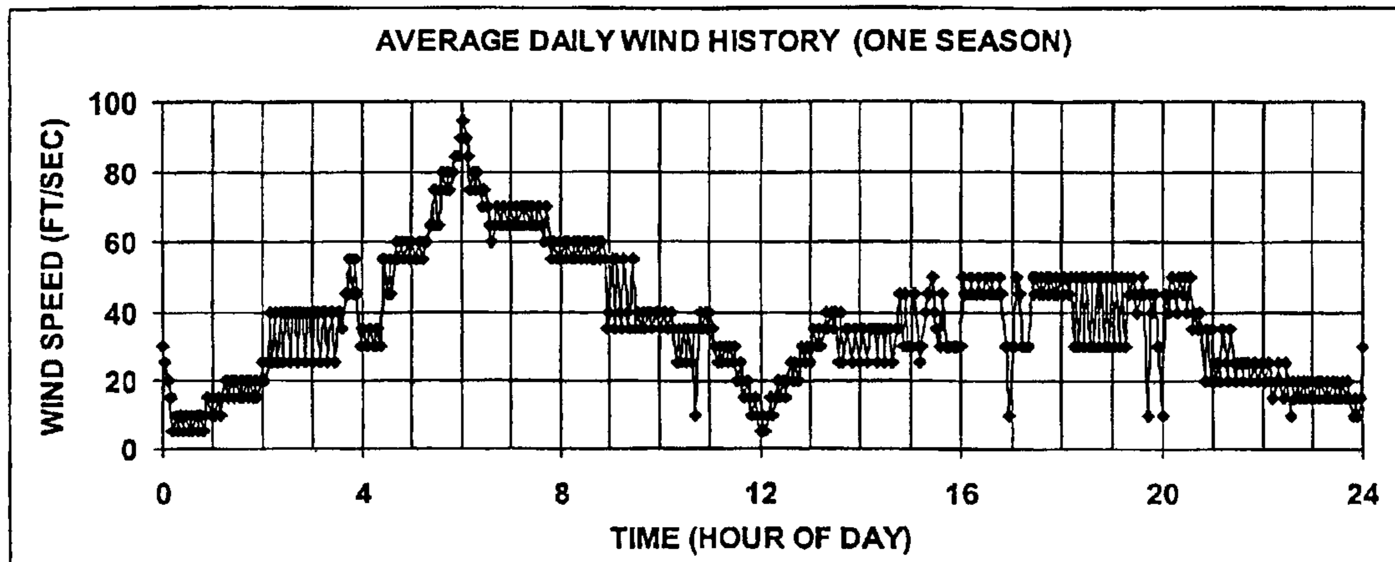
Figure 7. Example Wind History for Windy Site during One Season (CASE A)
