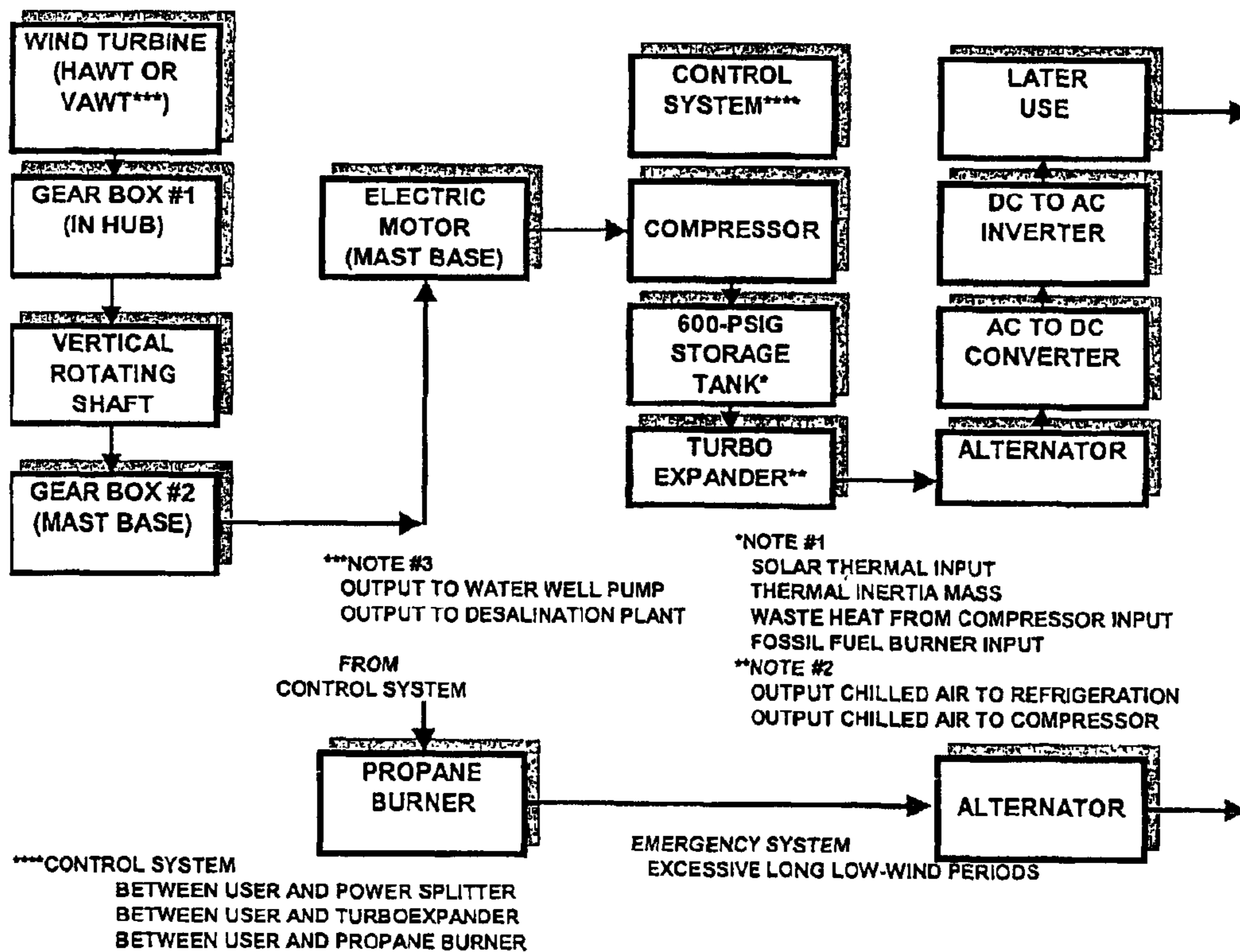
Figure 2. "Modified" HAWT or VAWT System
