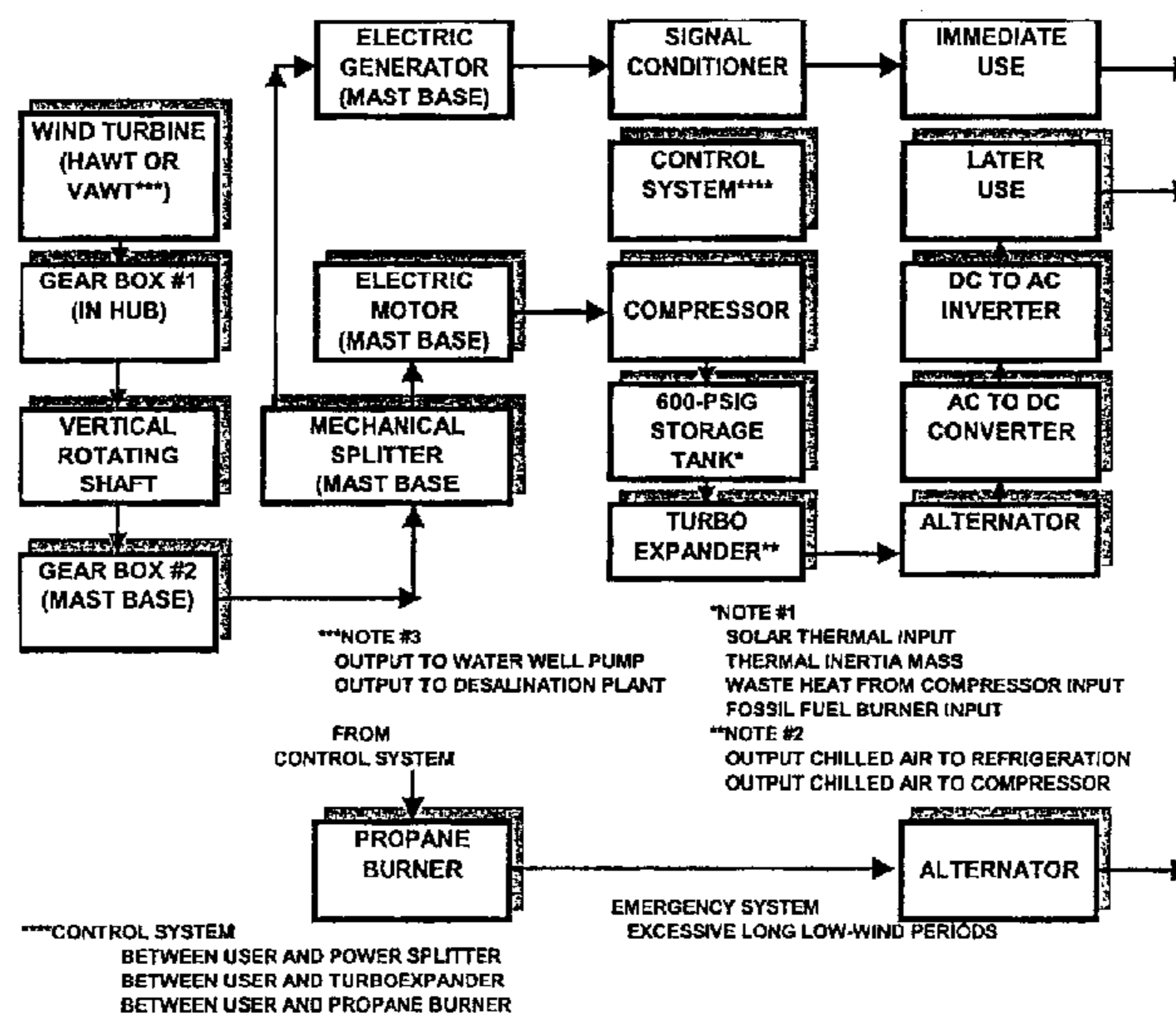
Hybrid Wind Turbine System
