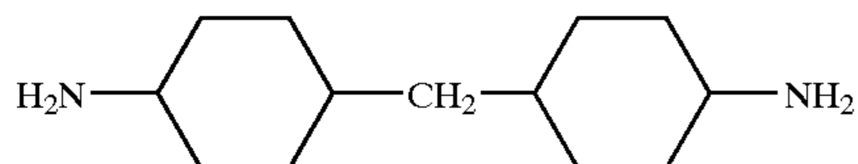
Chemical formula (17)
