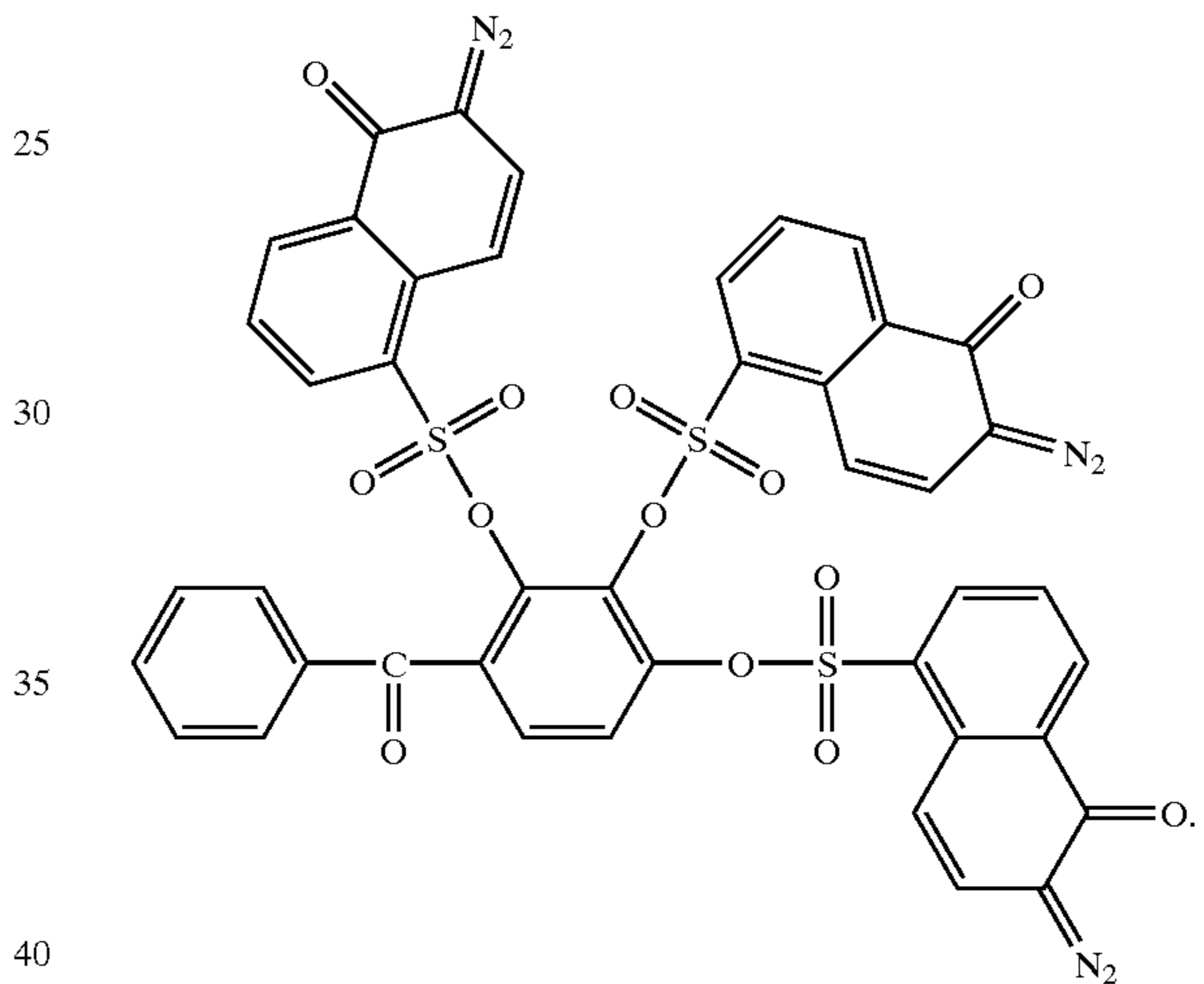
Chemical Formula (15)
