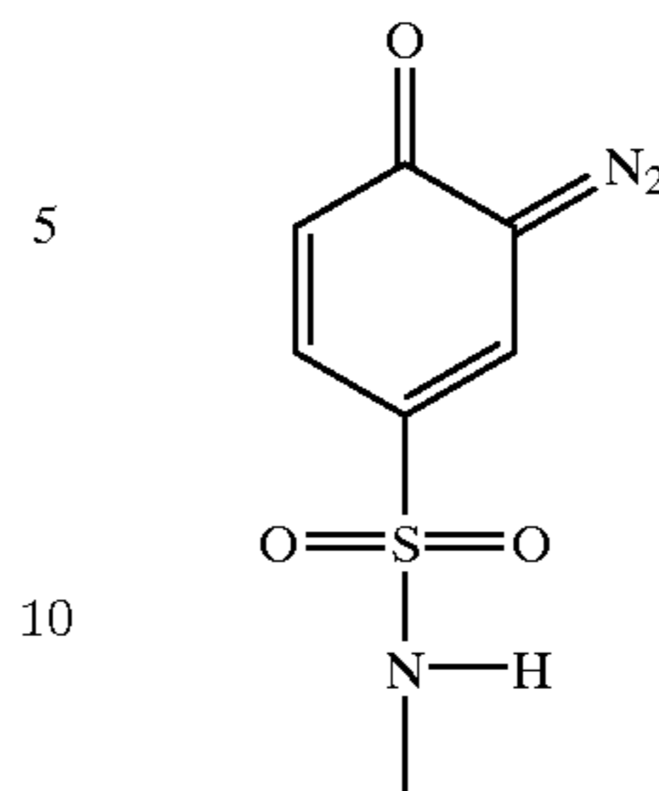
Formula (5)
