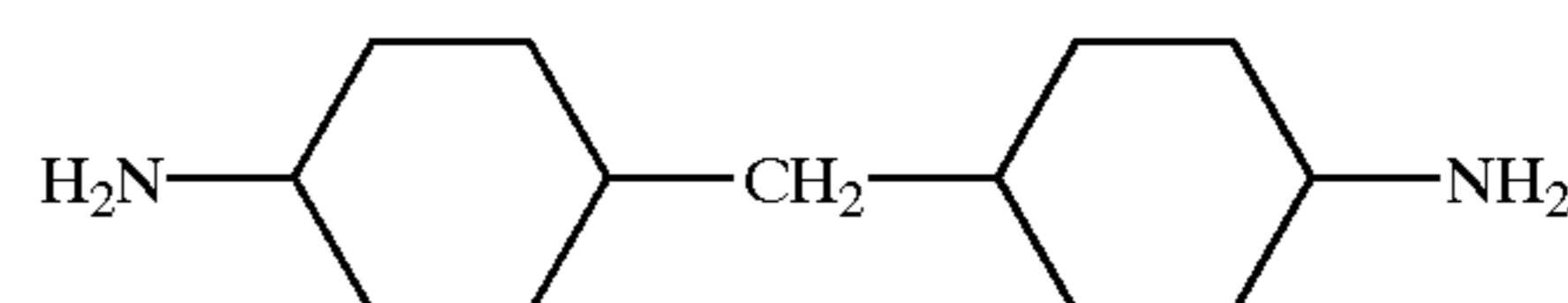
Chemical formula (17)
