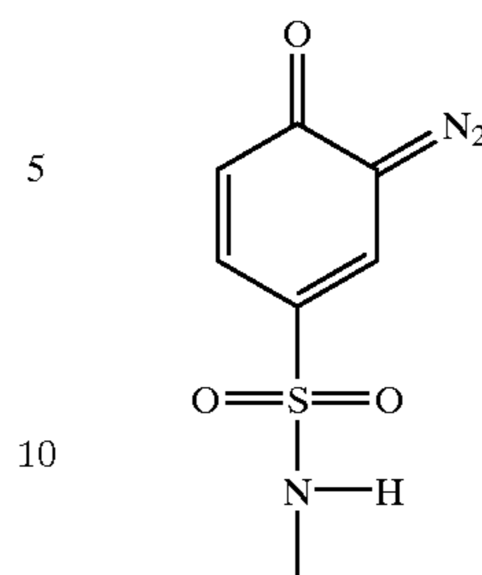
Formula (5)
