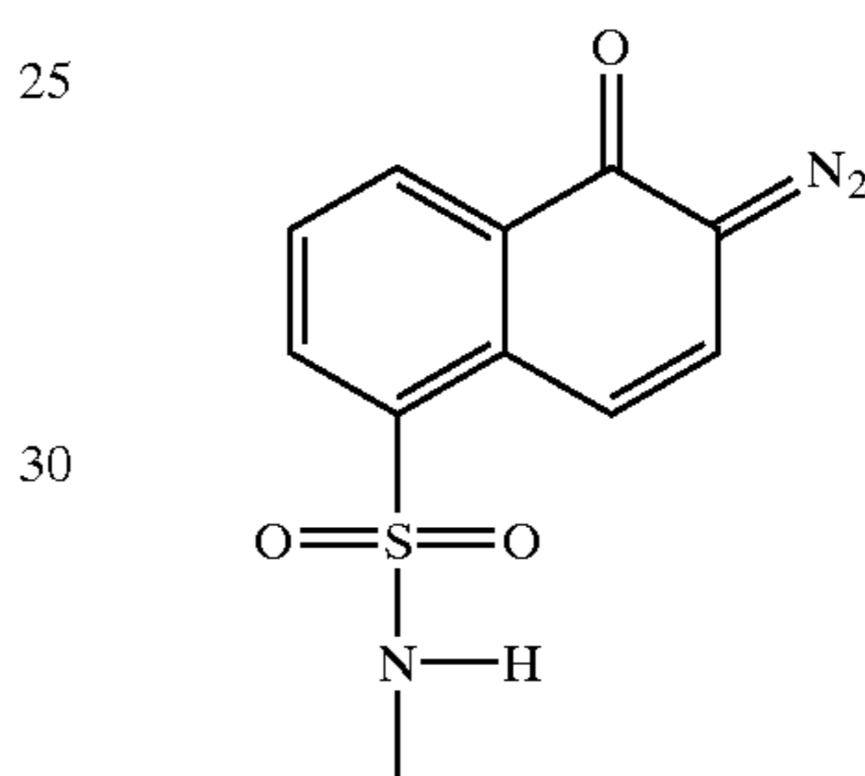
Chemical Formula (6)
