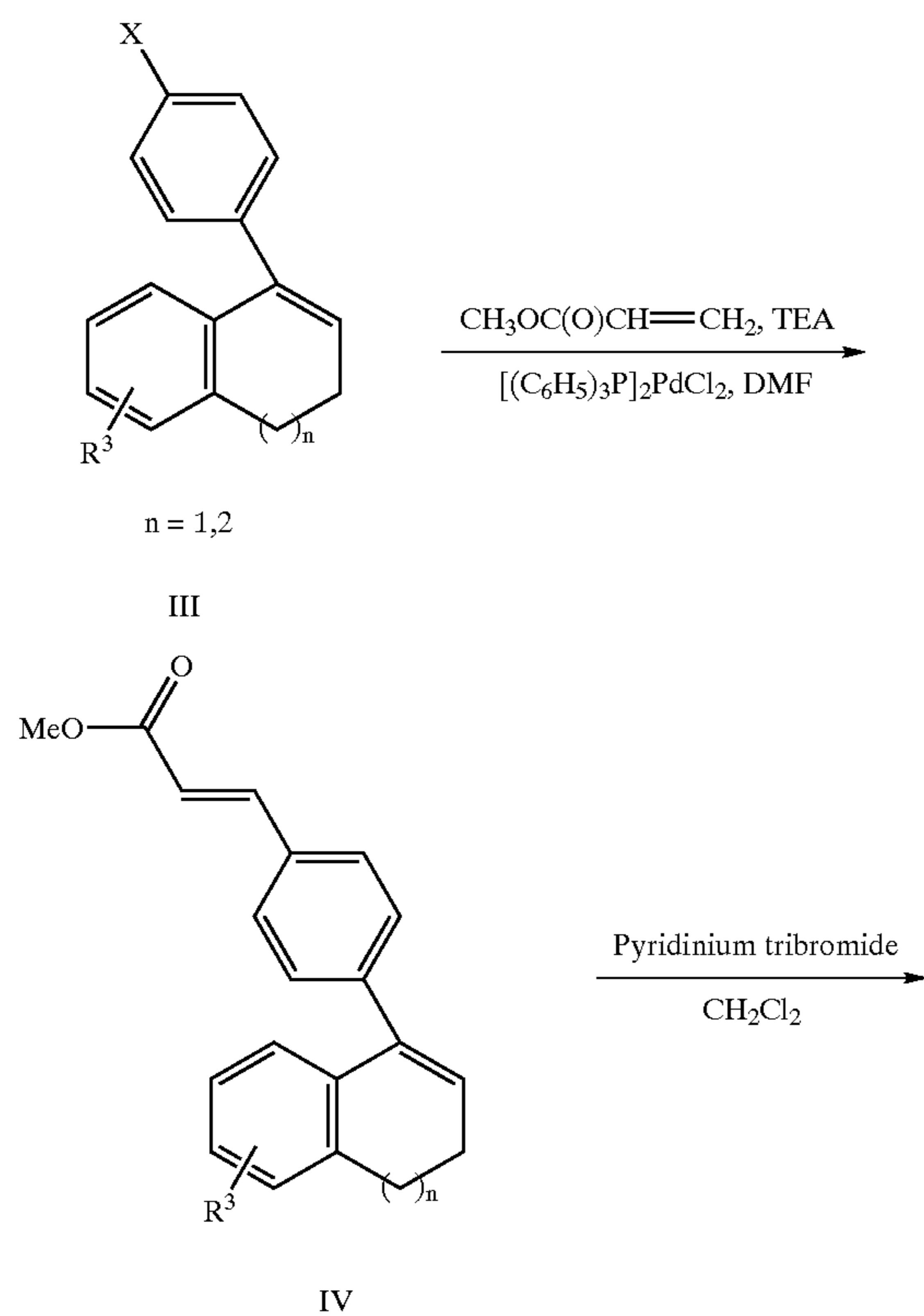
Scheme 2: General Synthesis of Acylsulfonamide VIII
