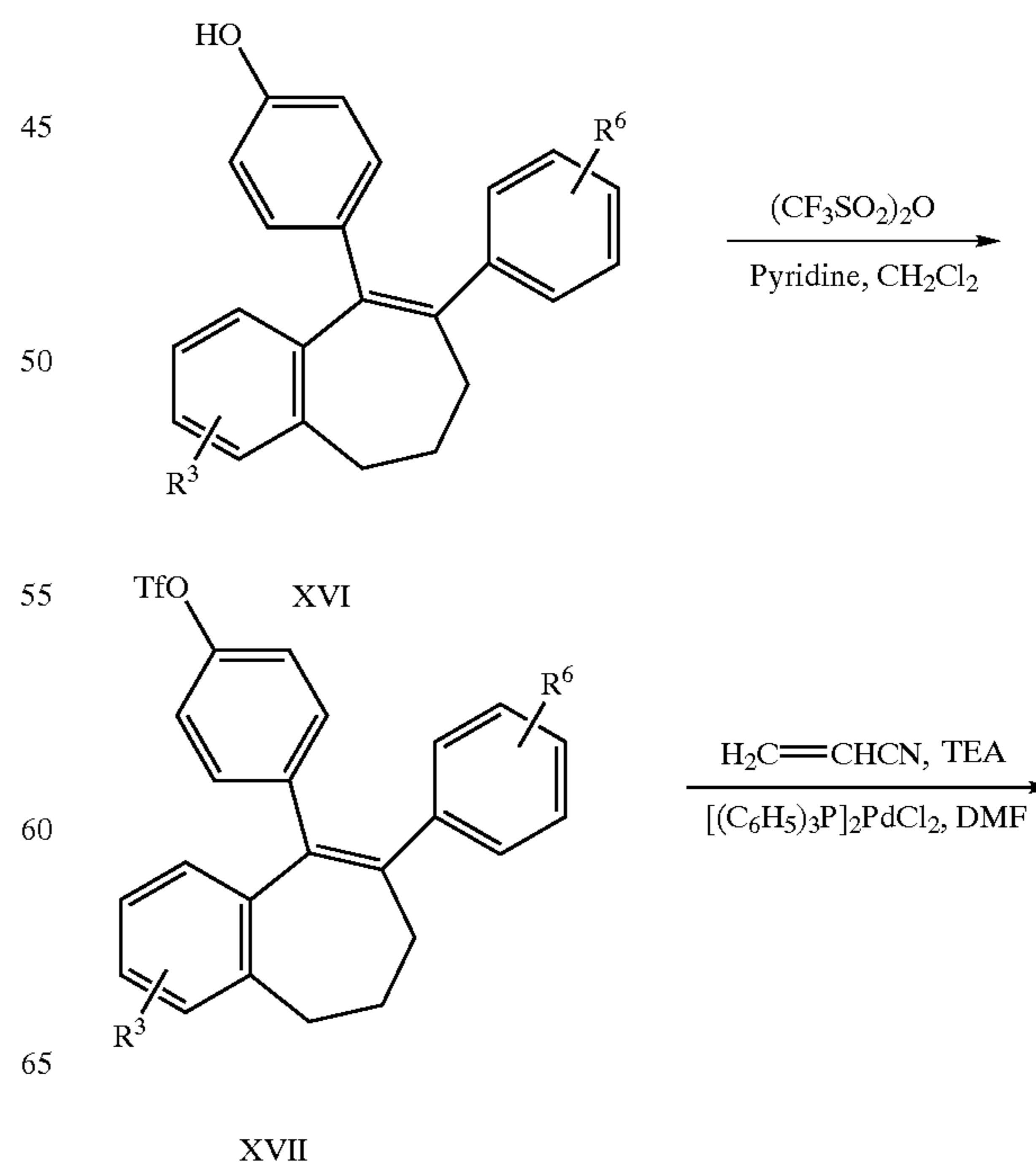
Scheme 5: Synthesis of dihydro benzocycloheptenyl tetrazole XIX
