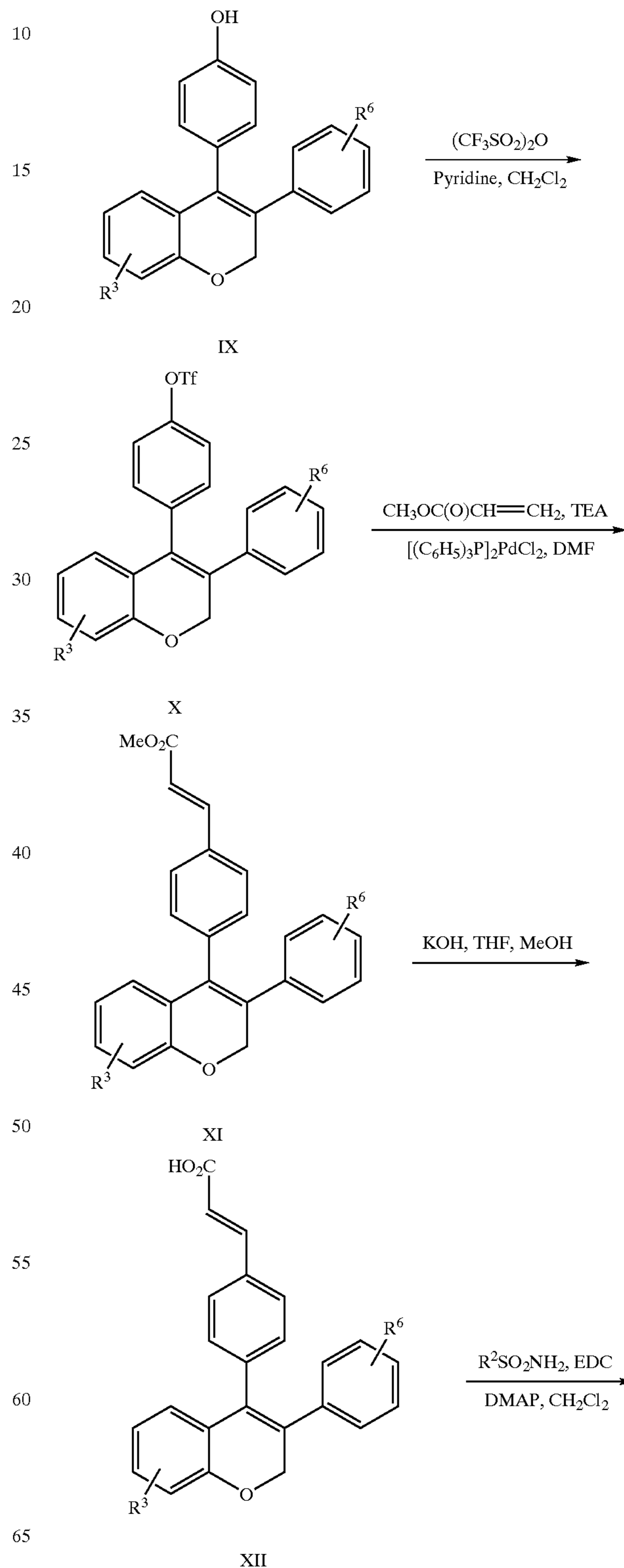
Scheme 3: General Synthesis of Benzopyran XIII
