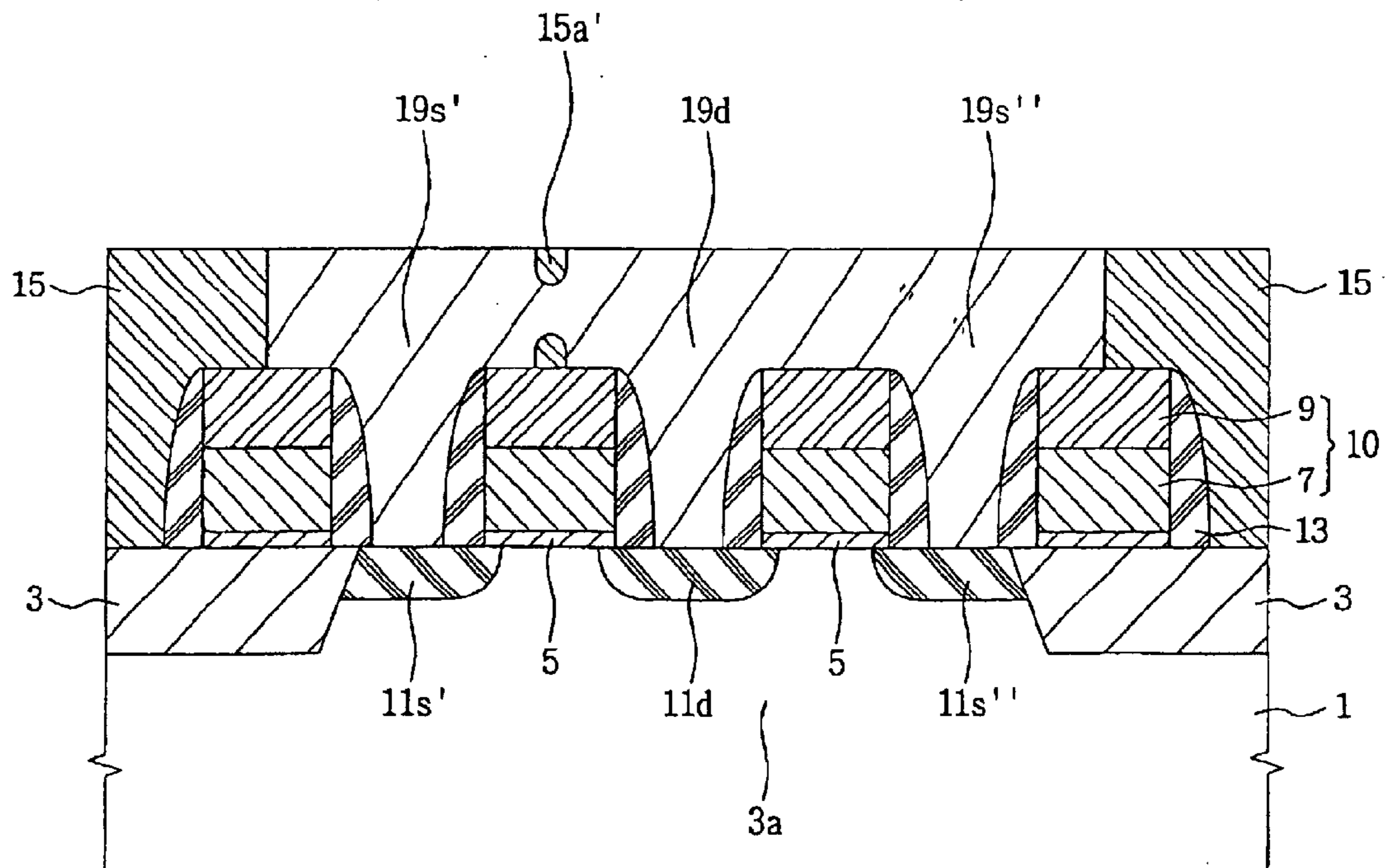
FIG. 4 (CONVENTIONAL ART)
