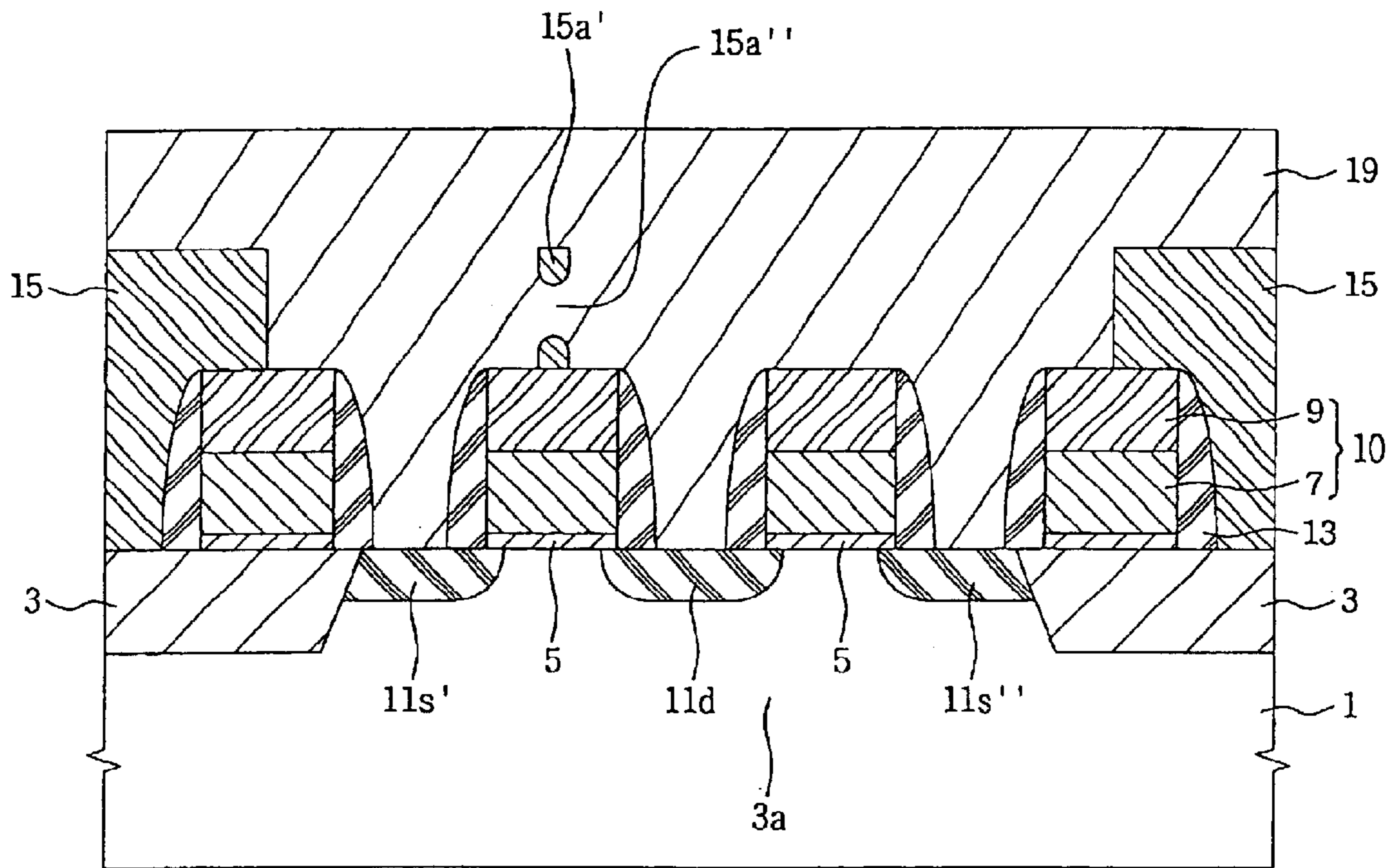
FIG. 3 (CONVENTIONAL ART)
