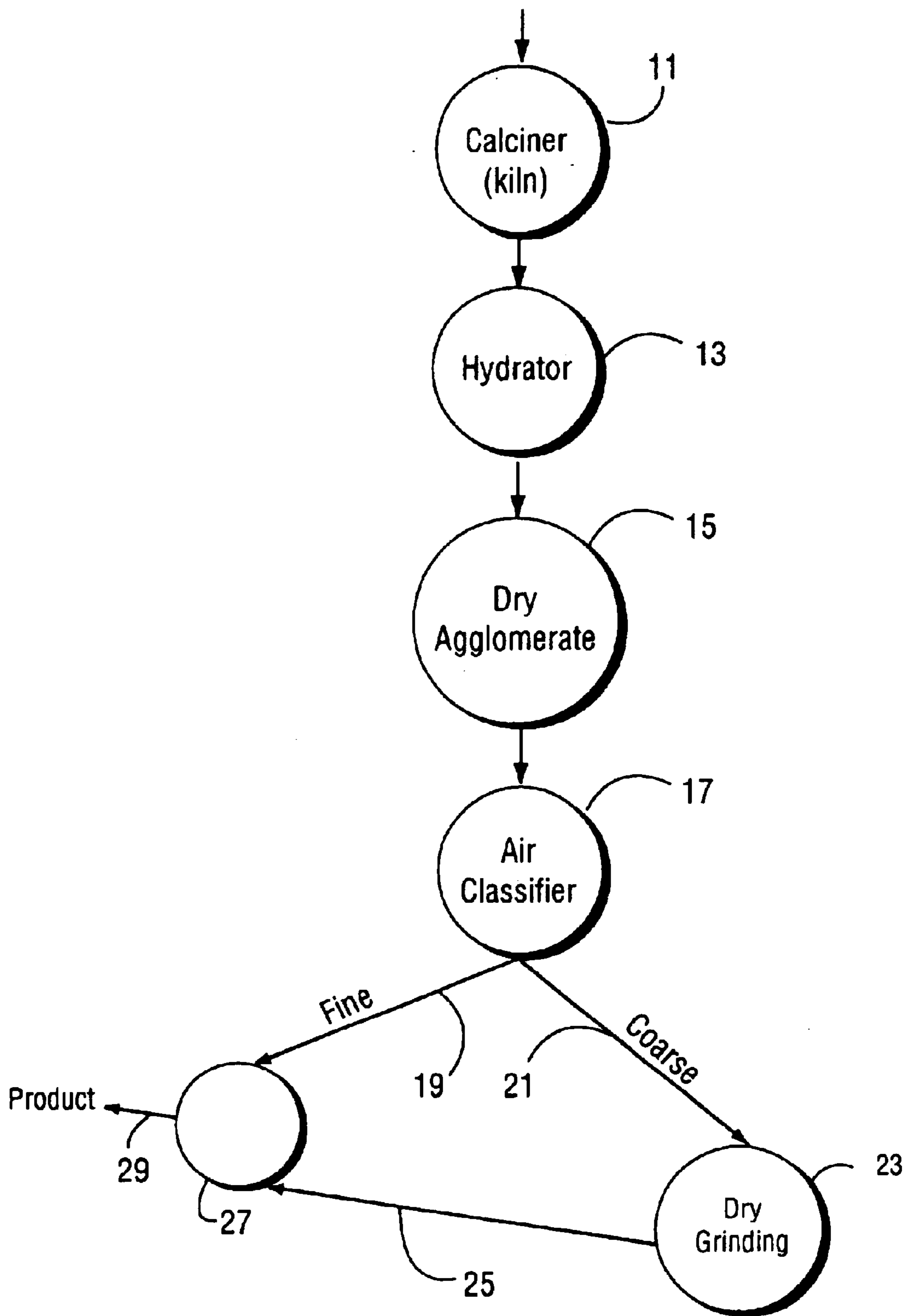
FIG. 1 (Prior Art)
