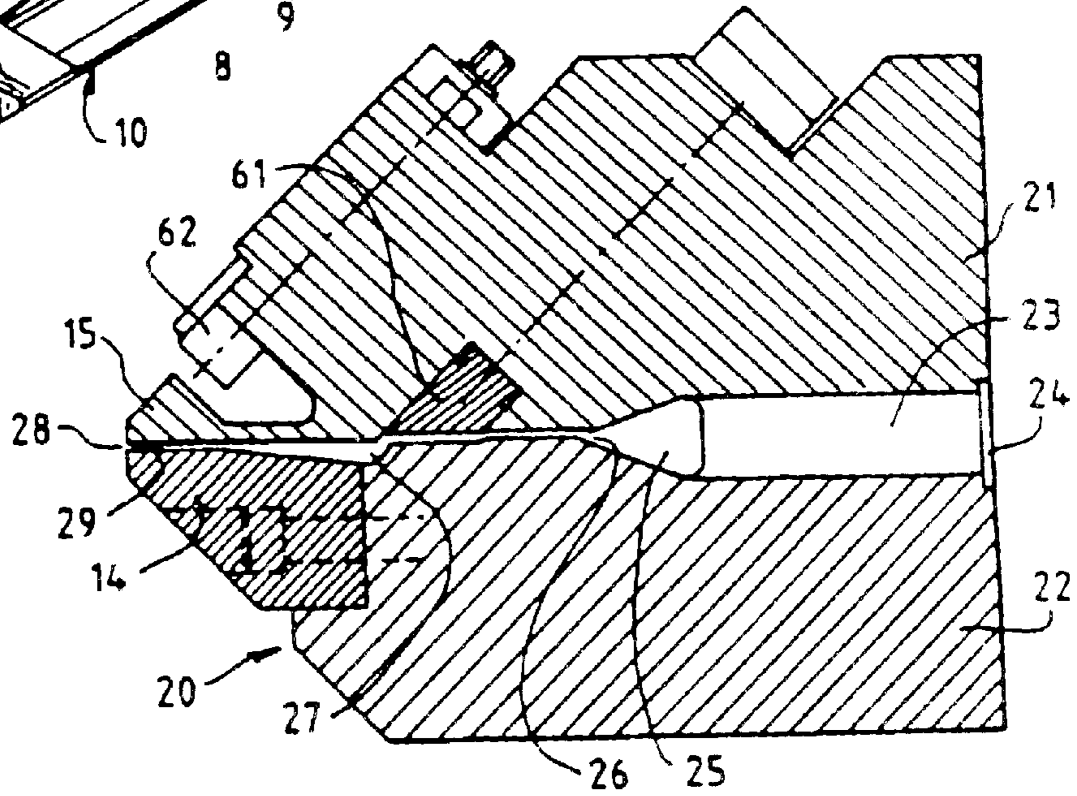
FIG. 2 PRIOR ART
