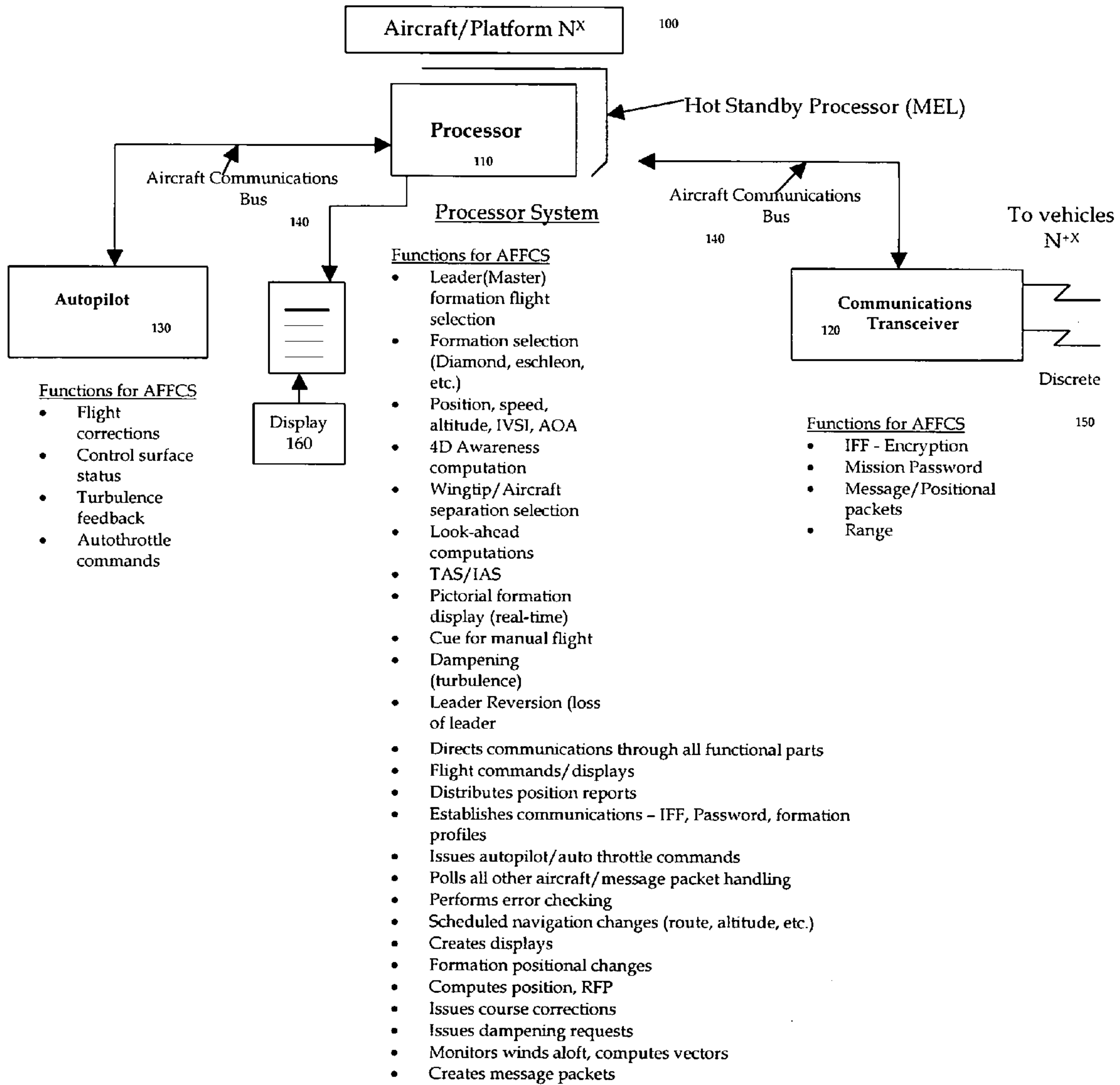
AFFCS Functional Block Diagram - Figure 1
