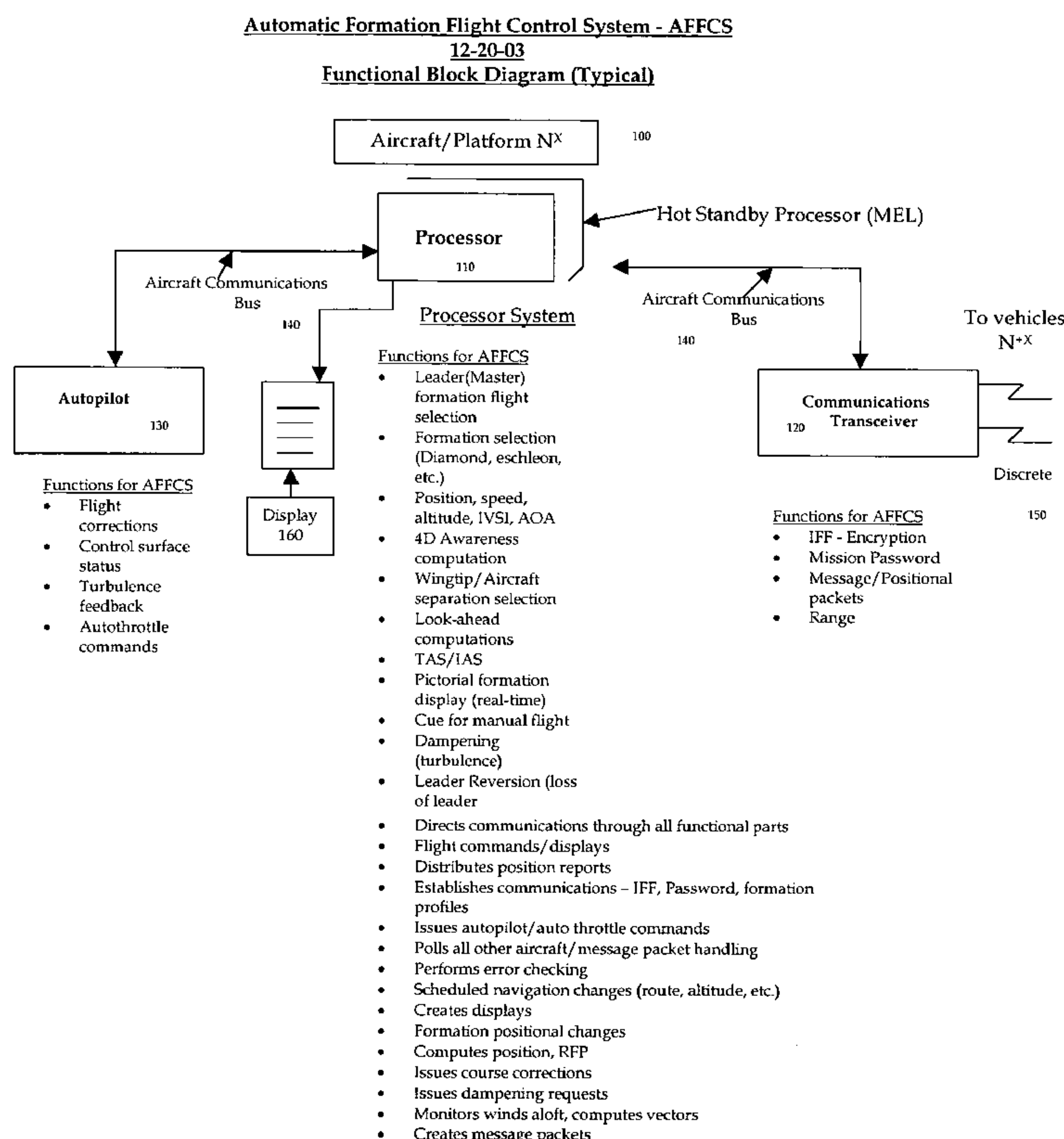
AFFCS Functional Block Diagram
