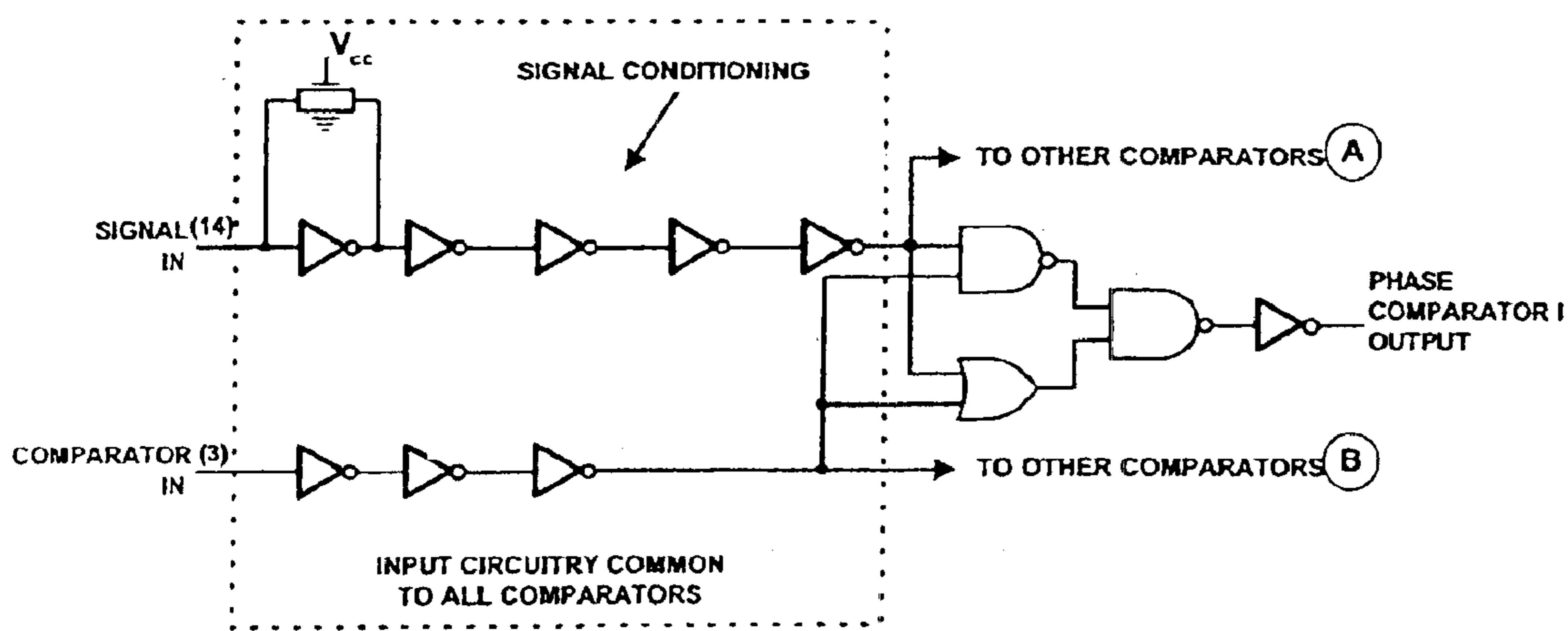
(B) DETAILED ON-CHIP IC CIRCUITRY IN 74HC4046
