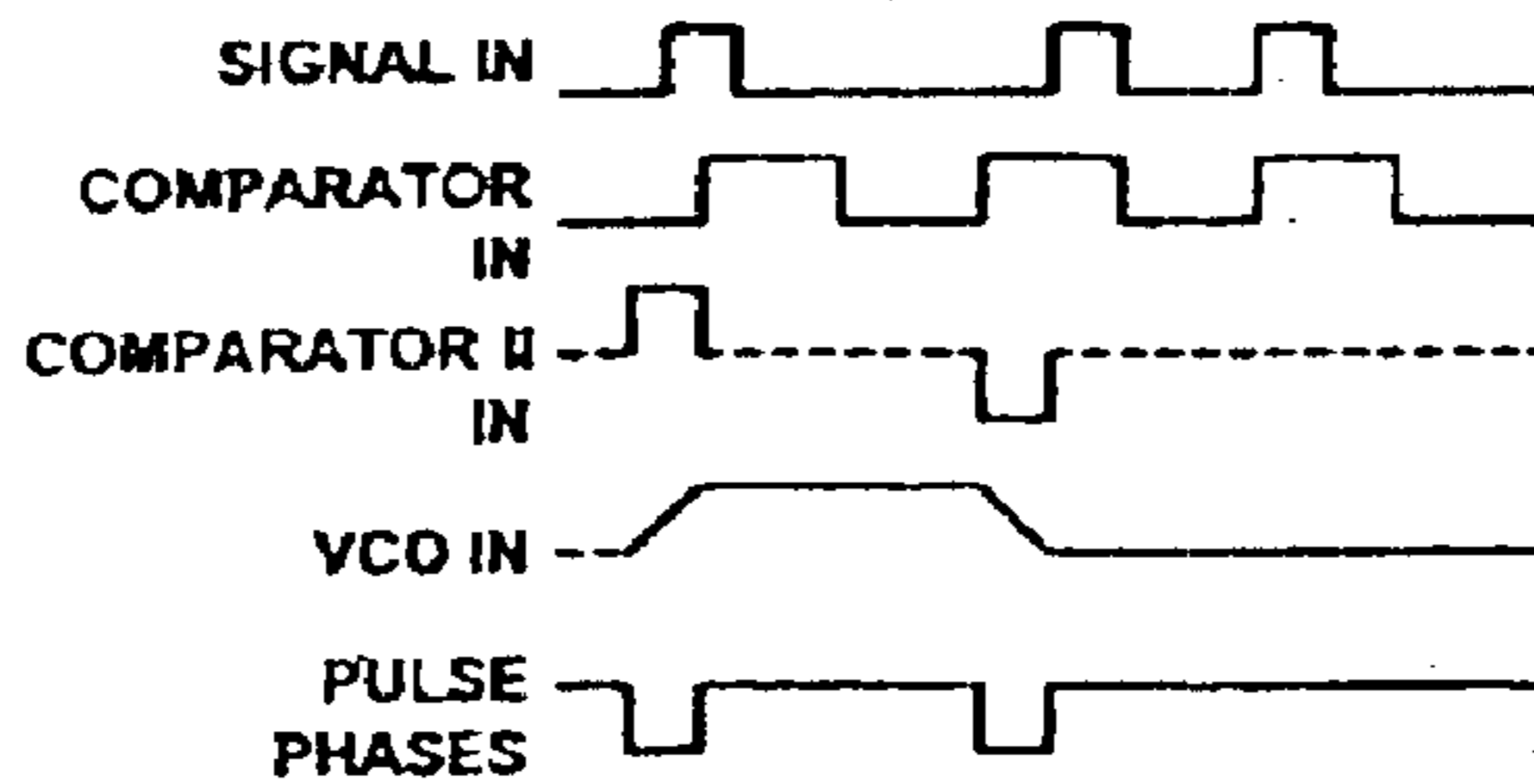
TIMING AND WAVEFORMS OF PFD (existing art)
