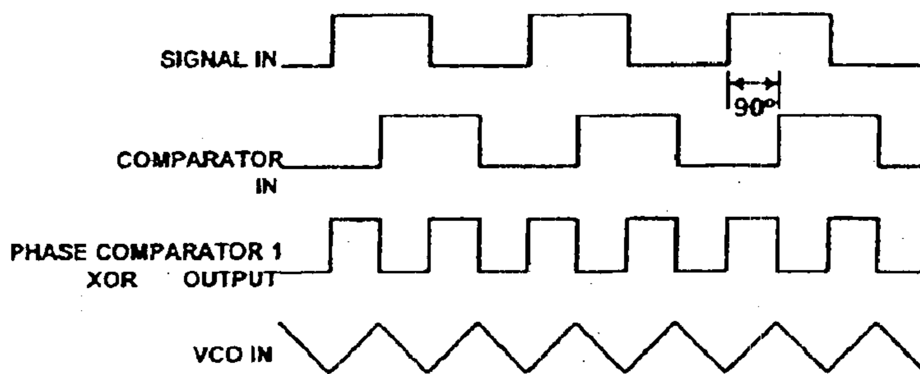
(C) TYPICAL XOR DETECTOR WAVEFORMS
