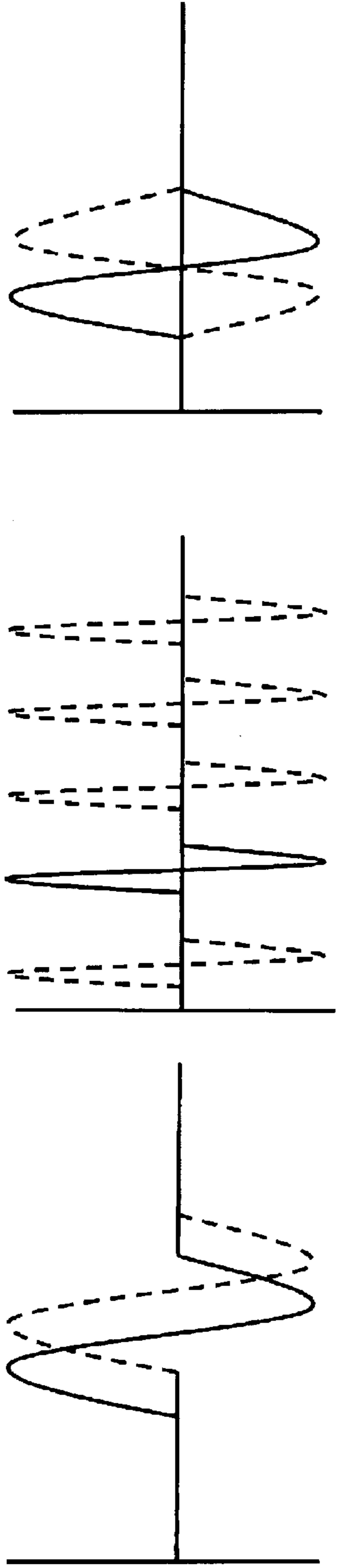
Early - Late Modulation FIG. 4A One of Many Modulation FIG. 4B Flip Modulation FIG. 4C
