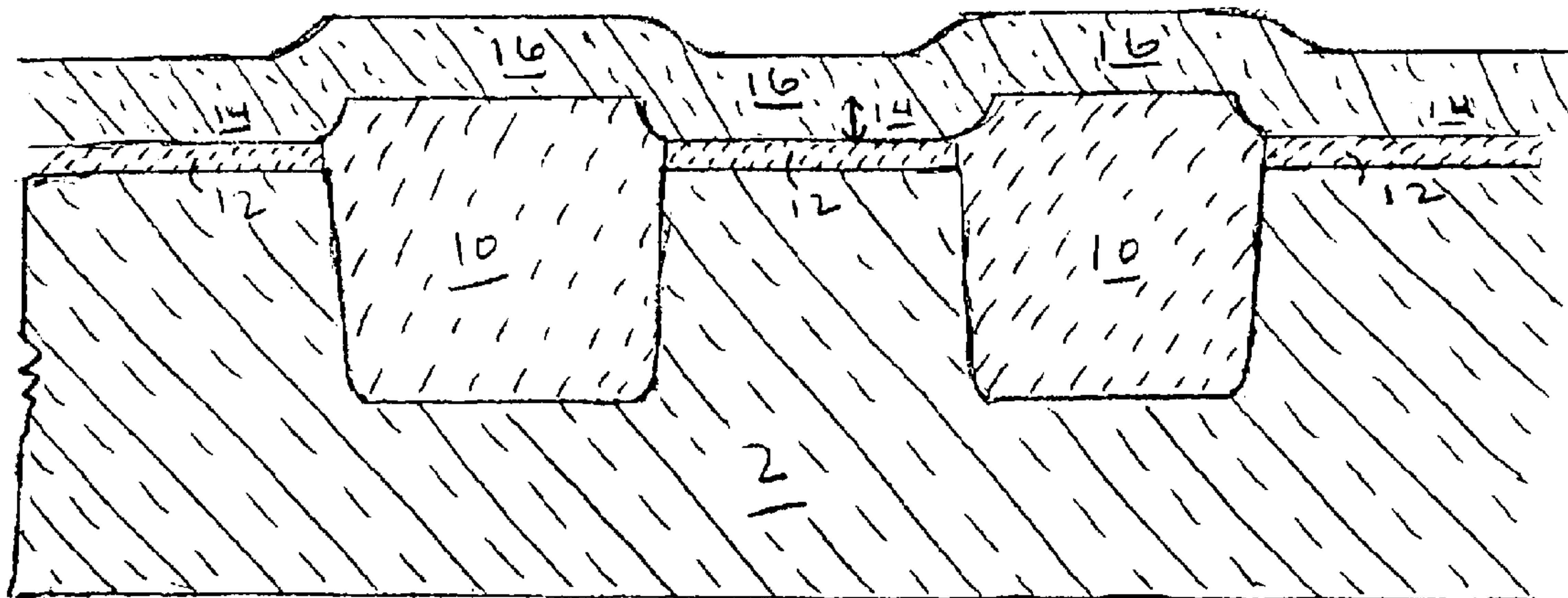
FIG. 1c PRIOR ART
