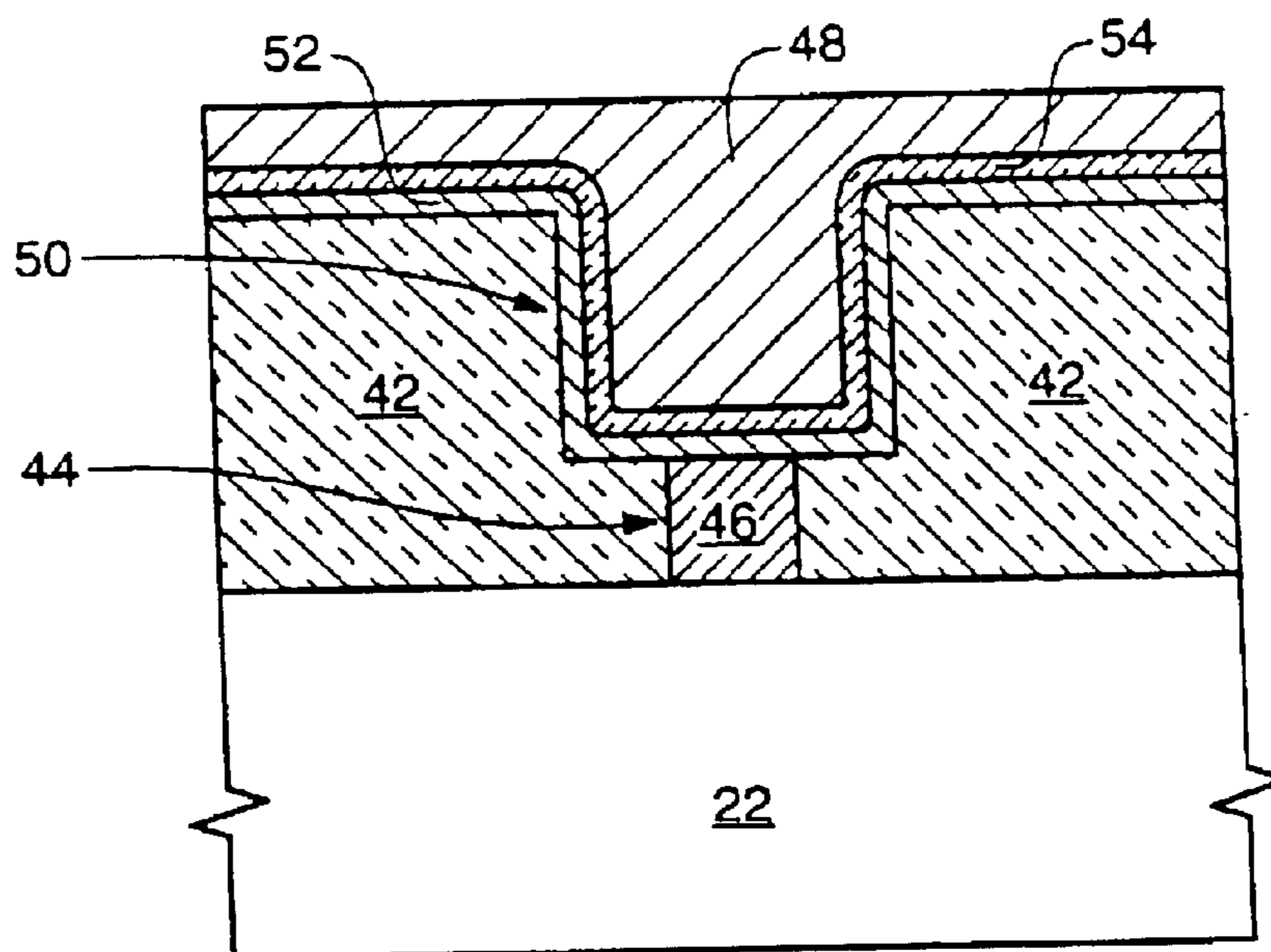
FIG. 8 (PRIOR ART)
