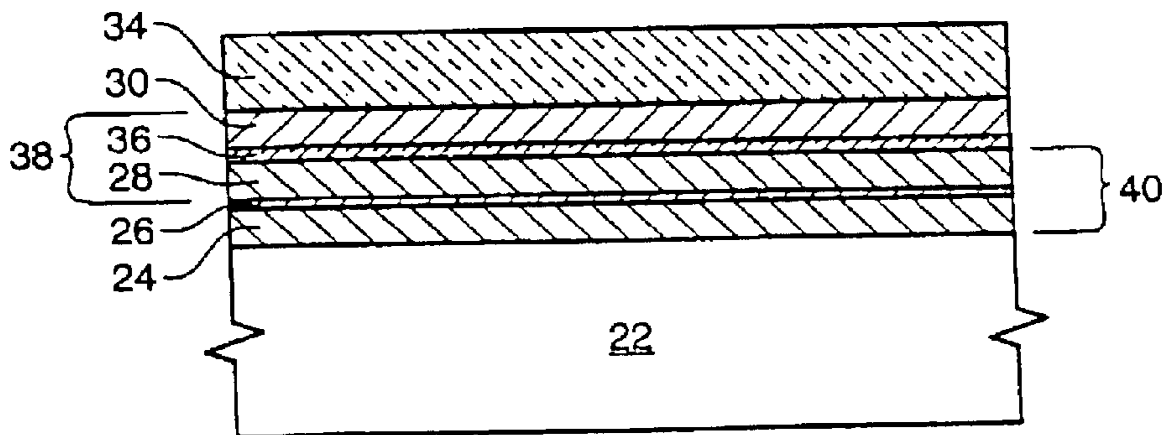
FIG. 3 (PRIOR ART)
