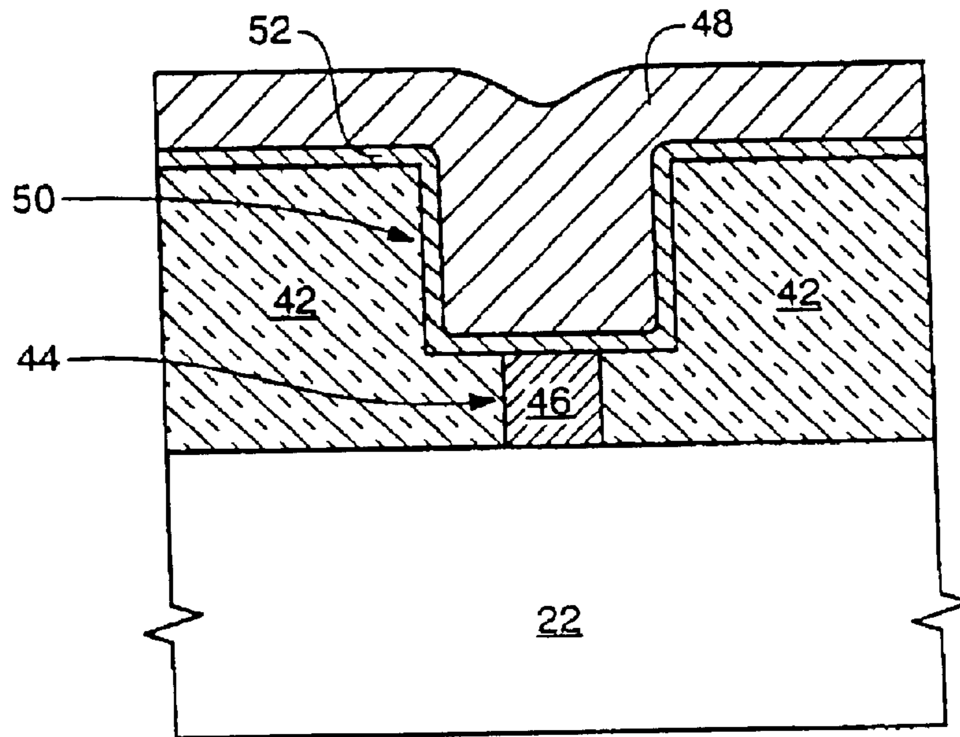
FIG. 7 (PRIOR ART)
