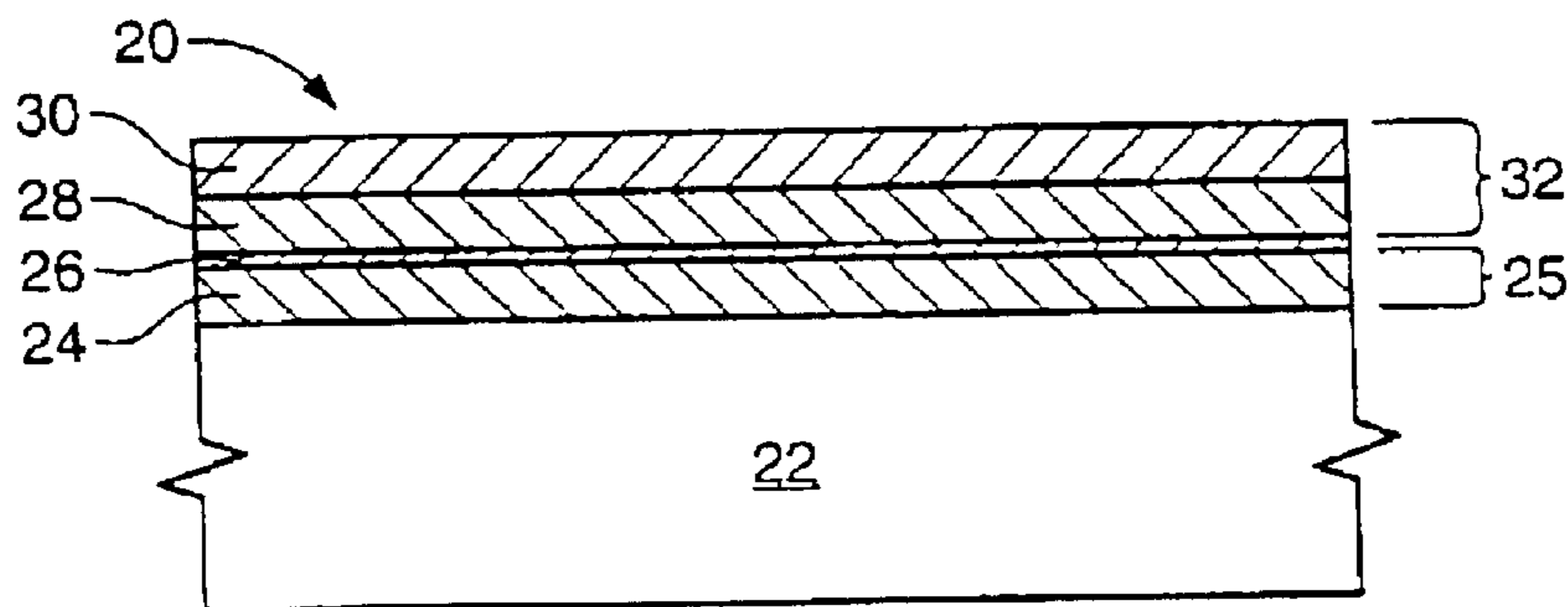
FIG. 2 (PRIOR ART)
